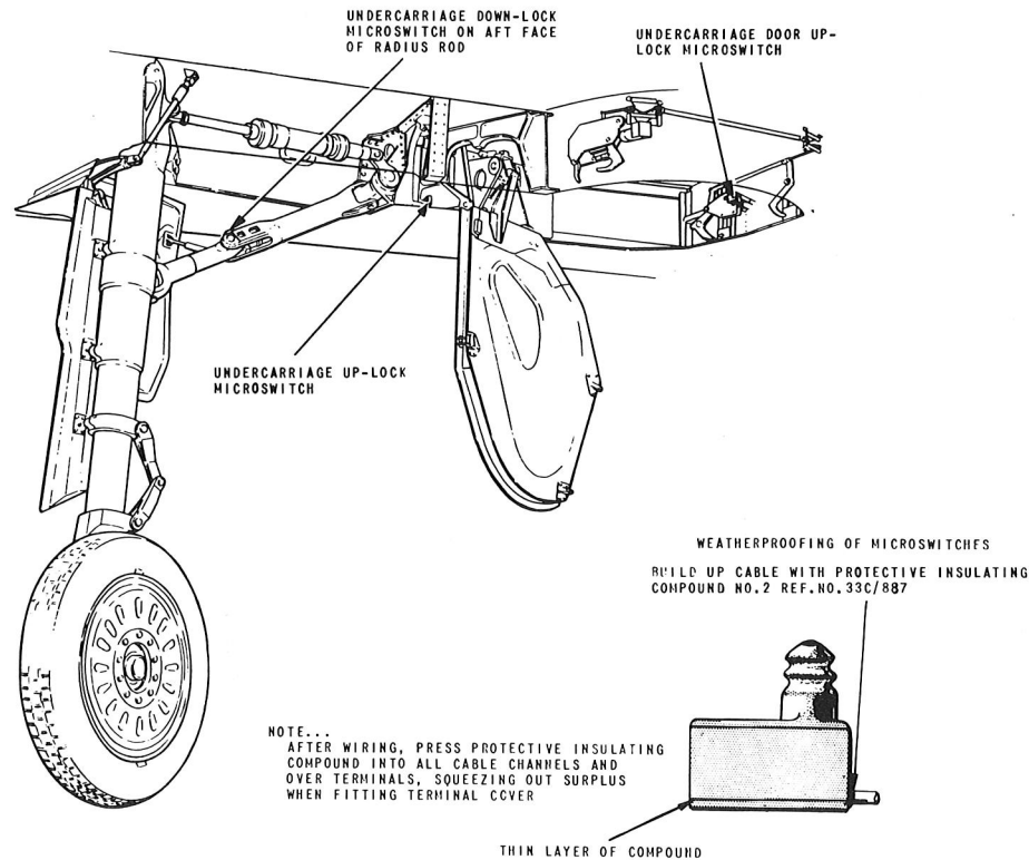
Fig. 2. Alighting gear details
