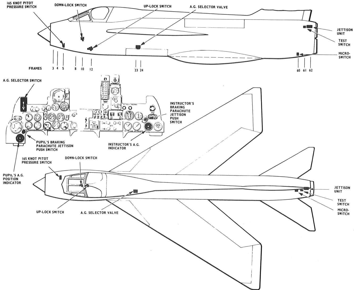
FIG.1. ALIGHTING GEAR AND BRAKING PARACHUTE JETTISON
