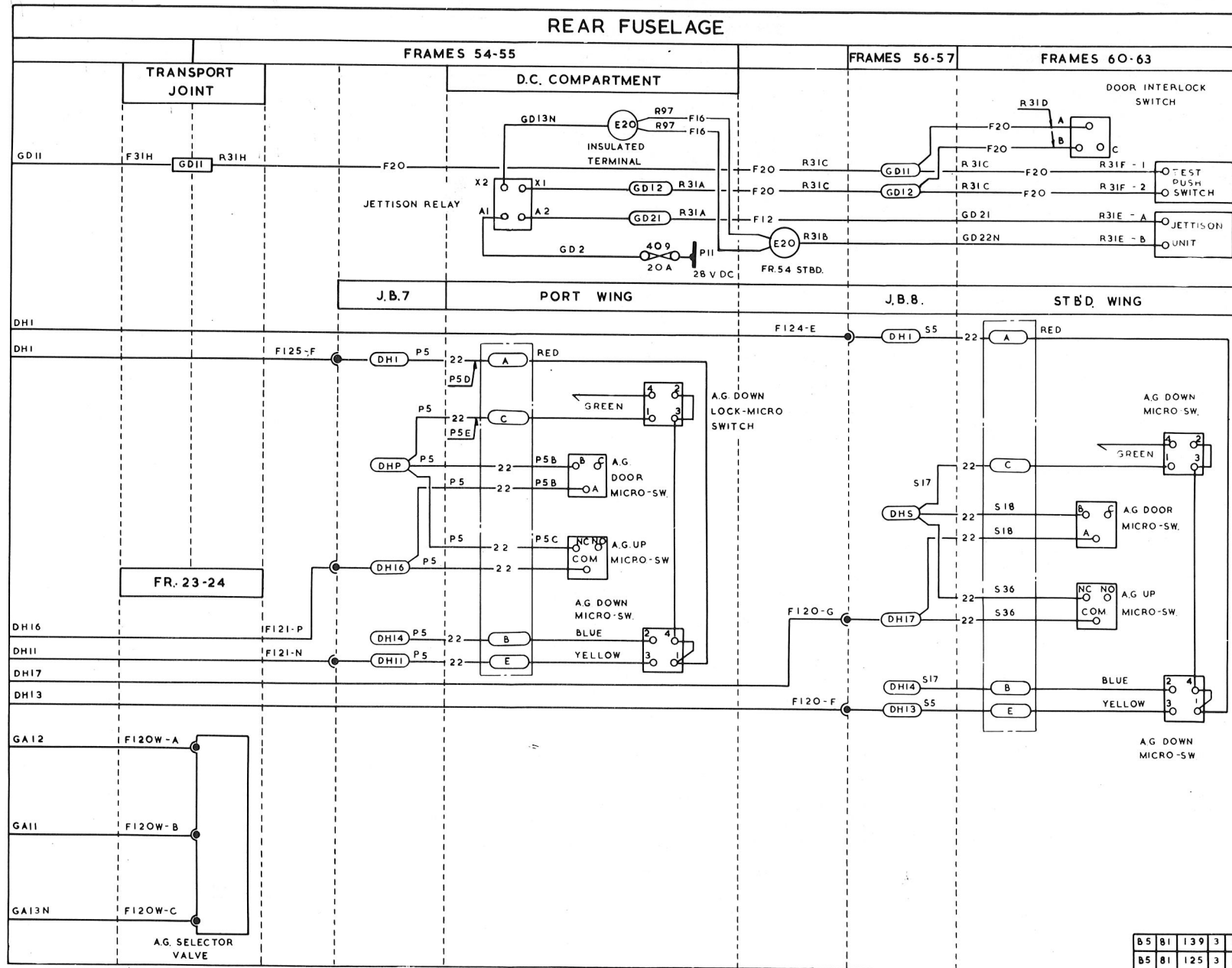
FIG. 4A. ALIGHTING GEAR AND BRAKING PARACHUTE JETTISON
