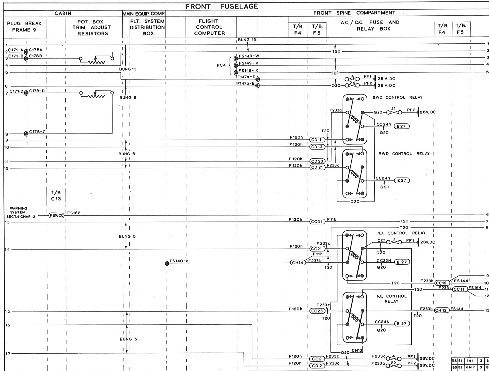
FIG.7A. FLIGHT CONTROL SYSTEM (STRIIP 3)
