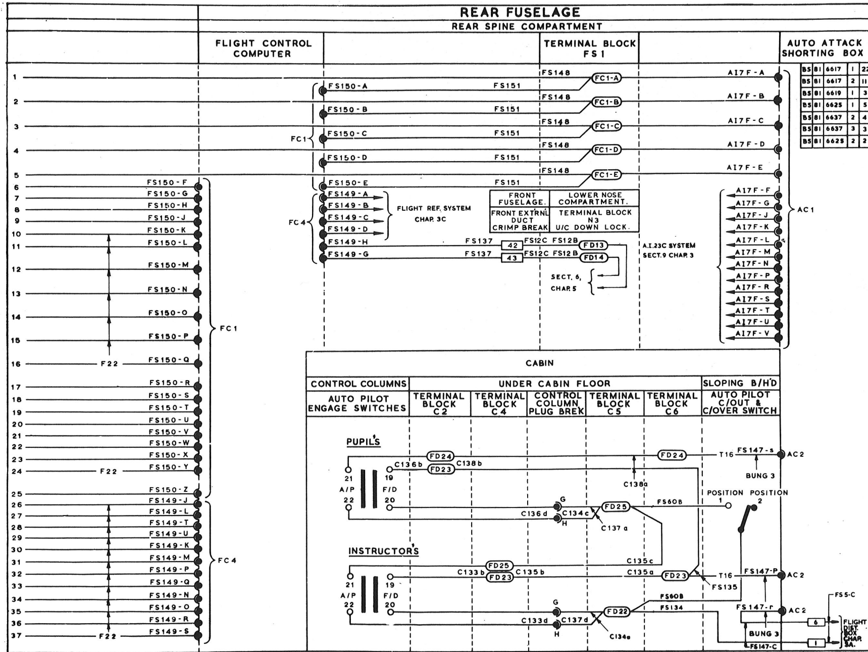
FIG.5 A. FLIGHT CONTROL SYSTEM
