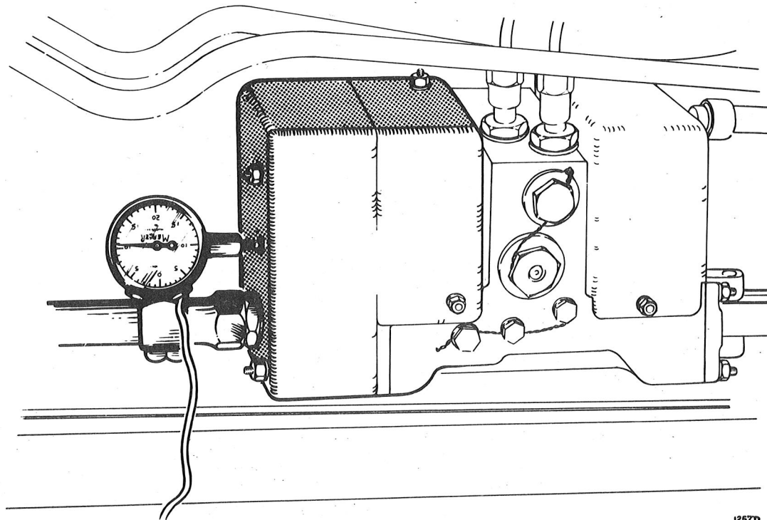
Fig. 3. Dither adjustment rig - ailerons
