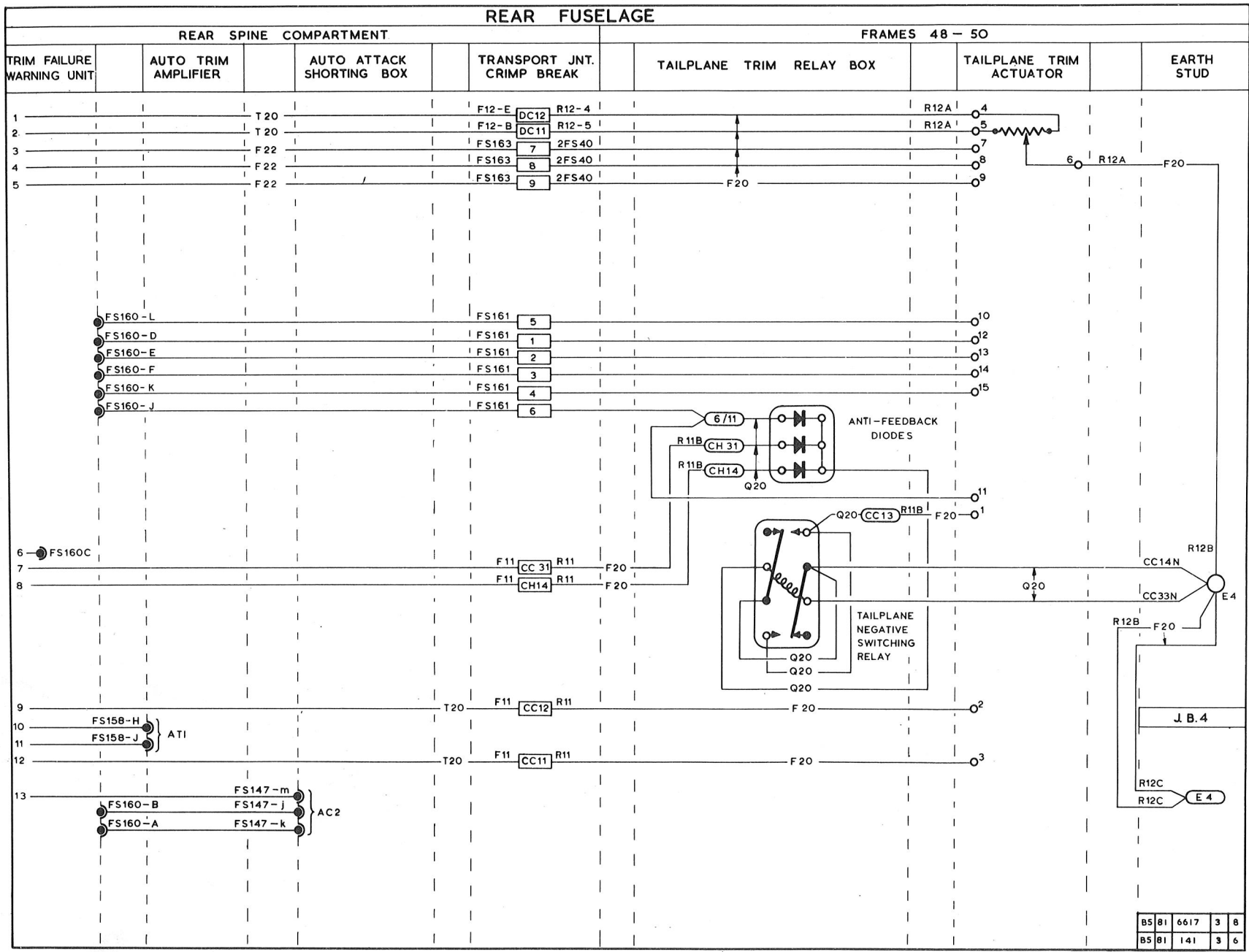
FIG.7B. FLIGHT CONTROL SYSTEM (STRIP 3)
