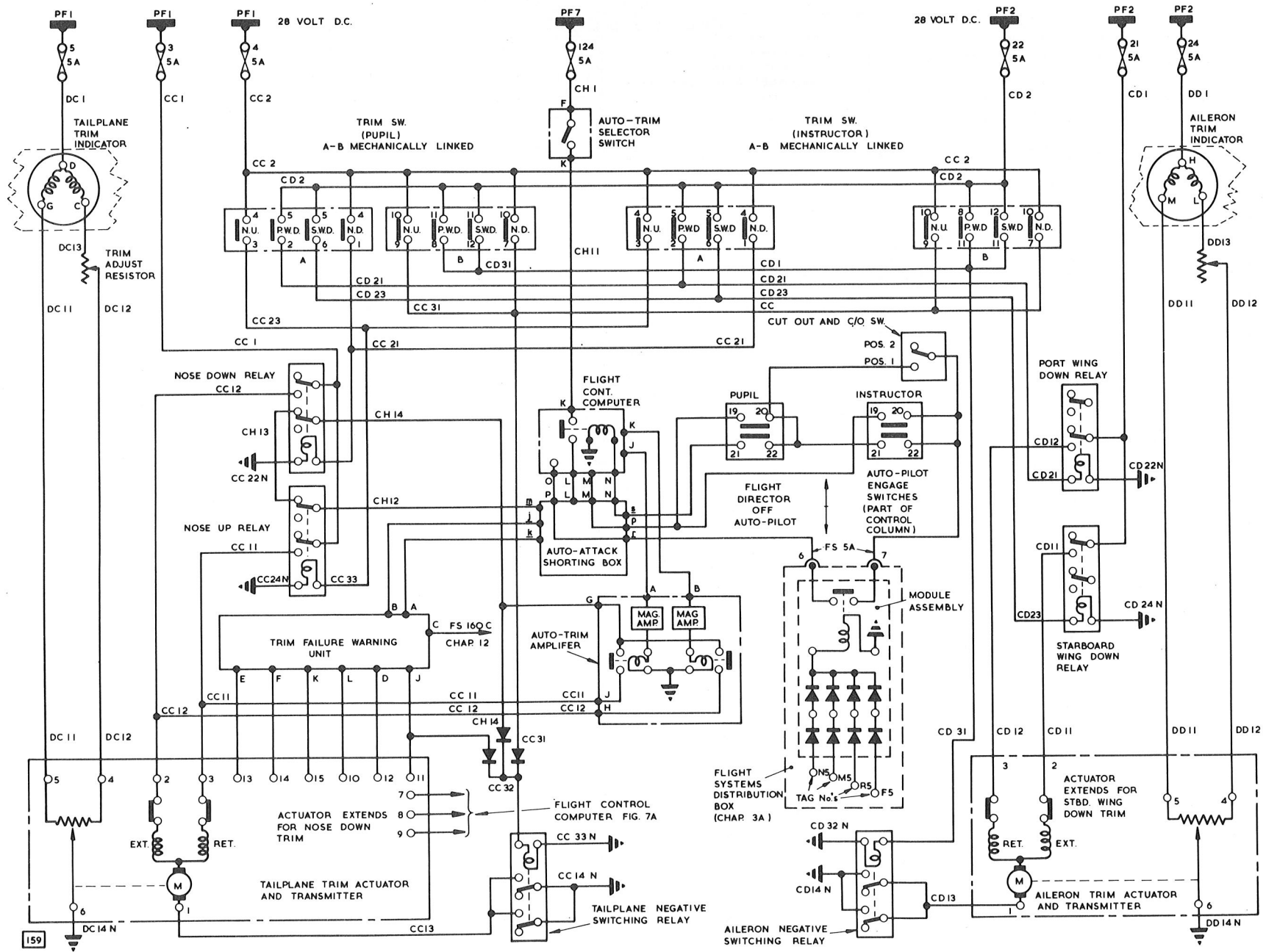
FIG.4. TAIL PLANE AND AILERON TRIM CONTROL
