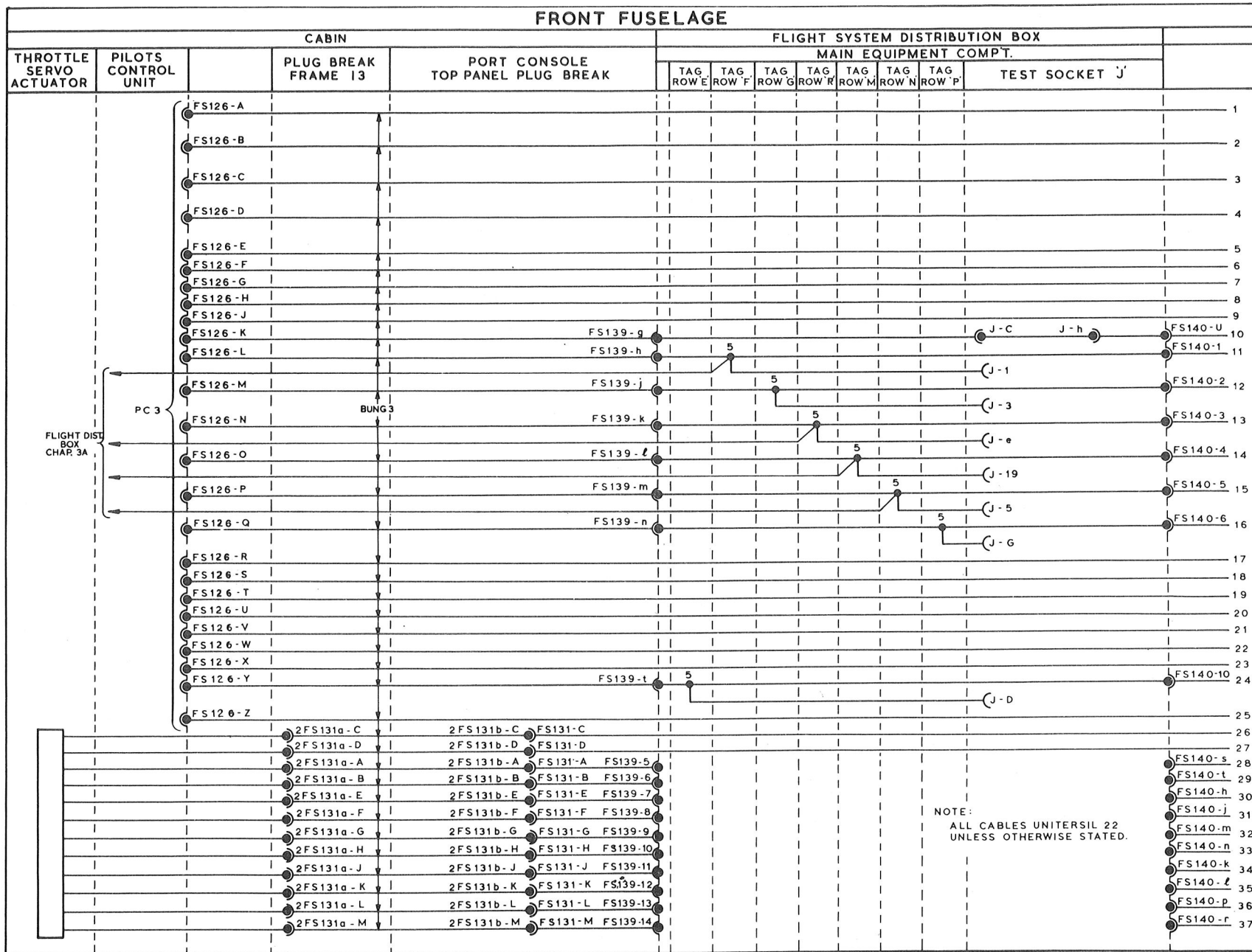
FIG.5. FLIGHT CONTROL SYSTEM (STRIP I)
