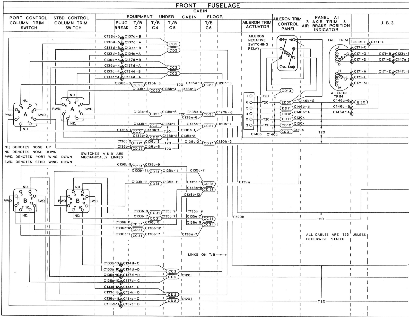
FIG.7. FLIGHT CONTROL SYSTEM (STRIP 3)
