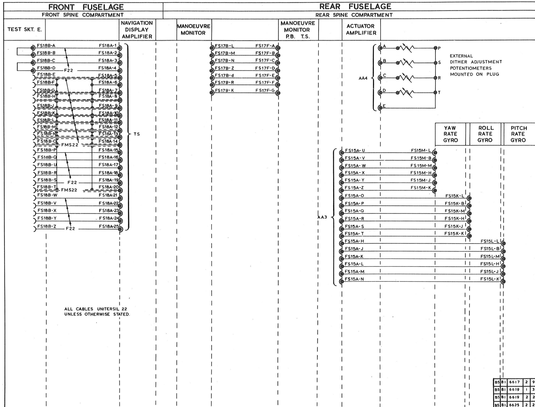
FIG.10. FLIGHT CONTROL SYSTEM (STRIP 6)
