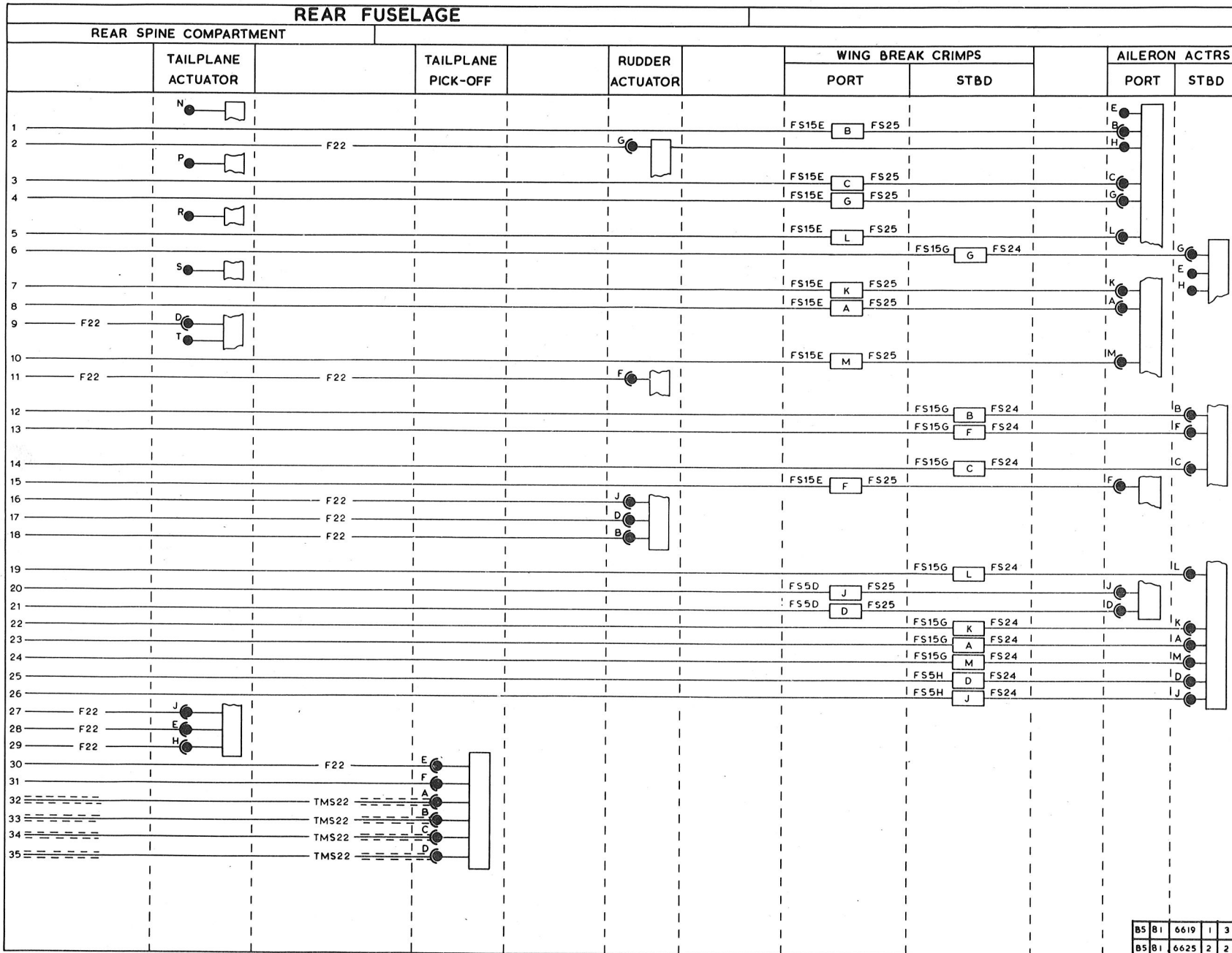
FIG.9B. FLIGHT CONTROL SYSTEM (STRIP 5)
