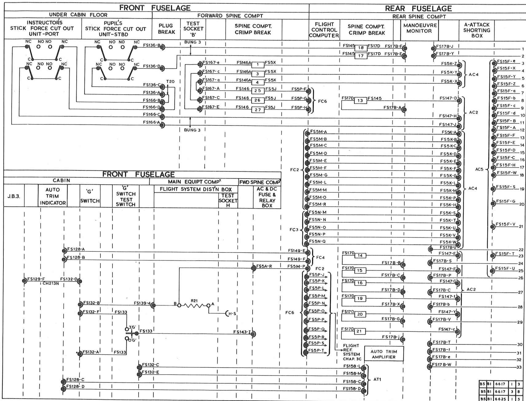
FIG.8. FLIGHT CONTROL SYSTEM
