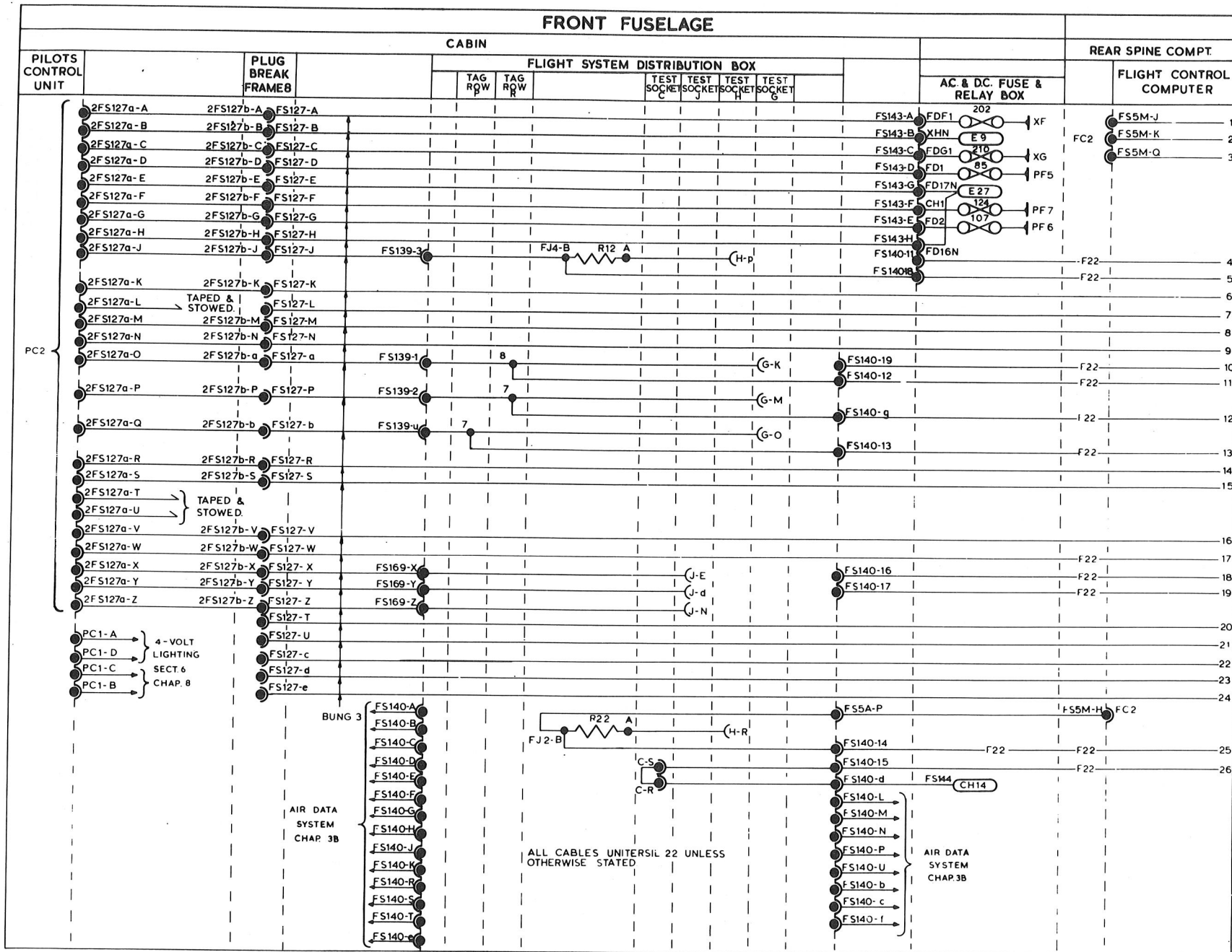
FIG.6. FLIGHT CONTROL SYSTEM (STRIP 2)
