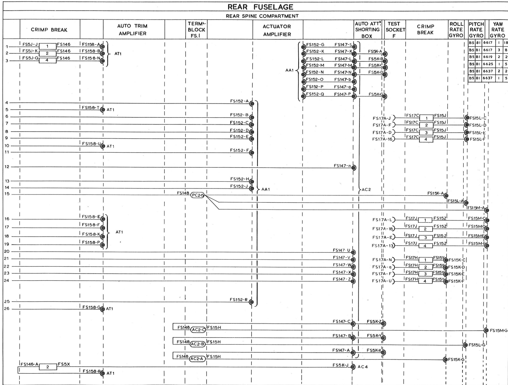
FIG.6A. FLIGHT CONTROL SYSTEM (STRIP 2)
