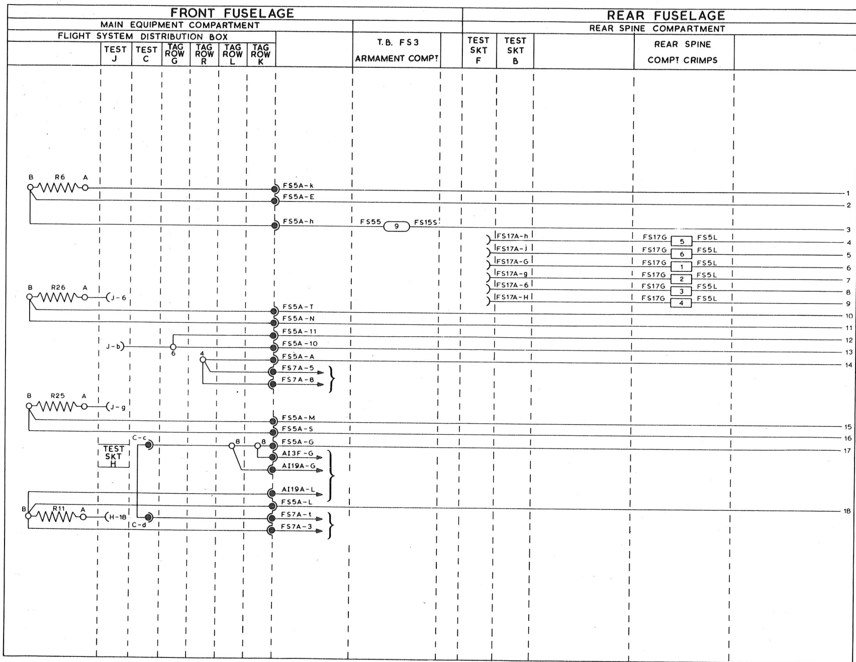
FIG.9. FLIGHT CONTROL SYSTEM (STRIP 5)
