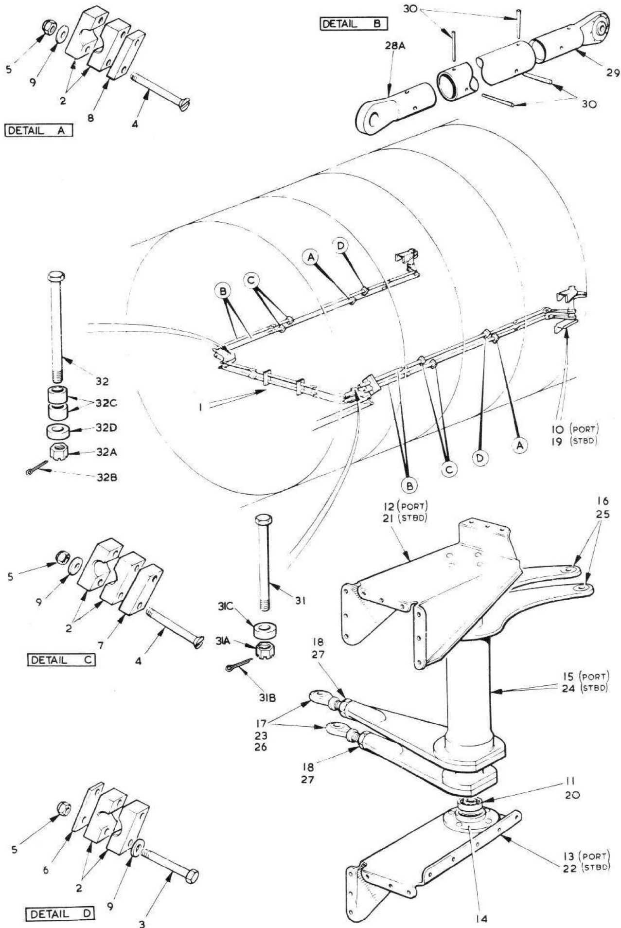
FIG. 1 ENGINE CONTROLS IN CENTRE FUSELAGE
