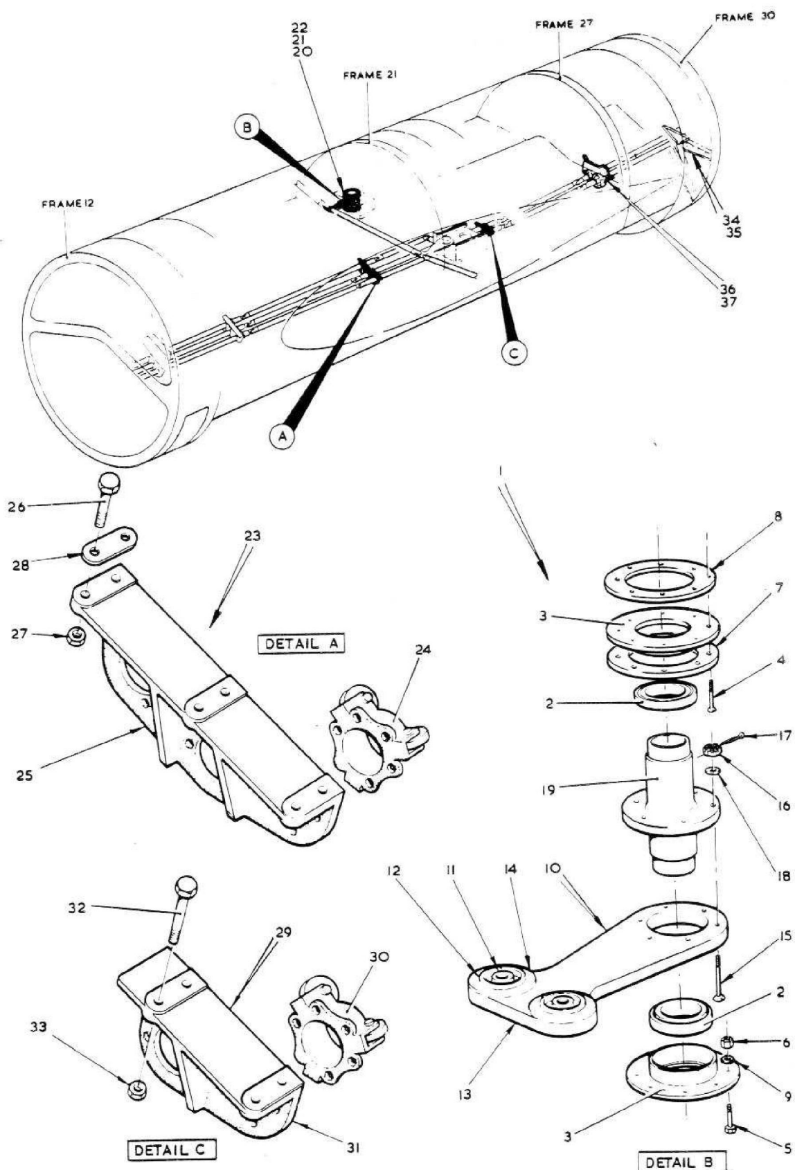
FIG2 FLYING CONTROLS IN CENTRE FUSELAGE
