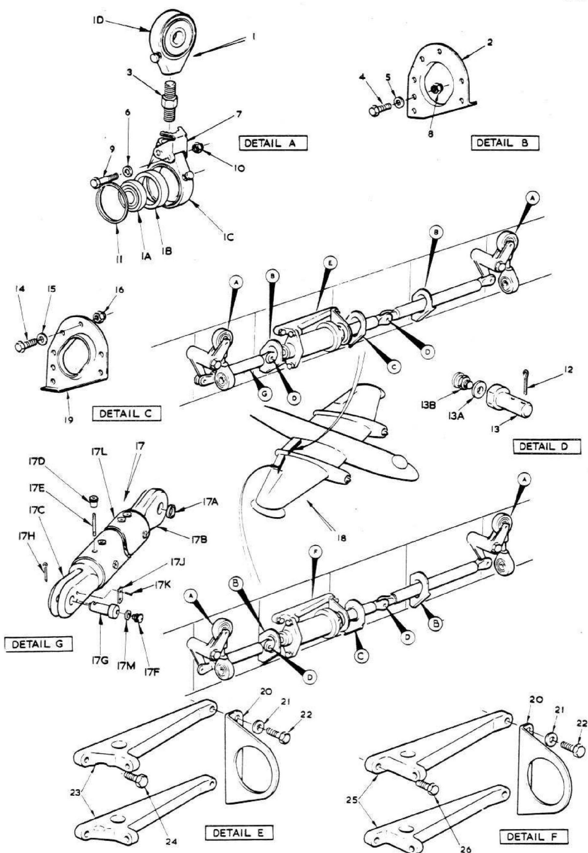
FIG.1 FLAP OPERATING MECHANISM, STBD
