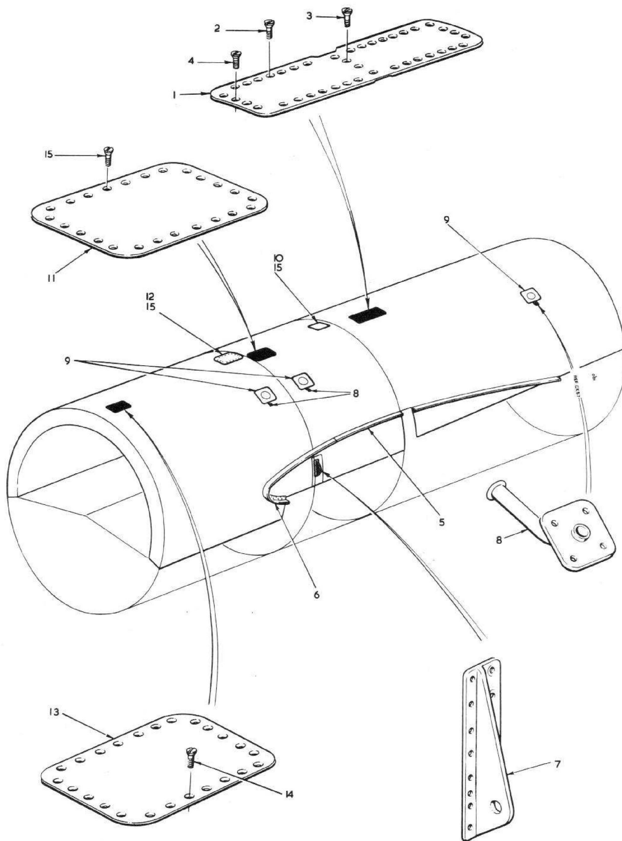
FIG.8 CENTRE FUSELAGE STRUCTURE
