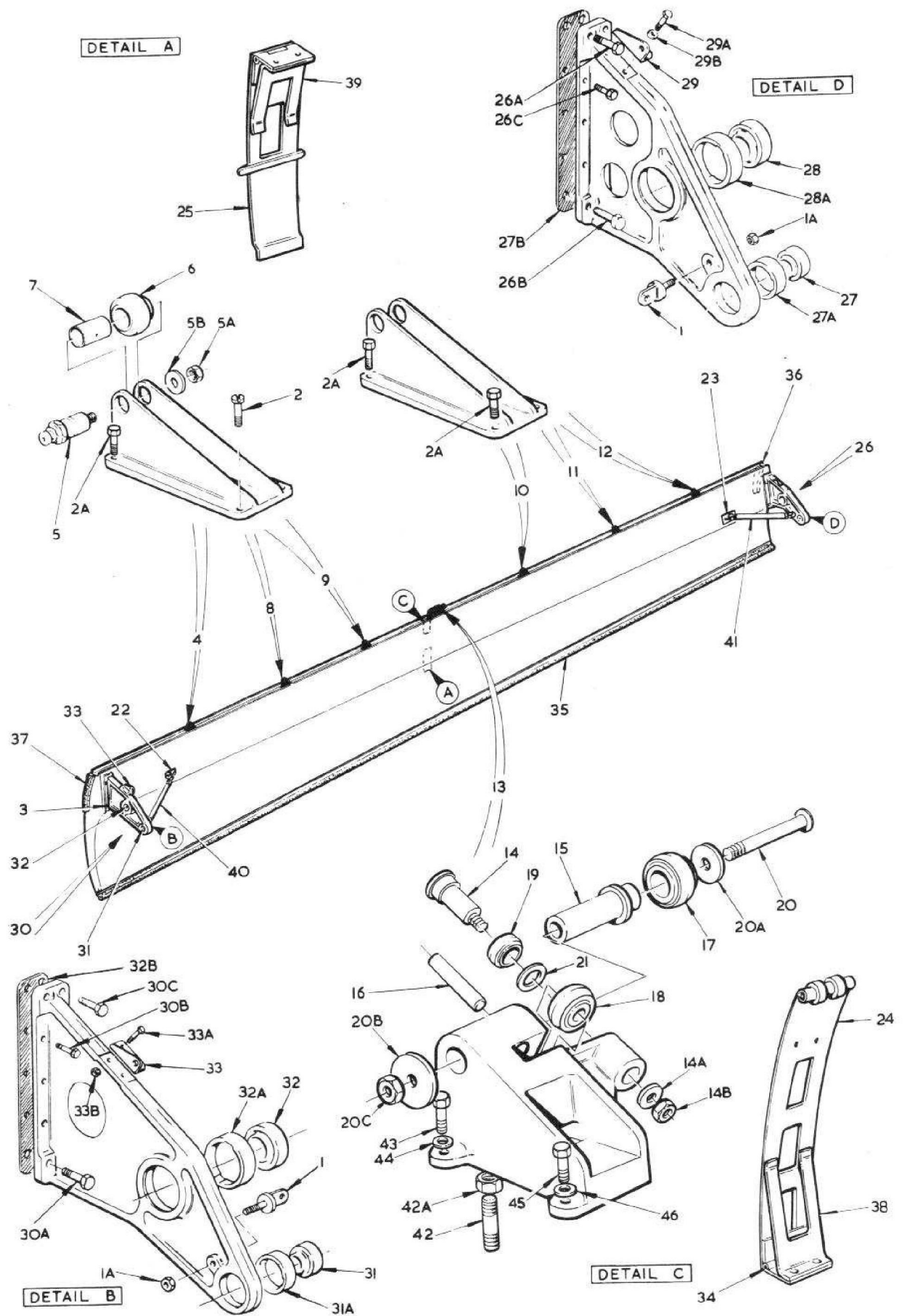
FIG.5 CENTRE FUSELAGE
