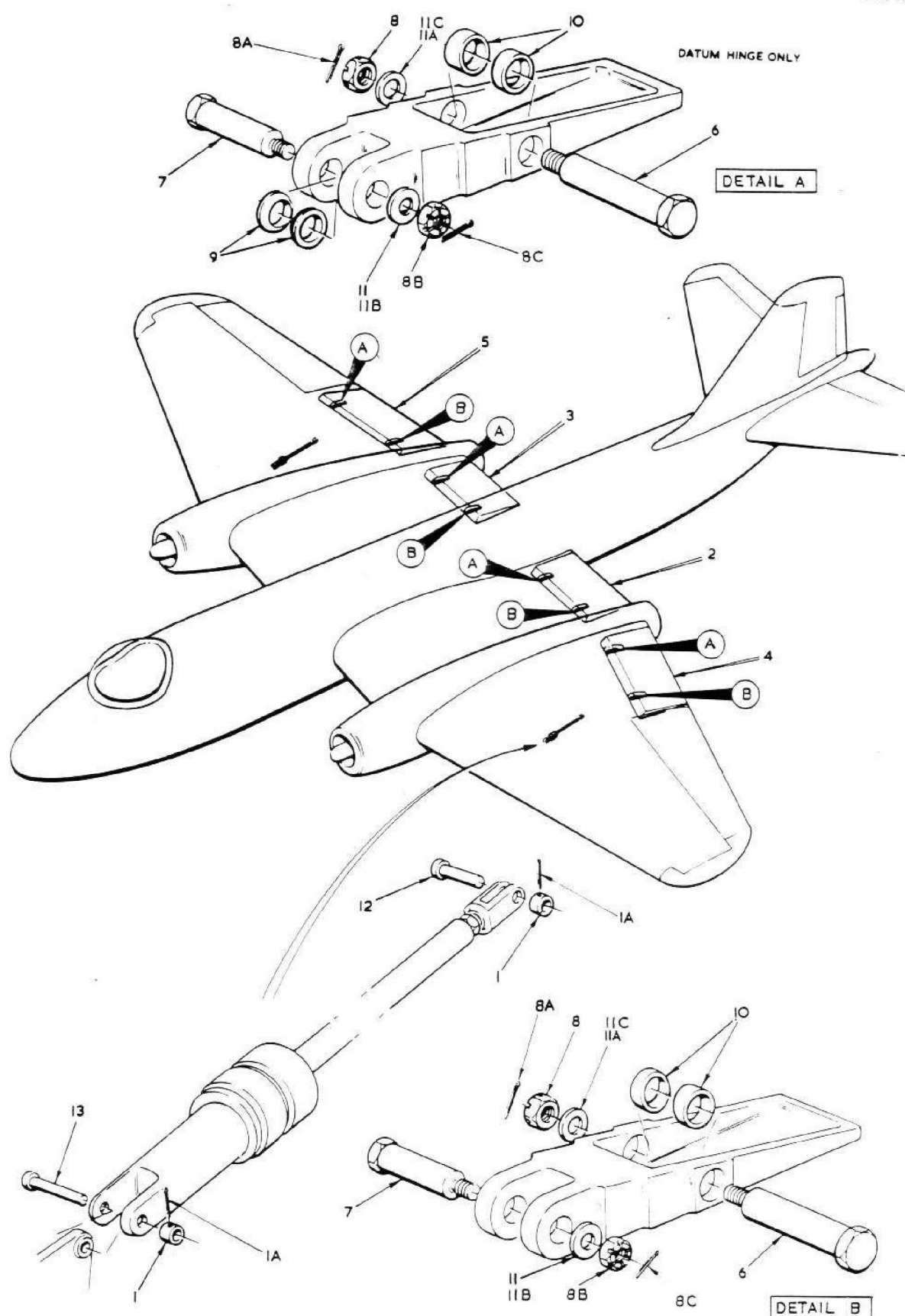
FIG 3 MAINPLANE AND FLAPS
