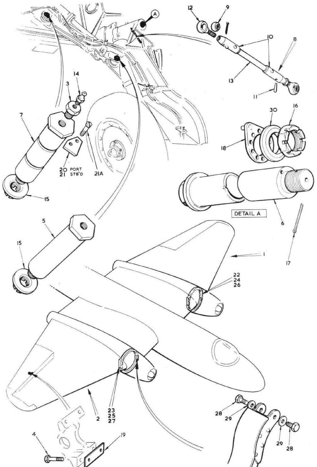
FIG.1 MAINPLANE AND FLAPS
