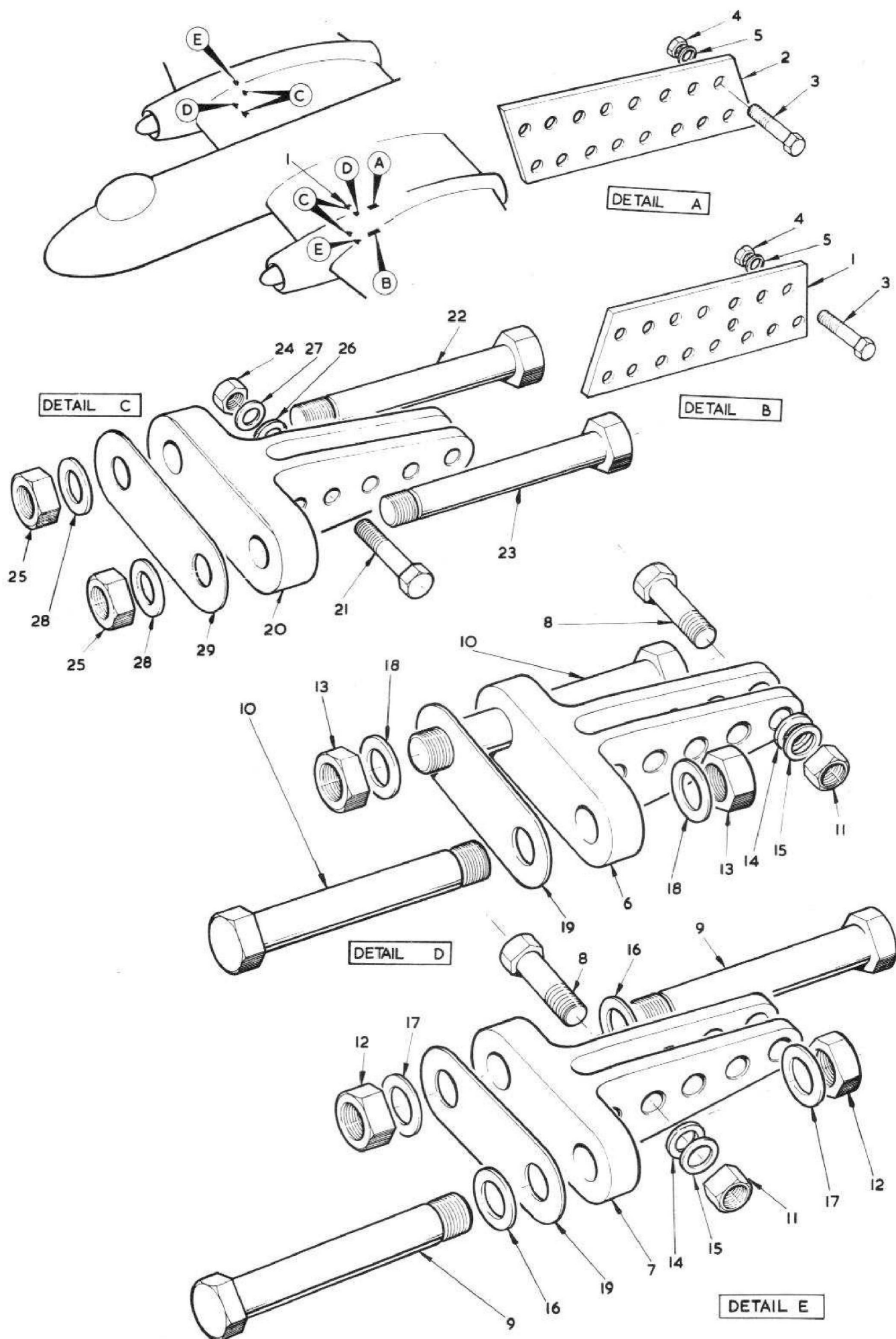
FIG.10 WING STRUCTURE
