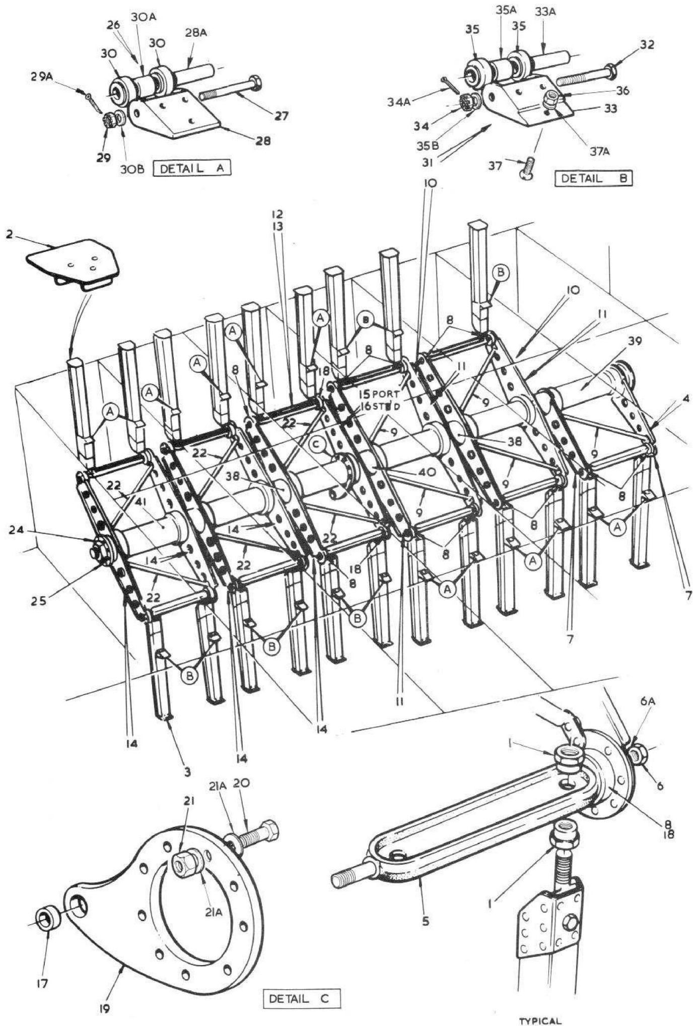
FIG2 WING STRUCTURE
