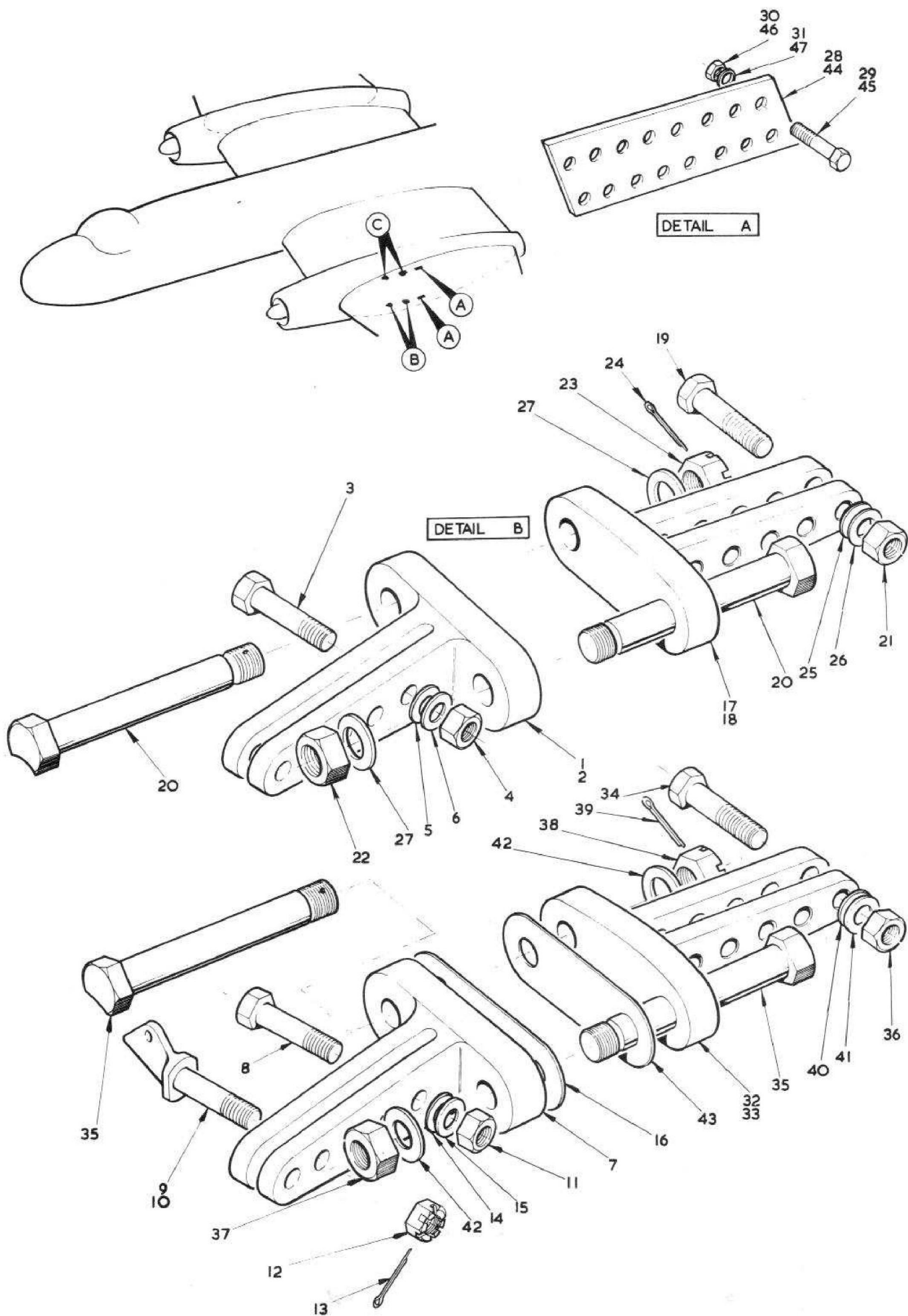
FIG.9 WING STRUCTURE
