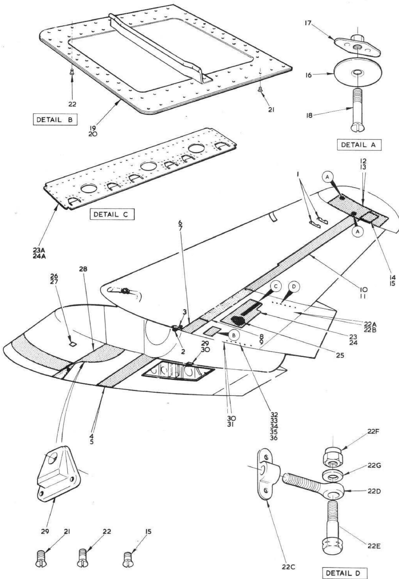
FIG.5 WING STRUCTURE
