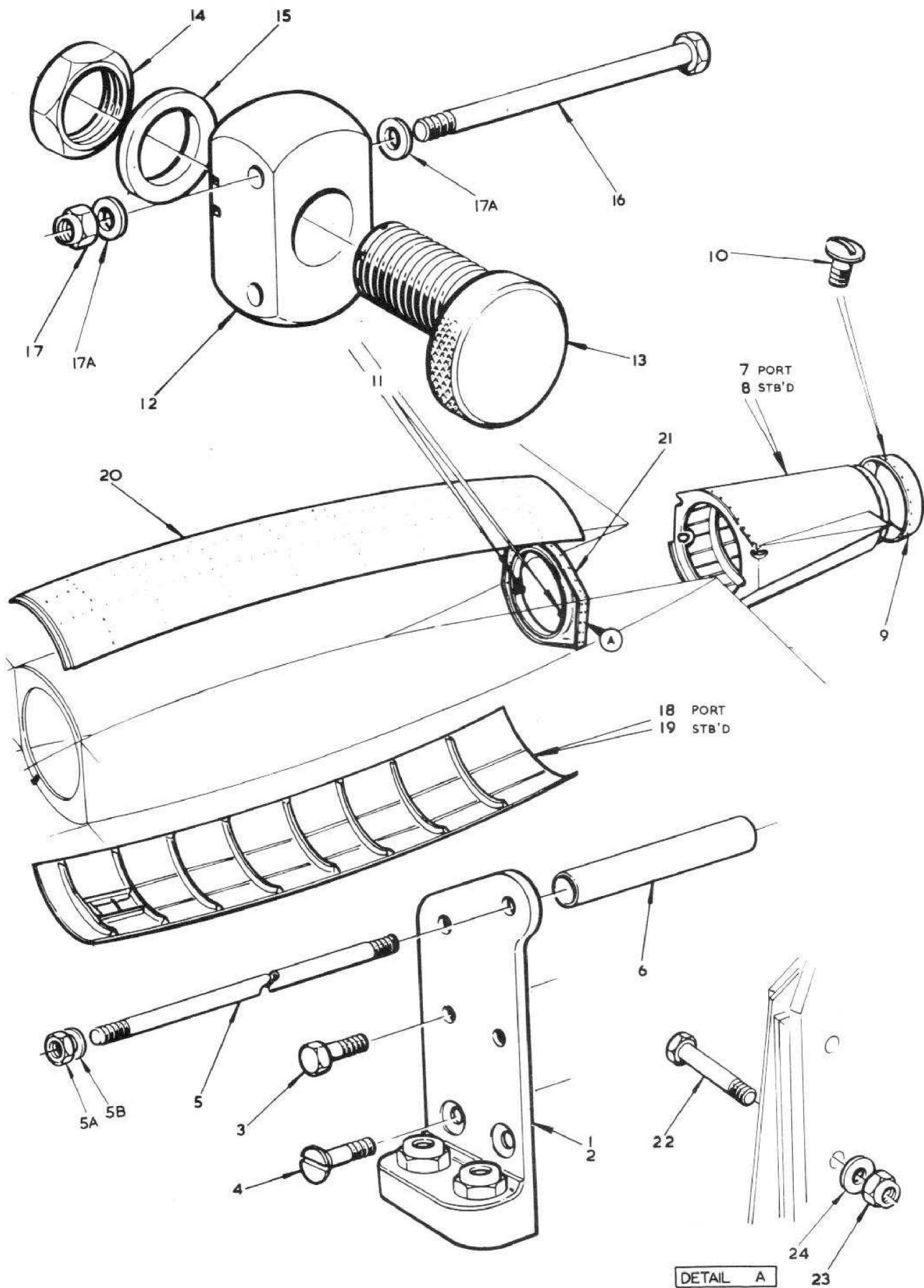
FIG 3 WING STRUCTURE
