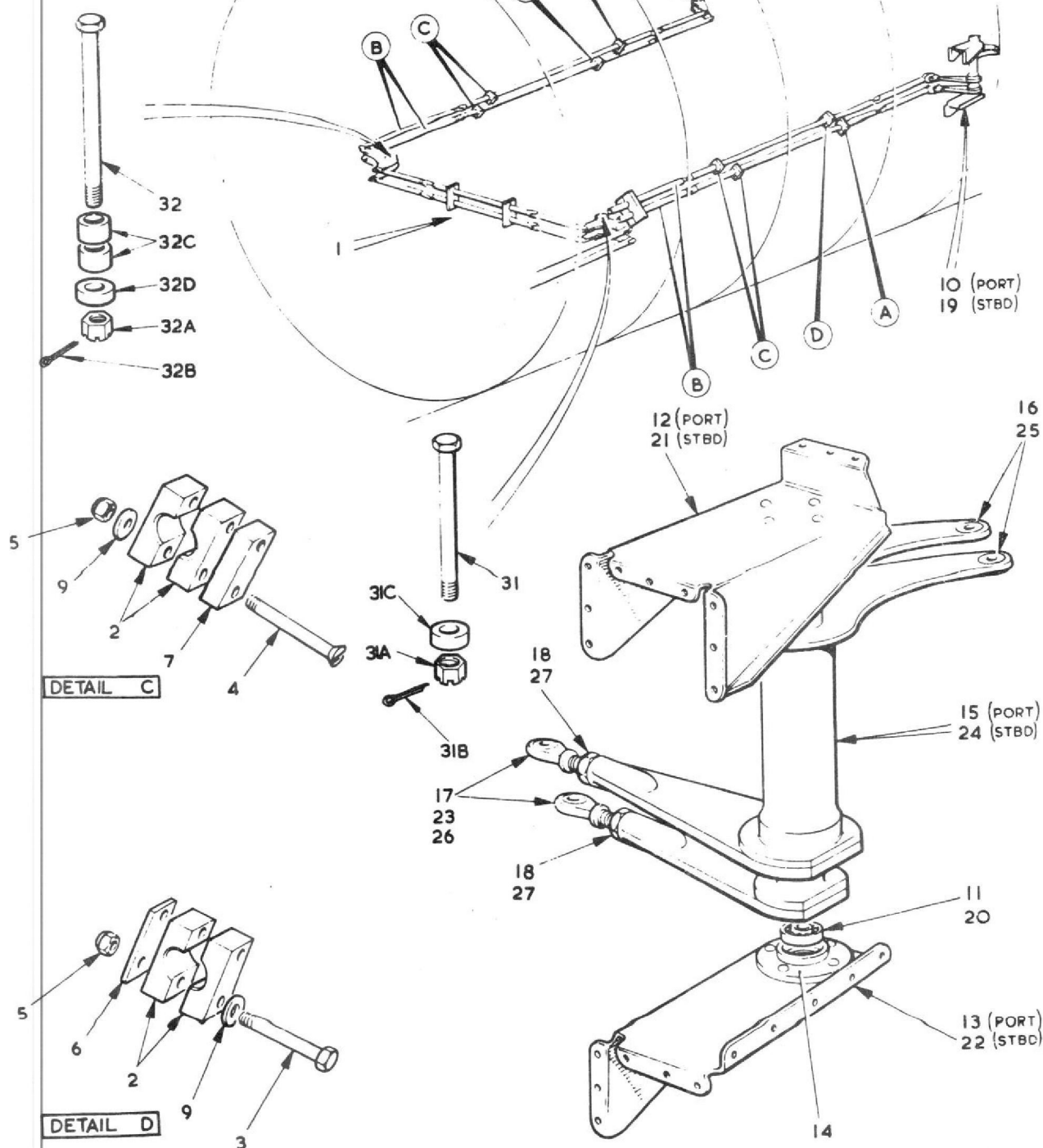
FIG. 1 ENGINE CONTROLS IN CENTRE FUSELAGE
