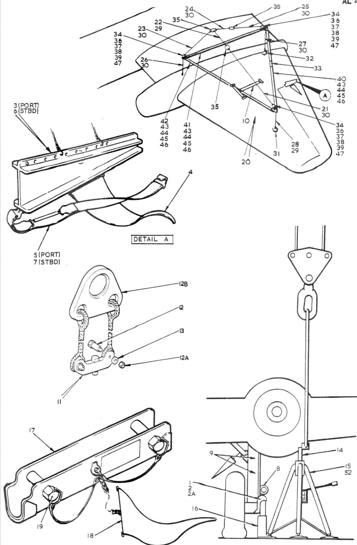
FIG. 3 EQUIPMENT GROUND &amp; MAINTENANCE
