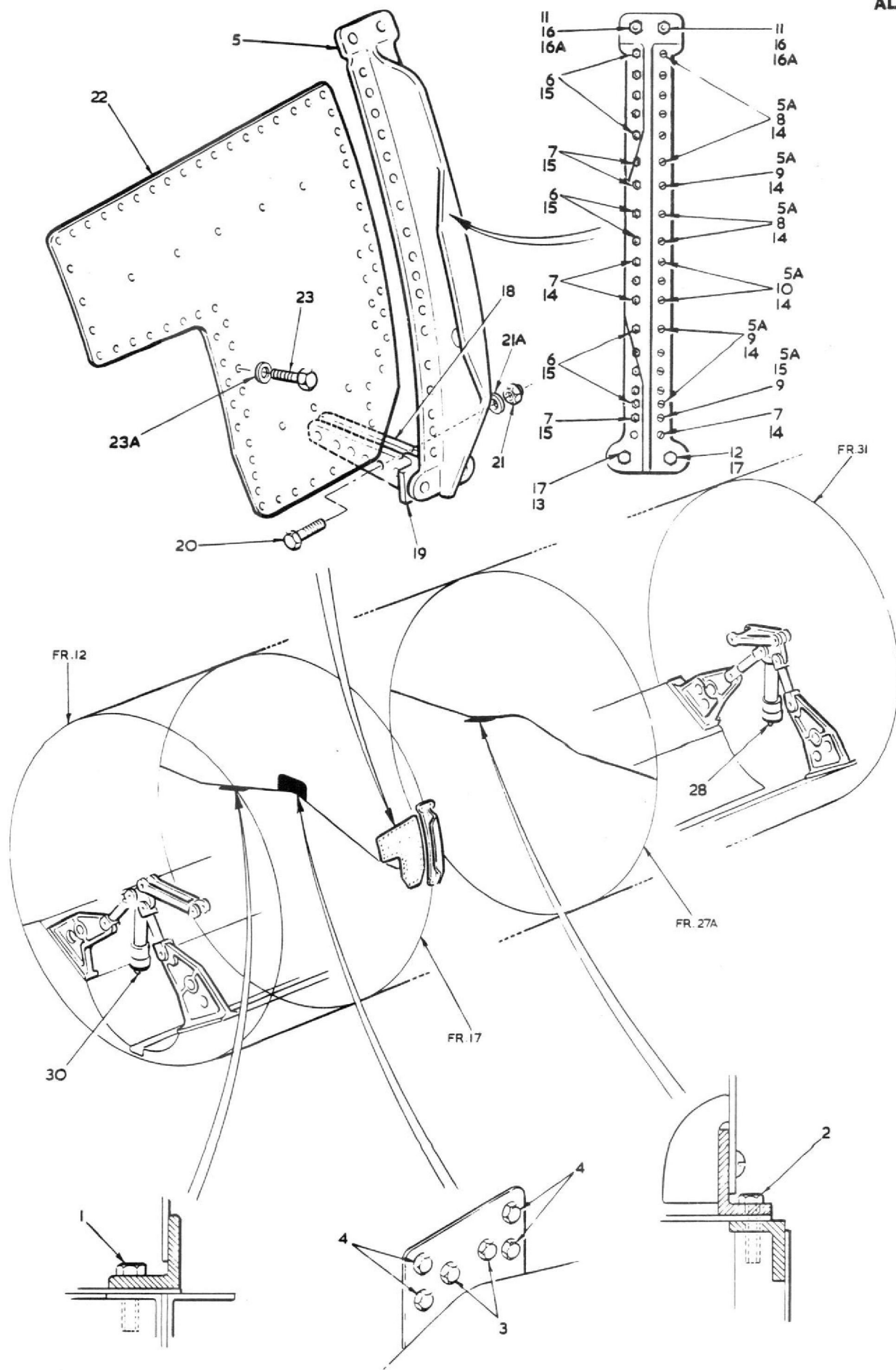
FIG.3 CENTRE FUSELAGE STRUCTURE
