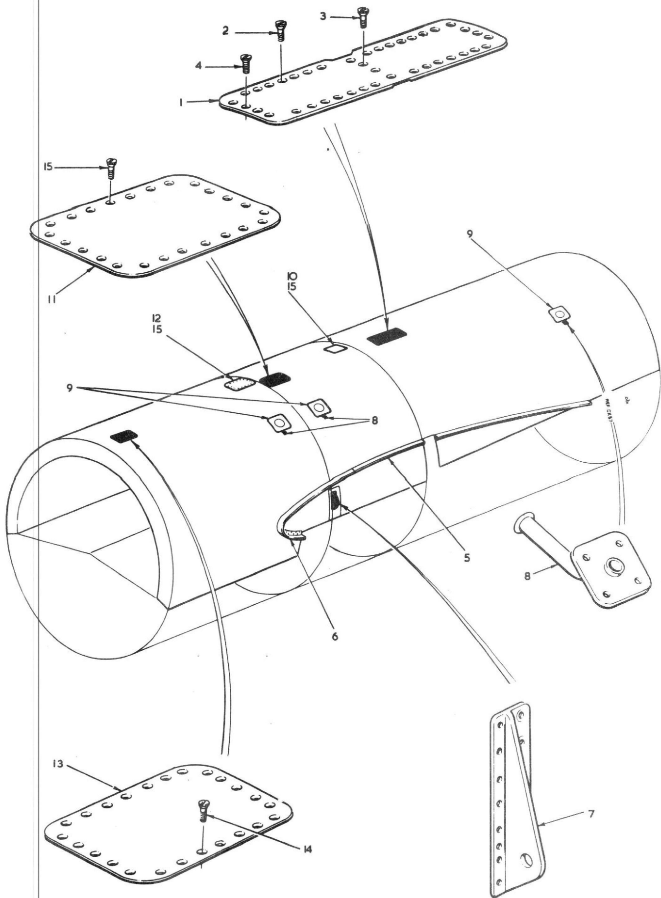
FIG.8 CENTRE FUSELAGE STRUCTURE
