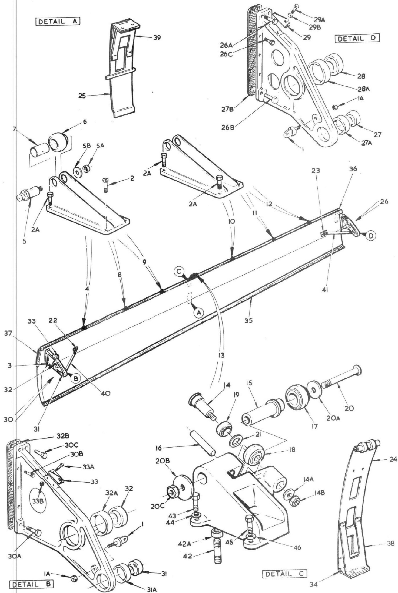
FIG.5 CENTRE FUSELAGE
