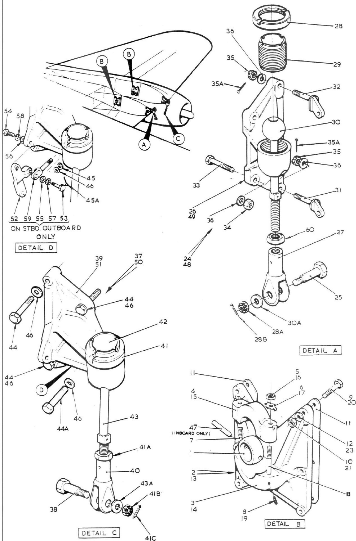
FIG1 ENGINE MOUNTINGS &amp; ATTACHMENTS PORT &amp; STBD
