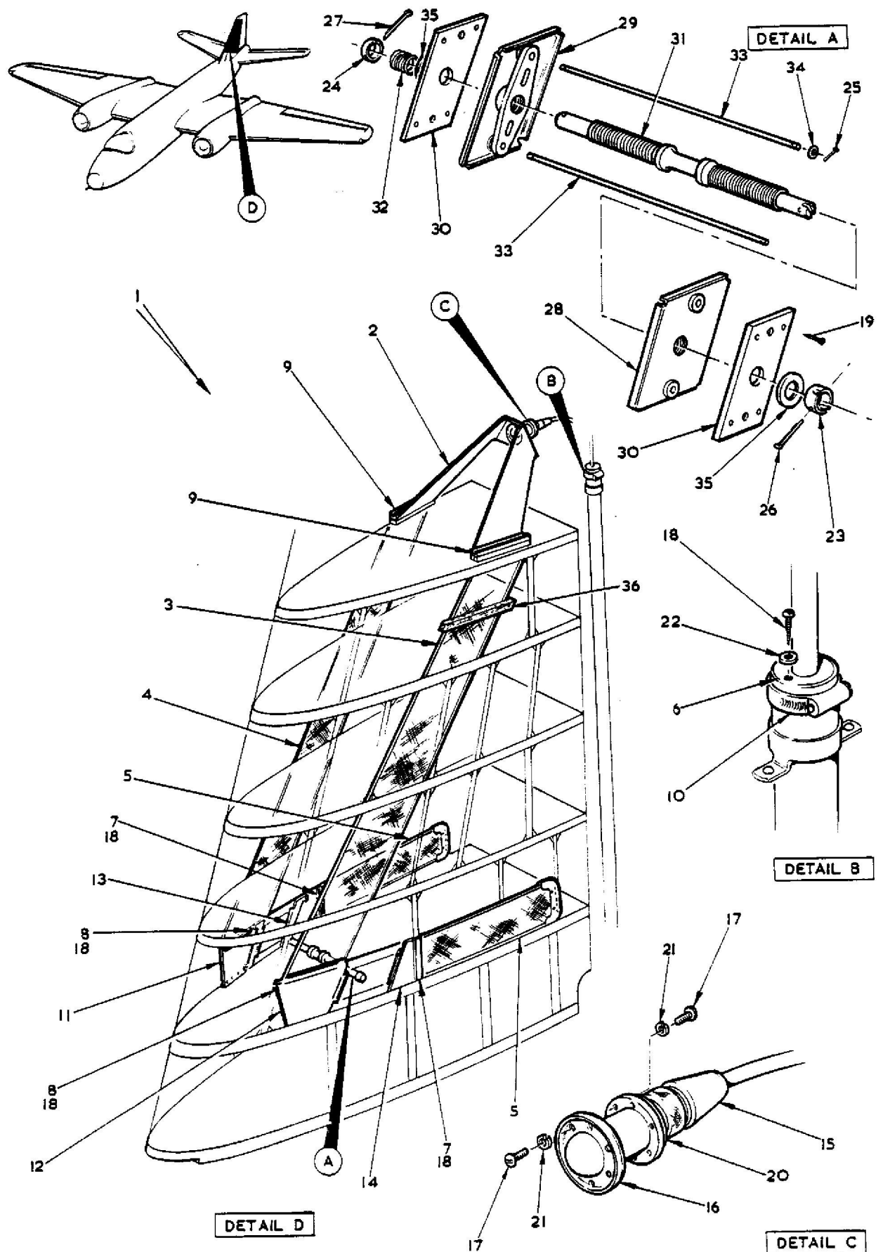
FIG.1 RADAR A.RL 5829 AERIAL INSTALLATION
