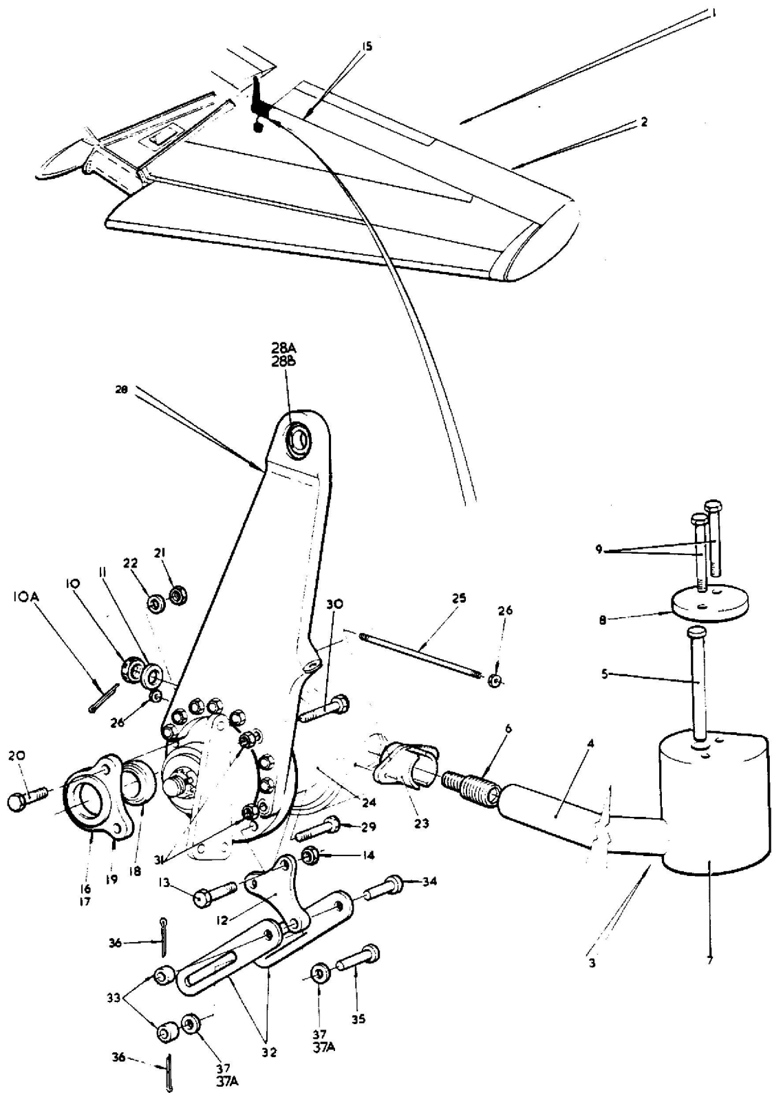
FIG 1 TAIL UNIT
