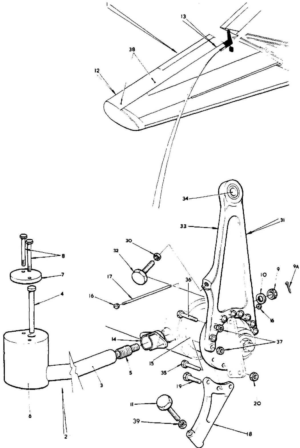
FIG 2 TAIL UNIT
