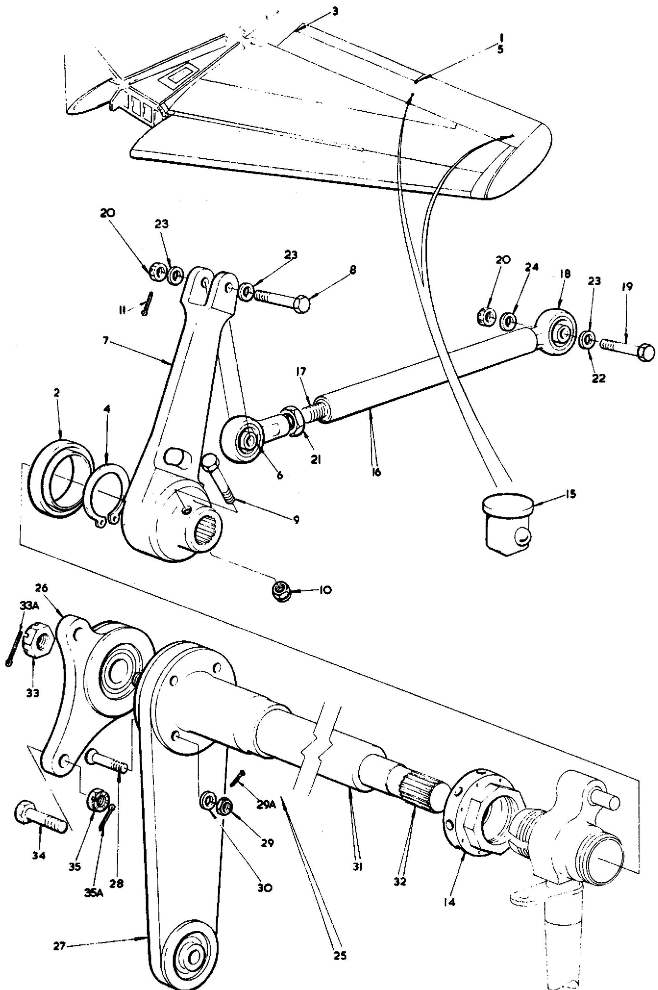
FIG 5 TAIL UNIT
