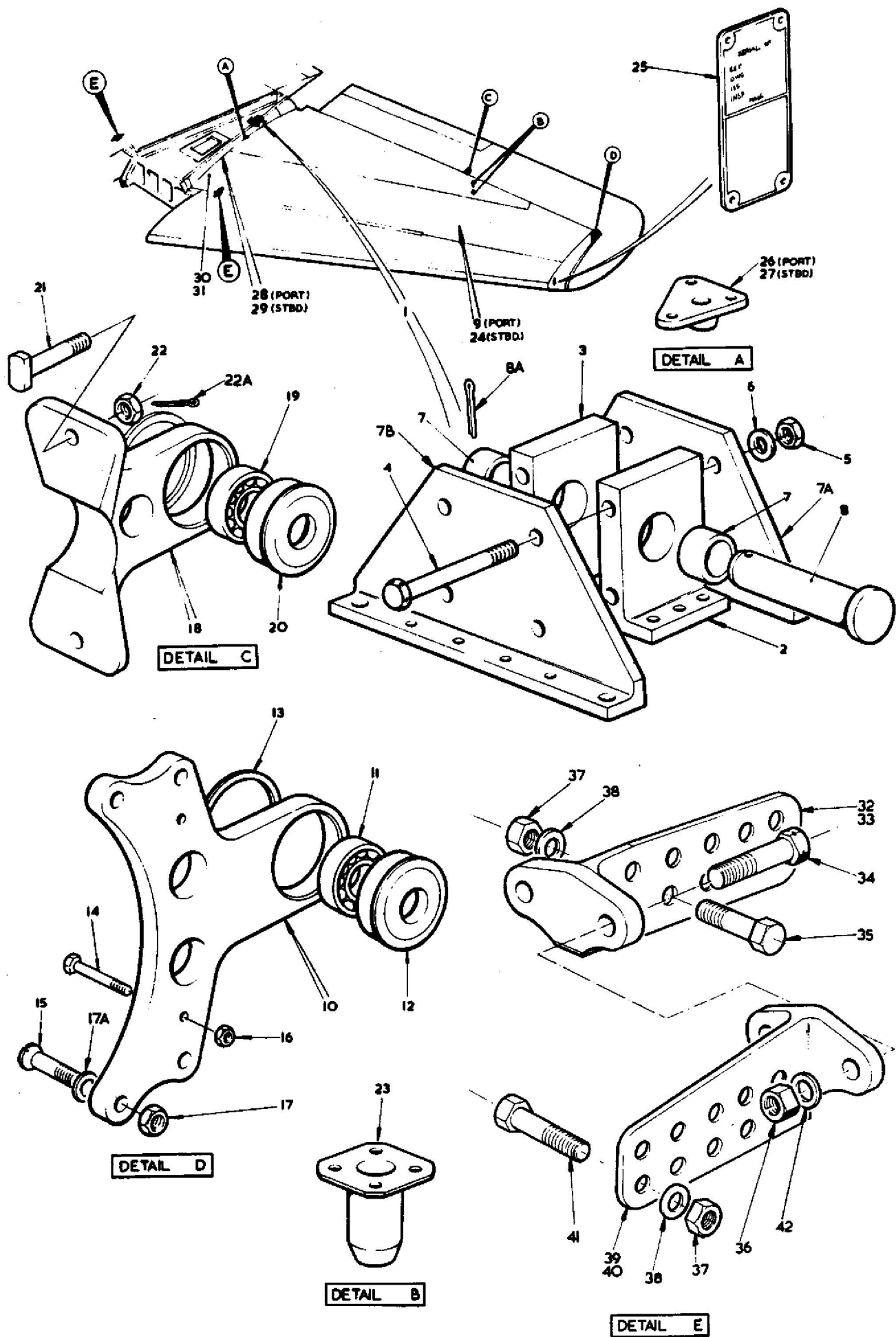
FIG 8 TAILPLANE & ELEVATORS
