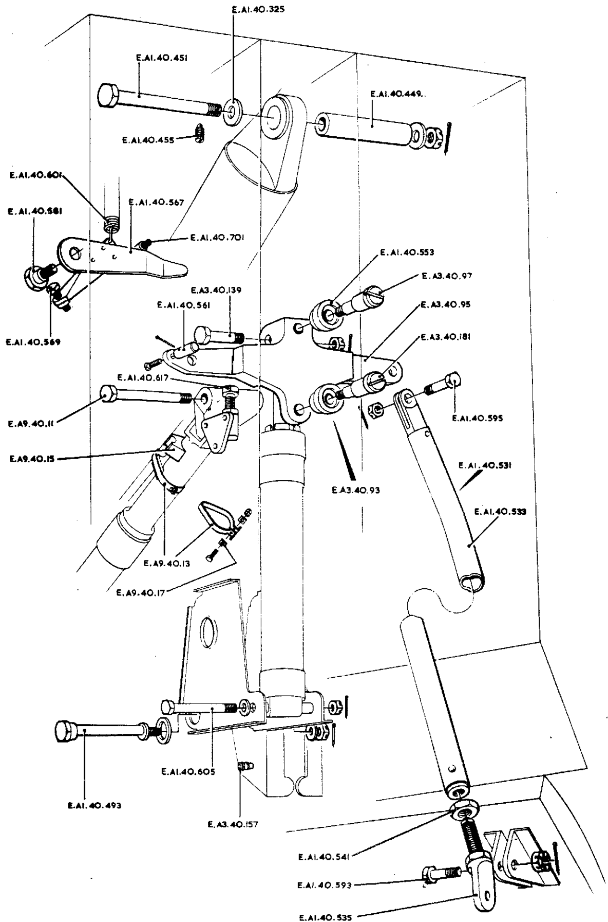
NOSEWHEEL DOOR MECHANISM
