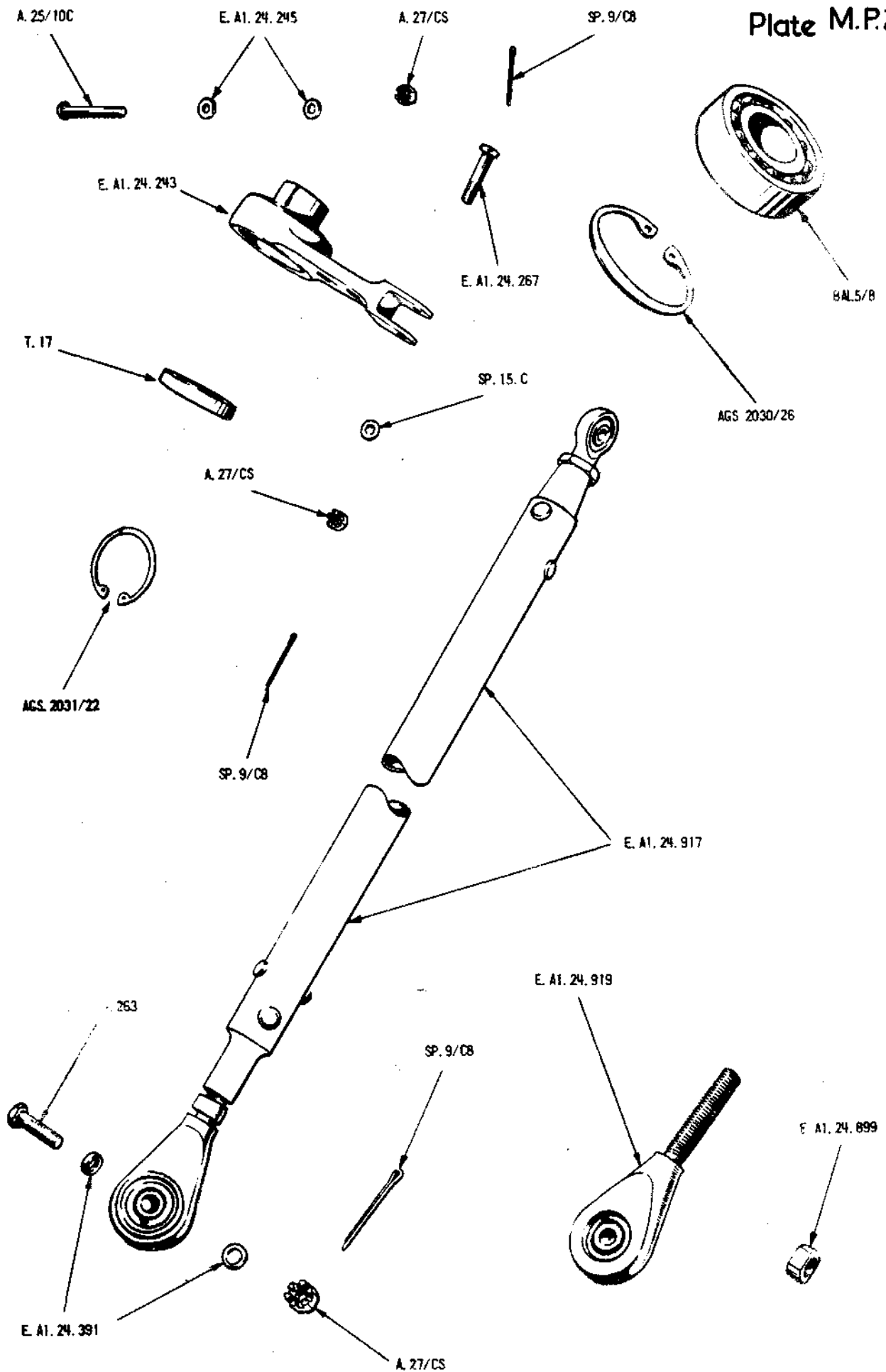
MAIN PLANE - TAB PUSH ROD AND LEVER
