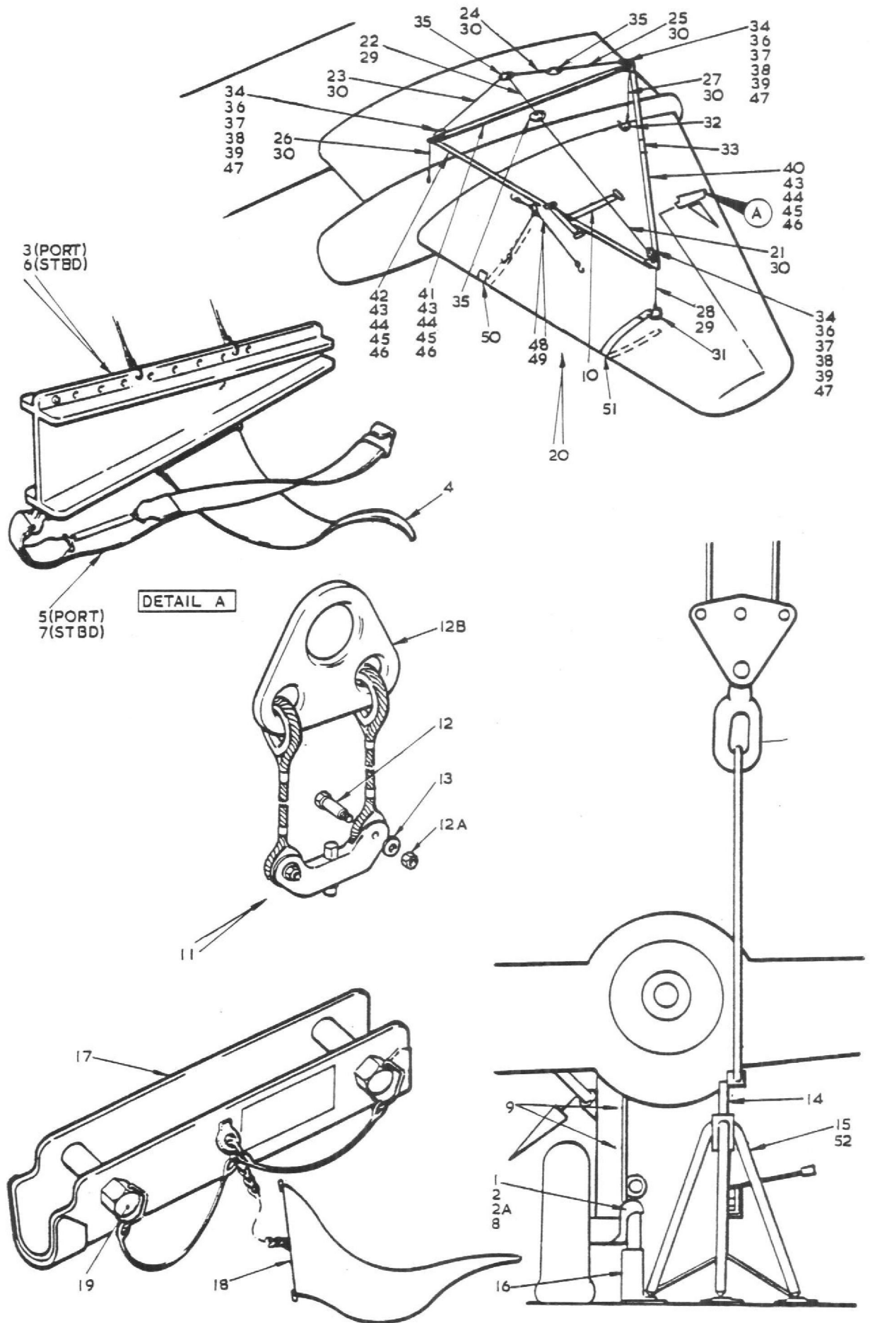
FIG. 3 EQUIPMENT GROUND &amp; MAINTENANCE
