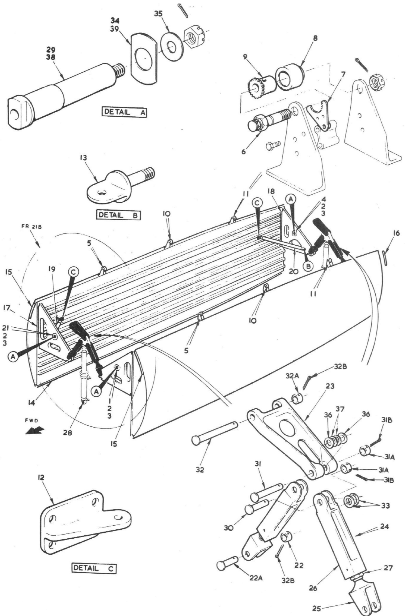
FIG.3 CENTRE FUSELAGE STRUCTURE
