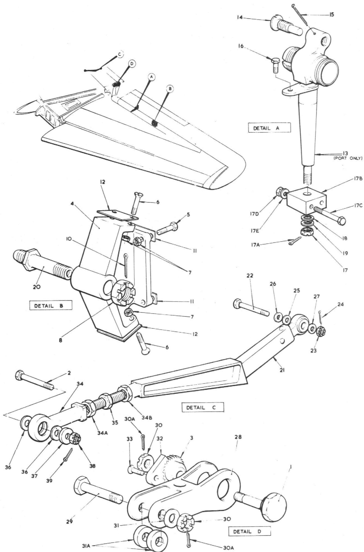
FIG 6 TAIL UNIT
