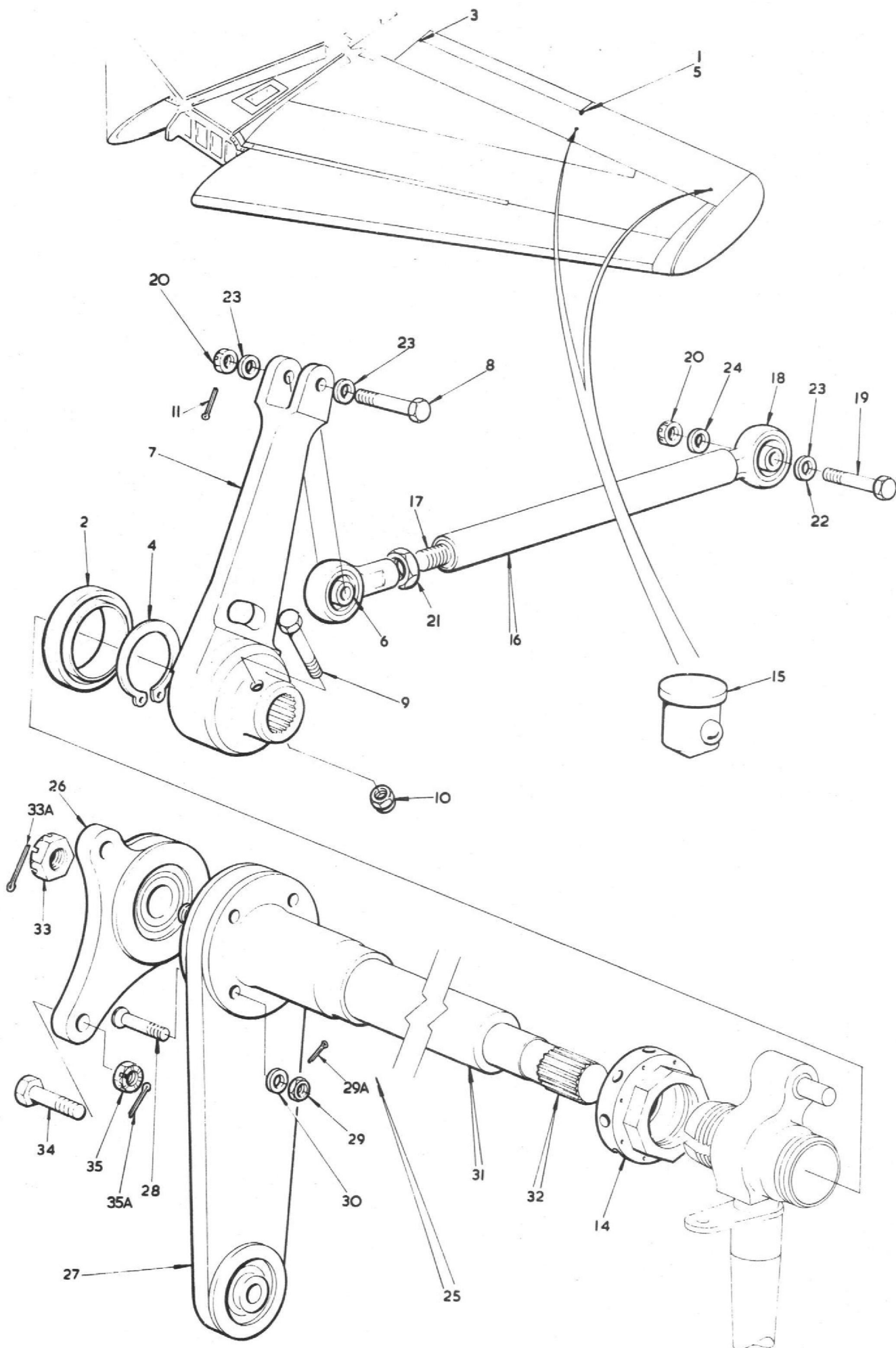
FIG 5 TAIL UNIT
