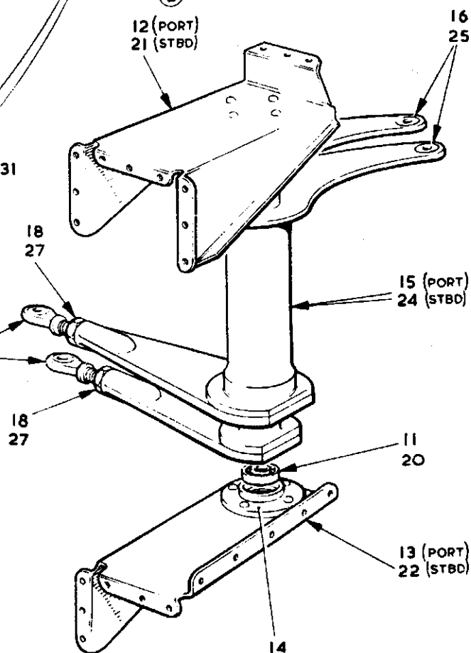
FIG. 1 ENGINE CONTROLS IN CENTRE FUSELAGE
