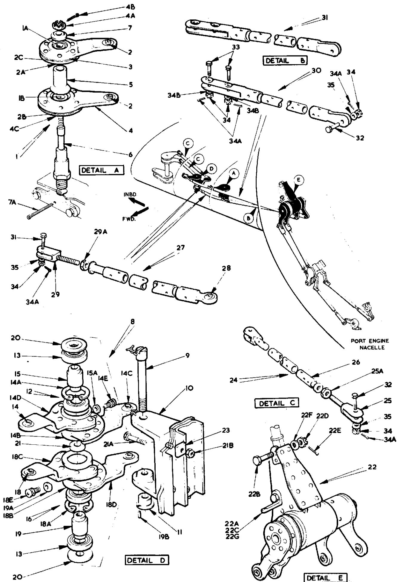
FIG.1 ENGINE CONTROLS IN PORT MAINPLANE
