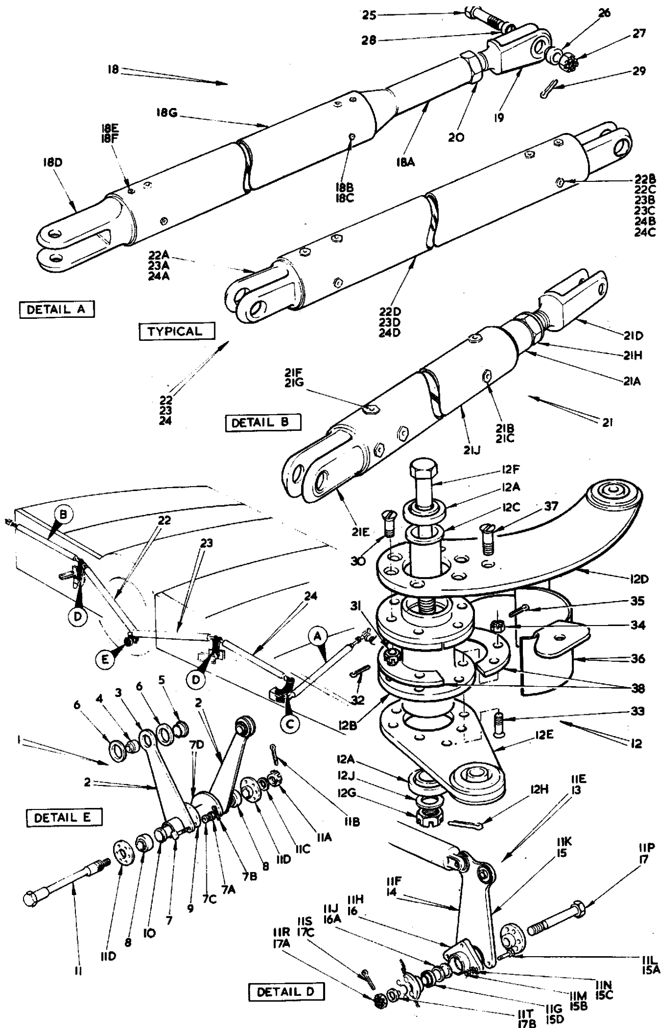
FIG. 1 AILERON CONTROLS IN WING
