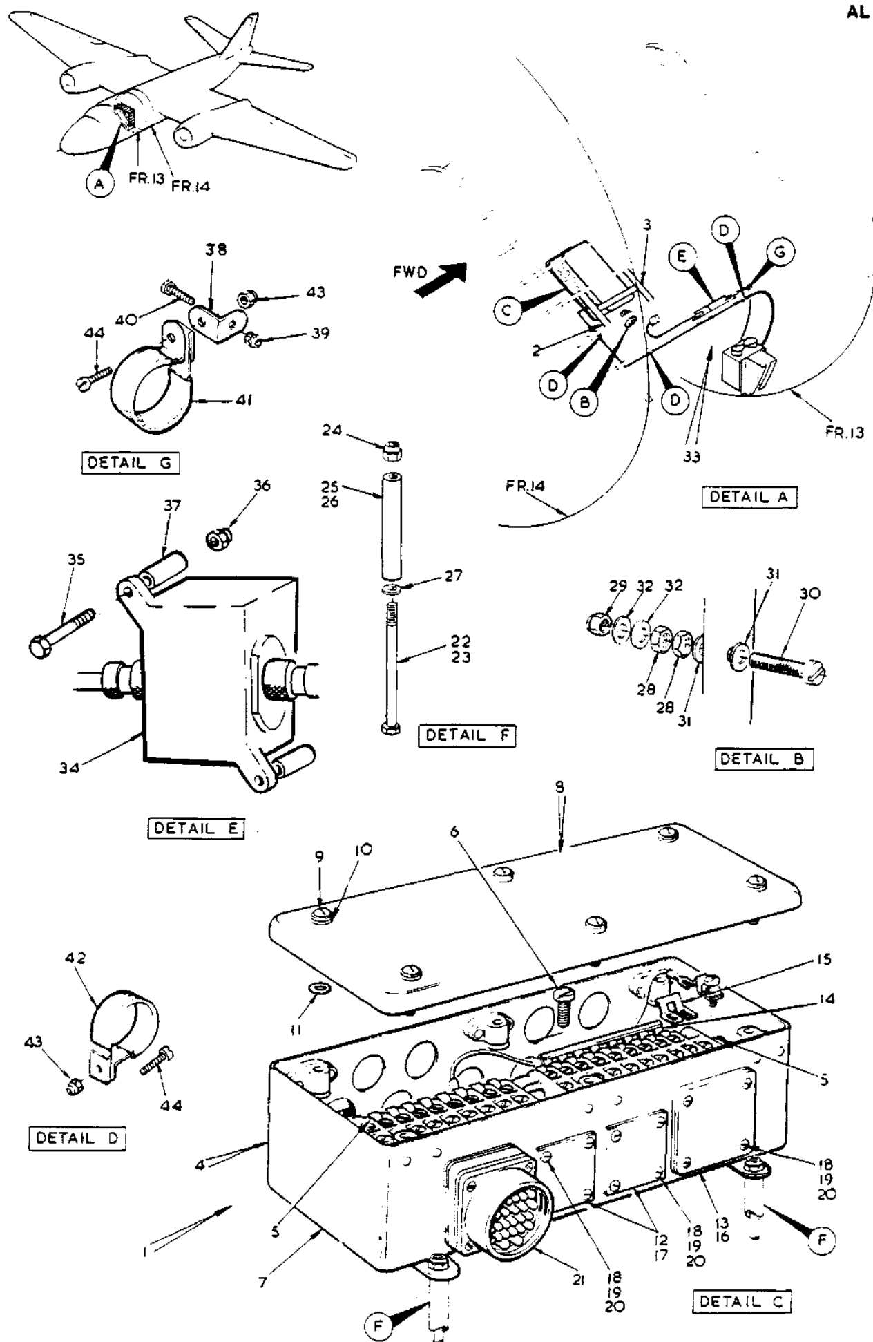
FIG. 3 ELECTRICAL EQUIPMENT IN CENTRE FUSELAGE
