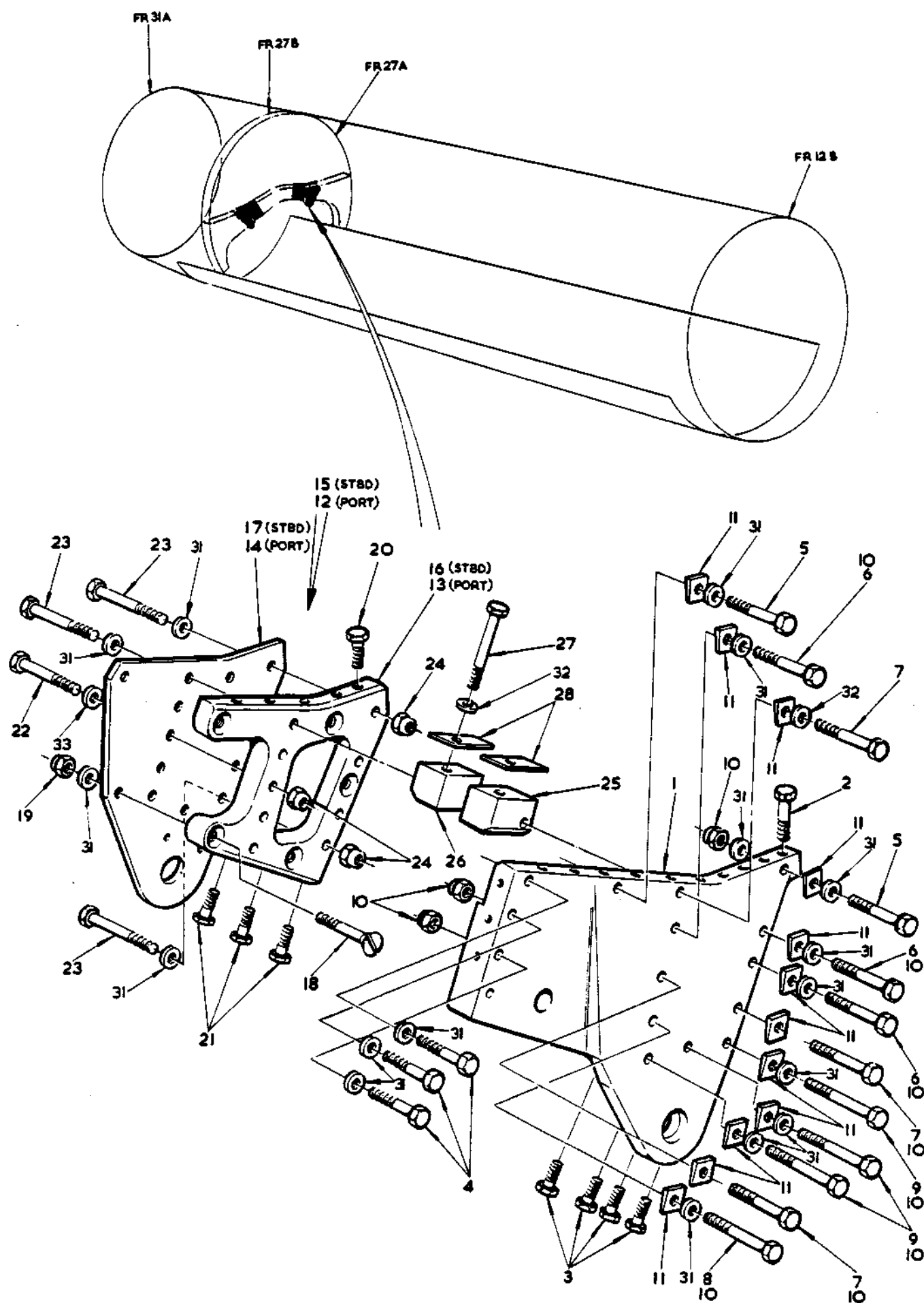
FIG 7 CENTRE FUSELAGE STRUCTURE
