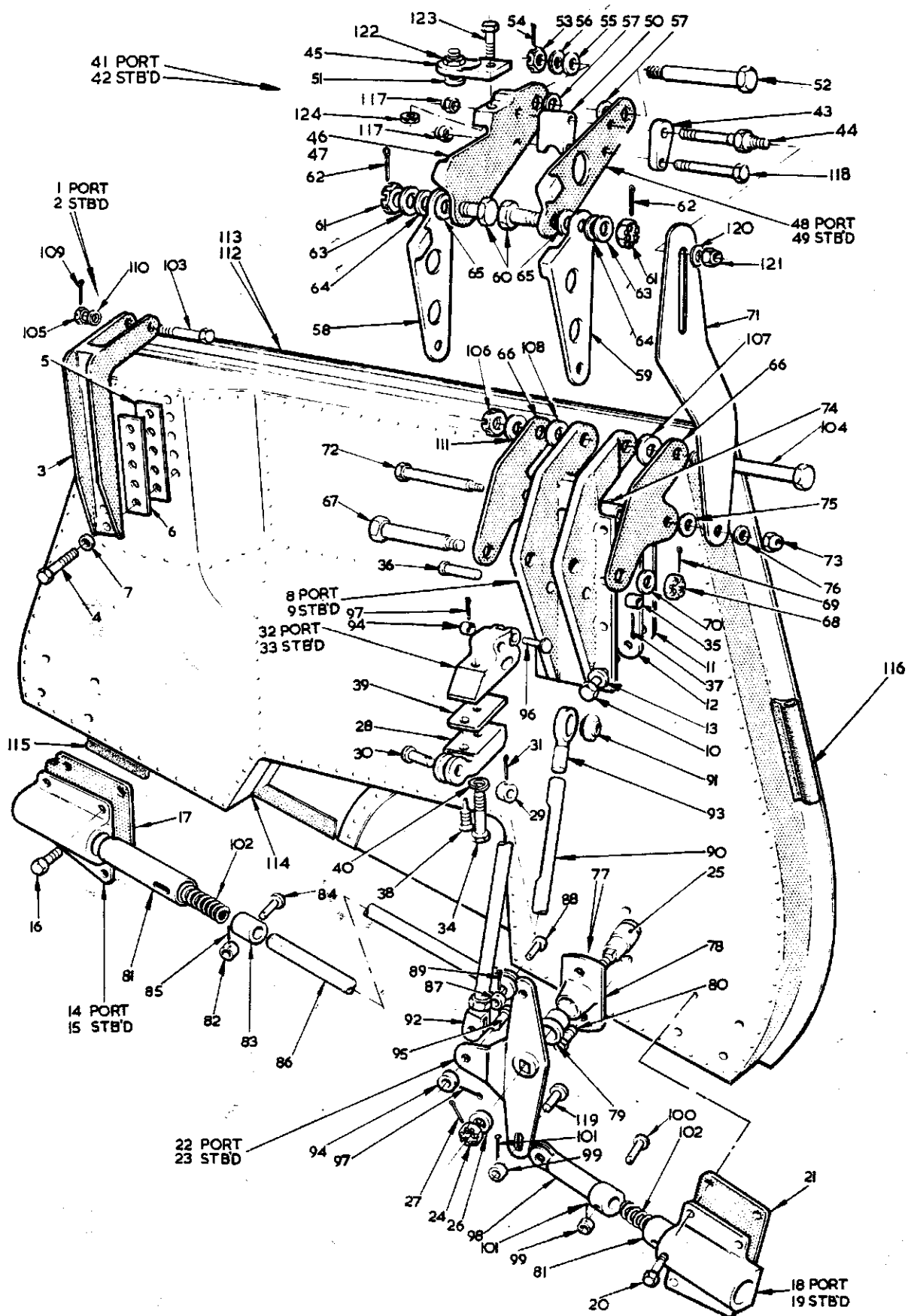
FIG 1 UNDERCARRIAGE DOOR COMPLETE WITH MECHANISM PORT & STBD
