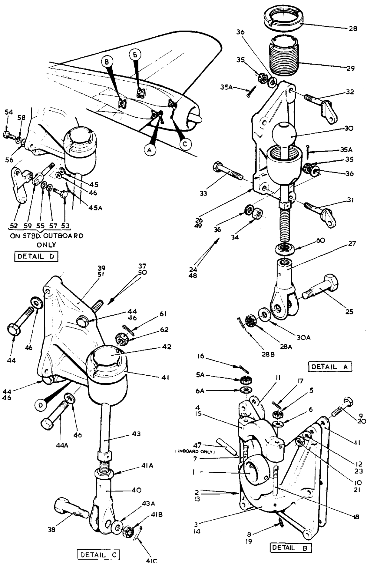
FIG1 ENGINE MOUNTINGS &amp; ATTACHMENTS PORT &amp; STBD
