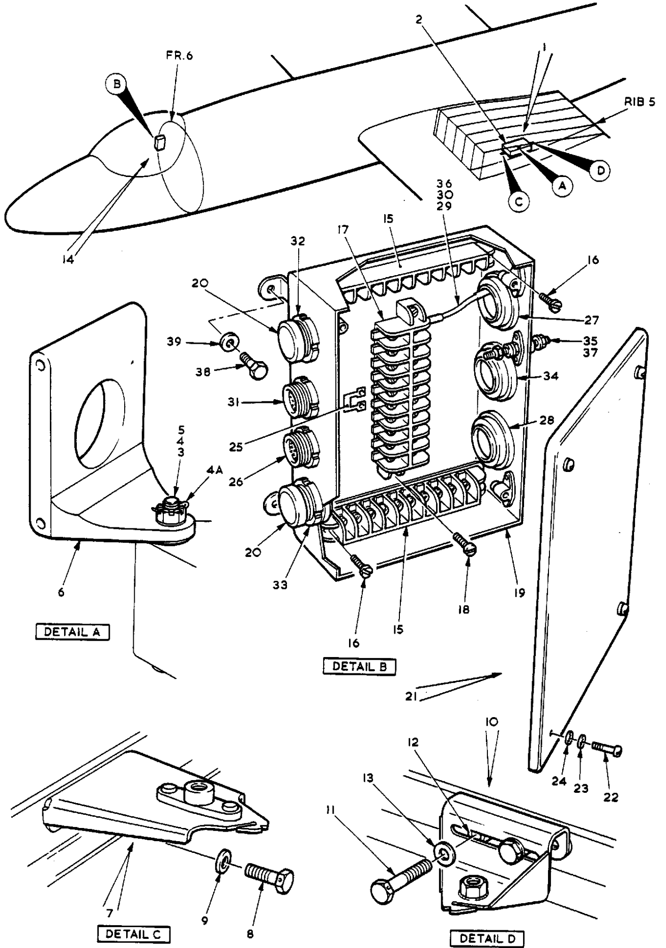
FIG. 1 RADAR, A.R.I.5885, BLUE SILK, INSTALLATION
