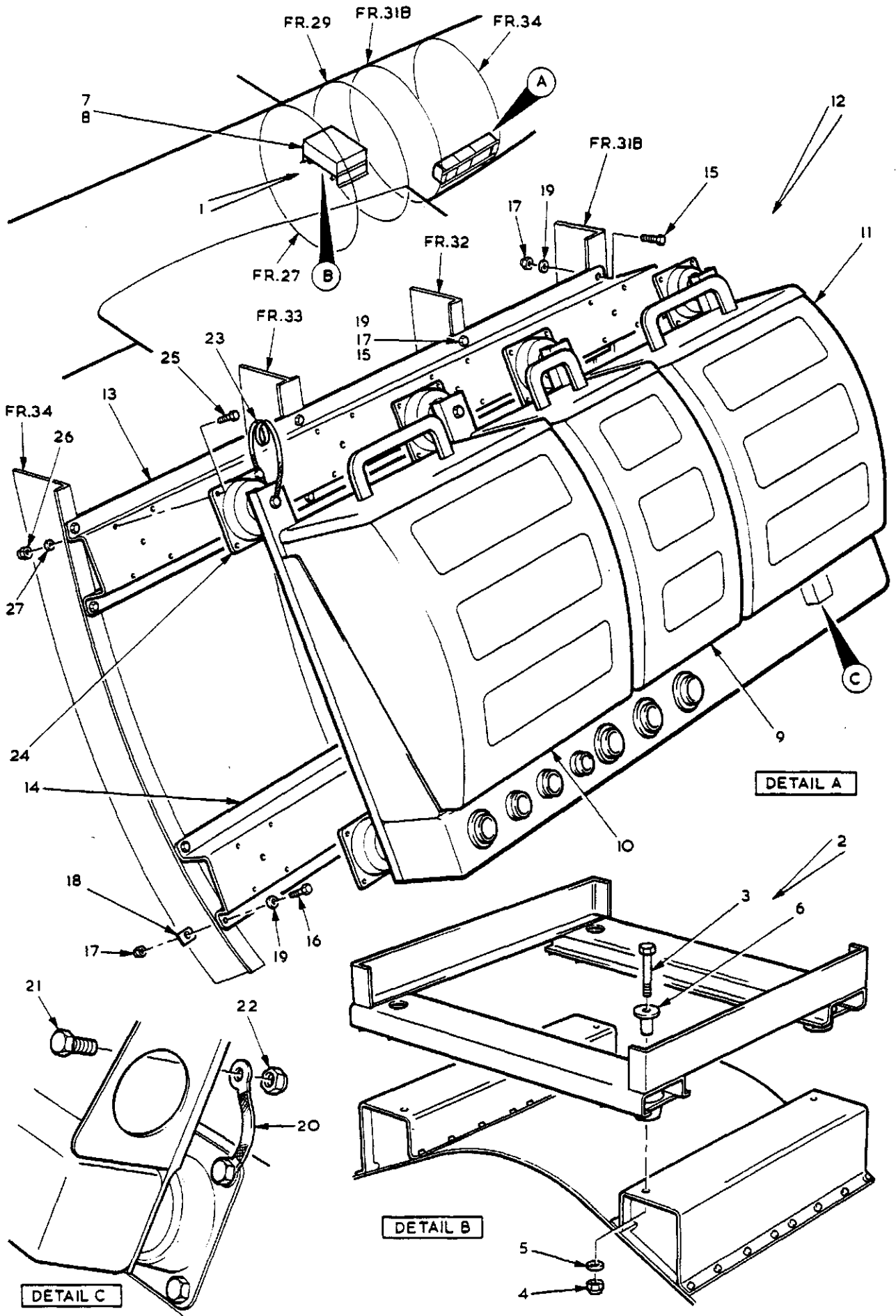
FIG. 3 RADAR, A.R.I.5885, BLUE SILK, INSTALLATION
