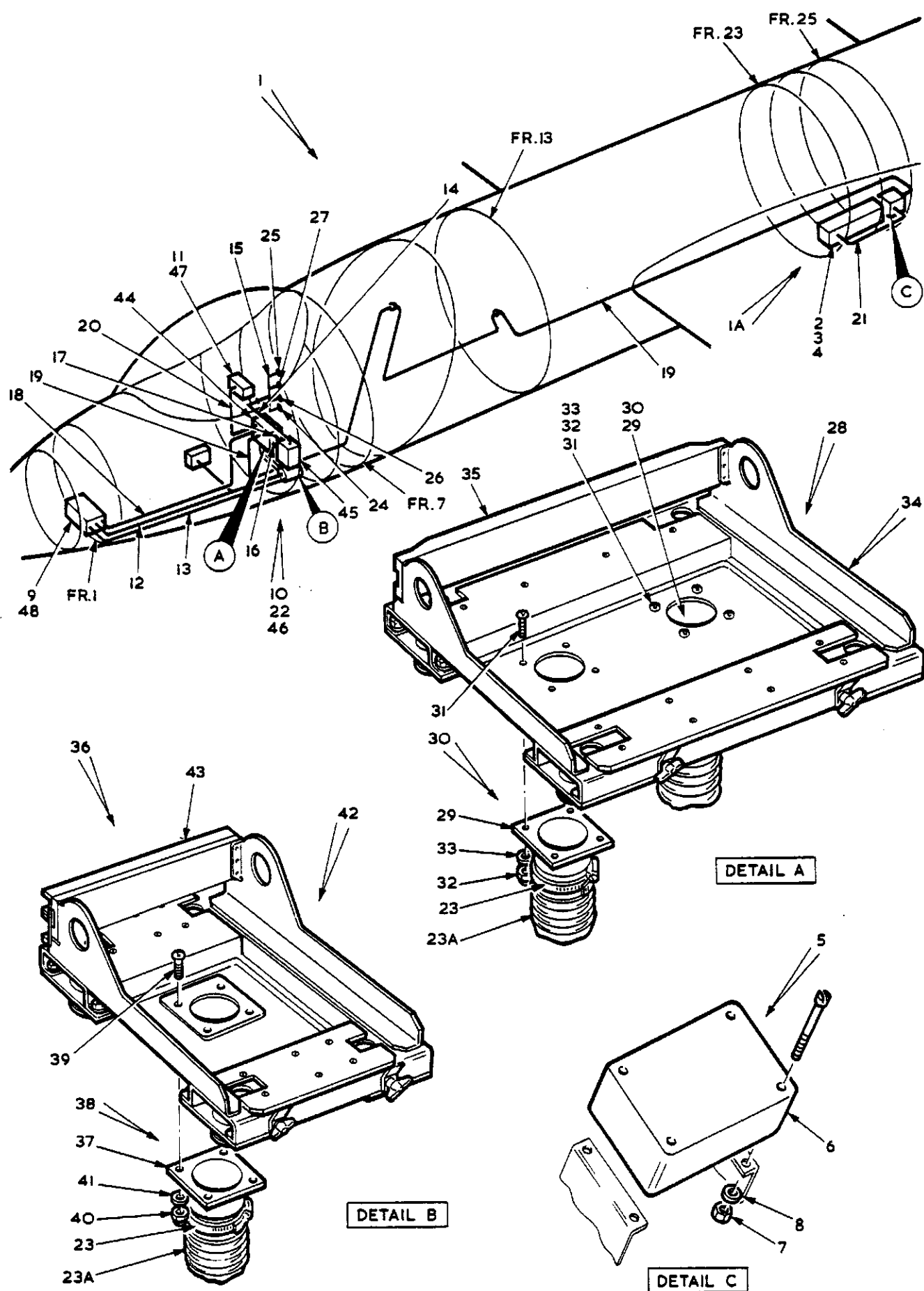
FIG. 1 RADIO, A.R.I.20376, DECCA MK.1 (AIR) INSTALLATION CODE Z
