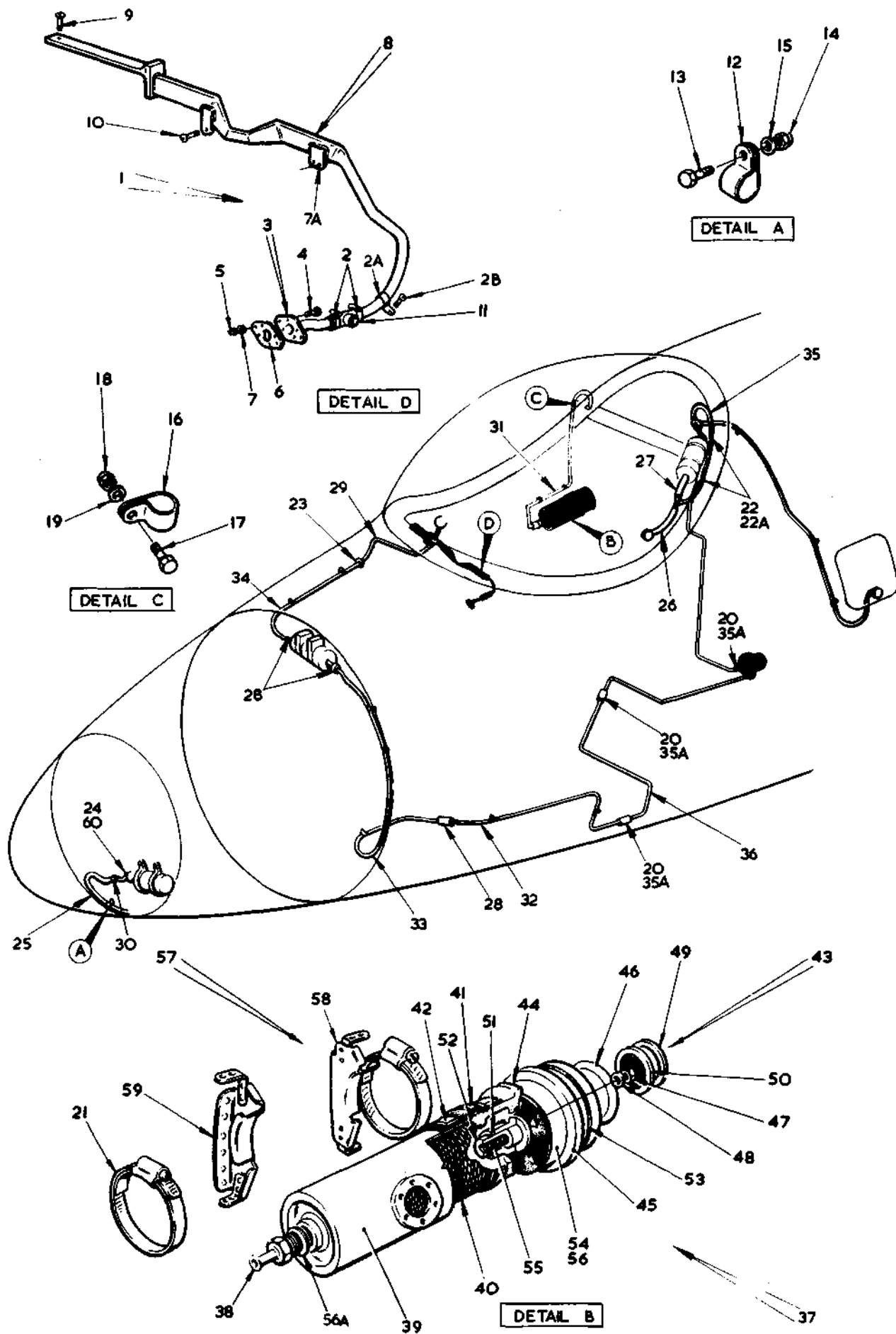
FIG. 2 DE-MISTING SYSTEM
