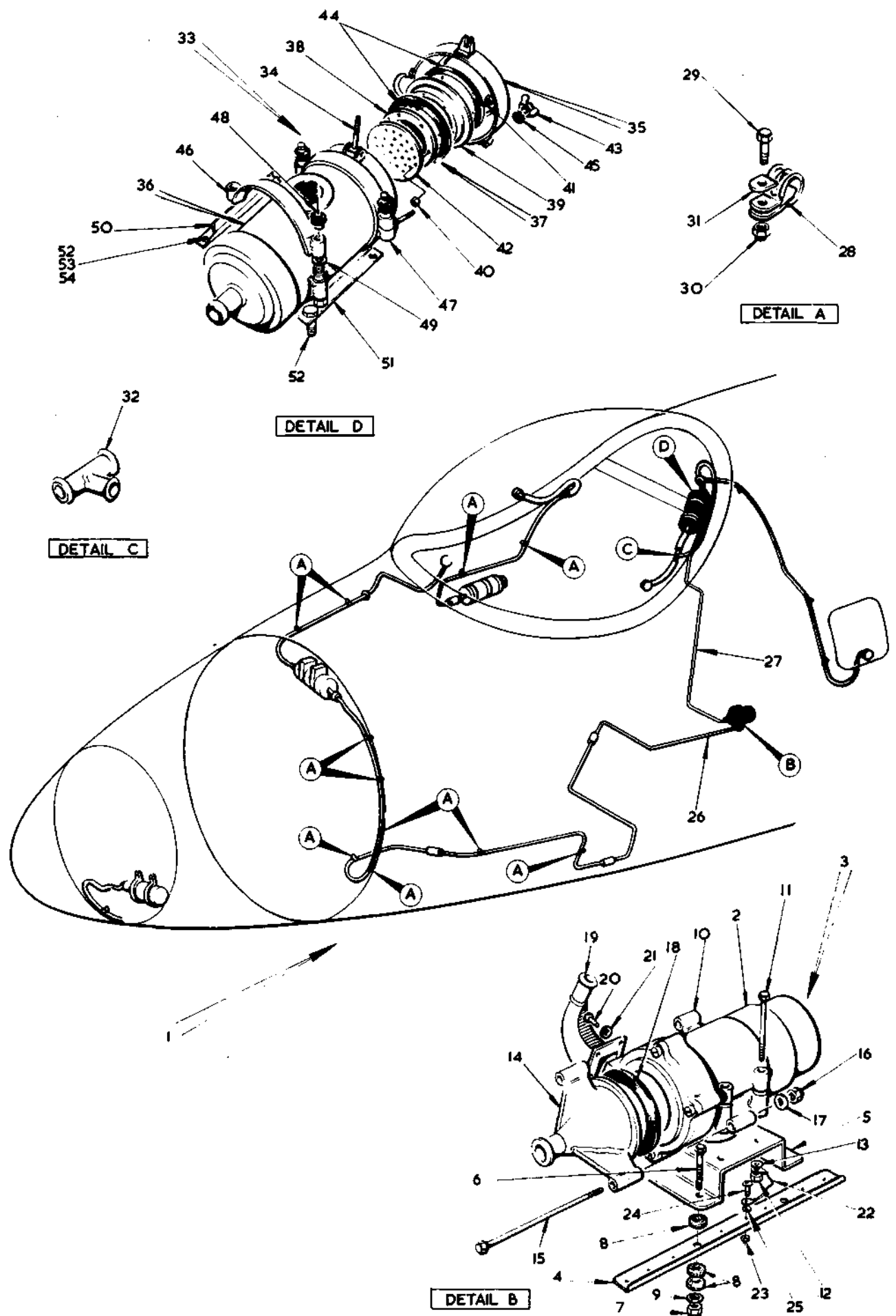
FIG.1 DE-MISTING SYSTEM
