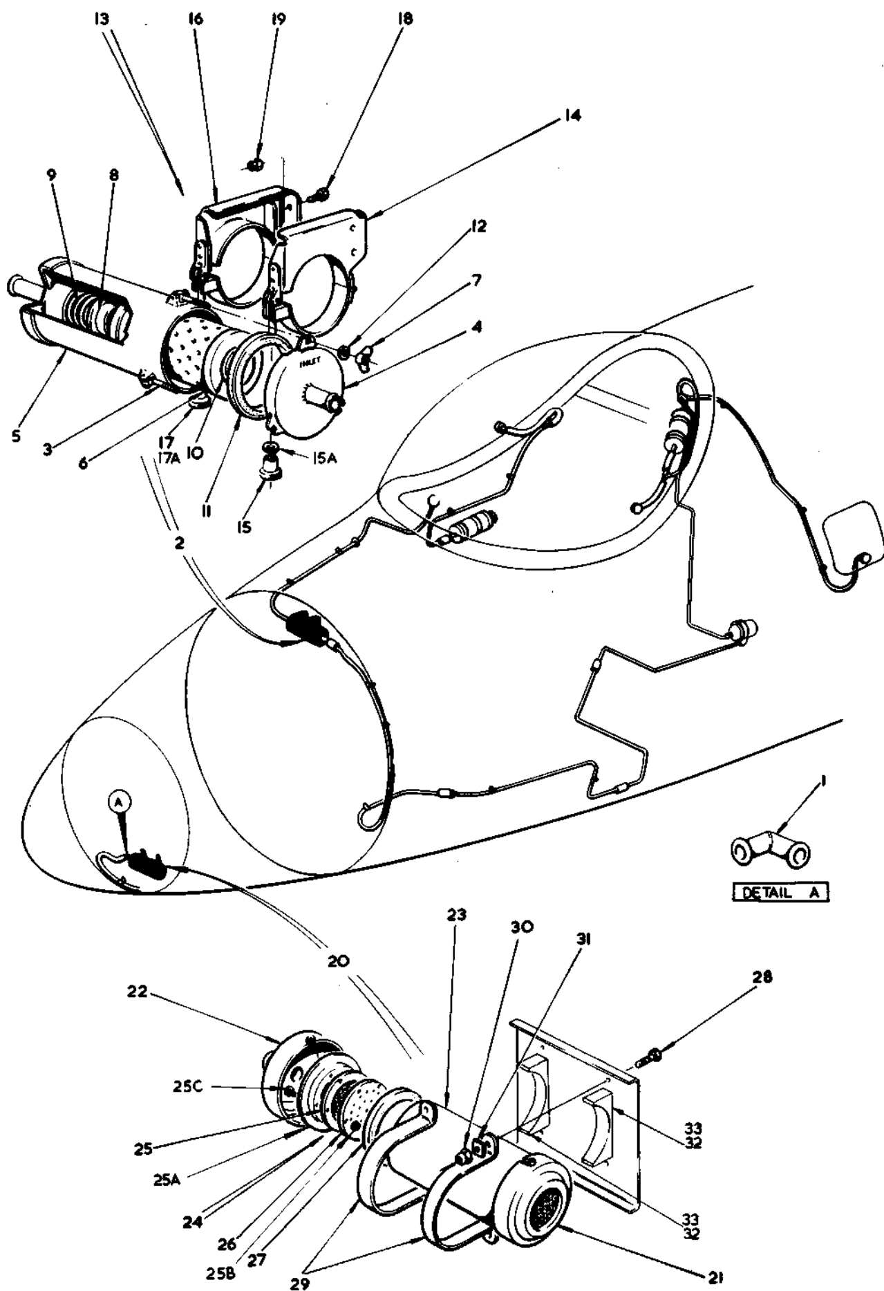
FIG. 3. DE-MISTING SYSTEM
