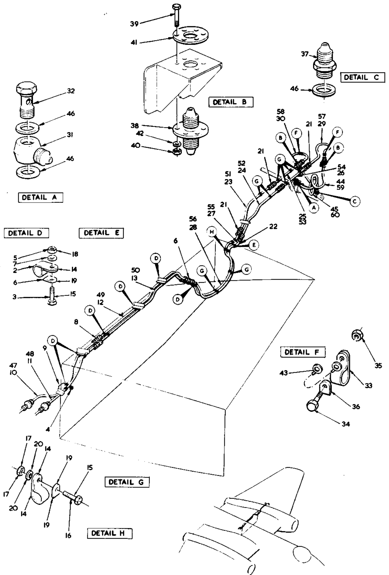
FIG.24 HYDRAULIC SYSTEM
