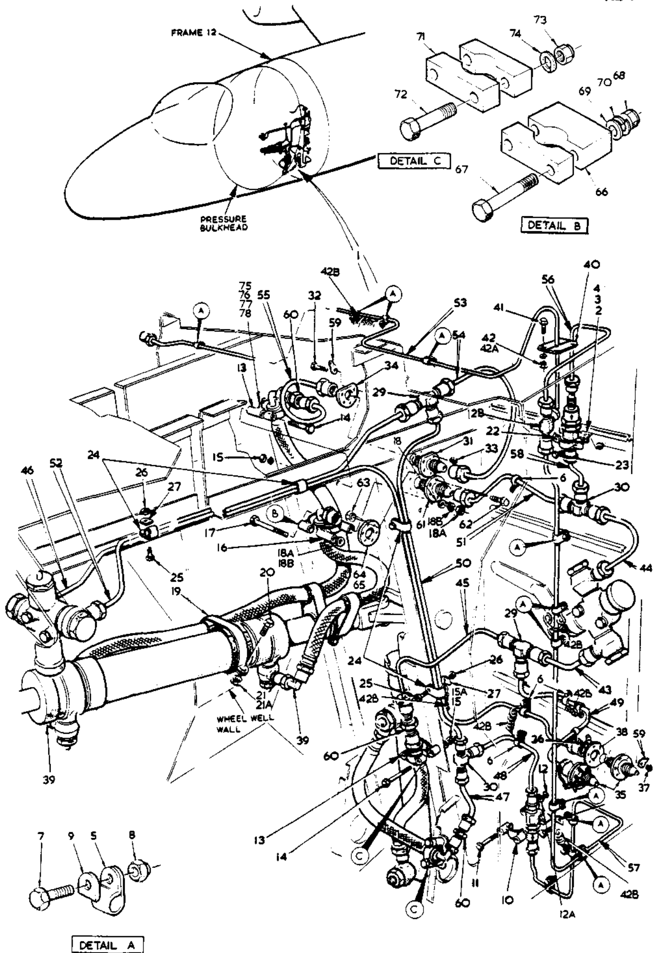
FIG. 6 HYDRAULIC SYSTEM
