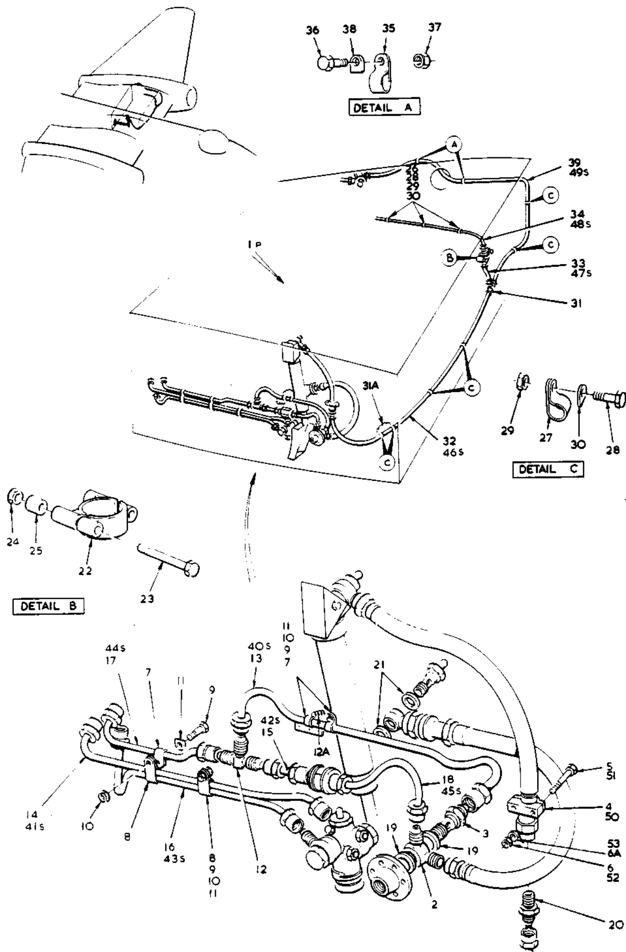
FIG.25 HYDRAULIC SYSTEM
