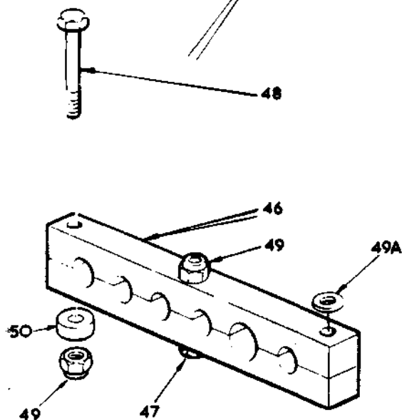
FIG. 4 HYDRAULIC SYSTEM
