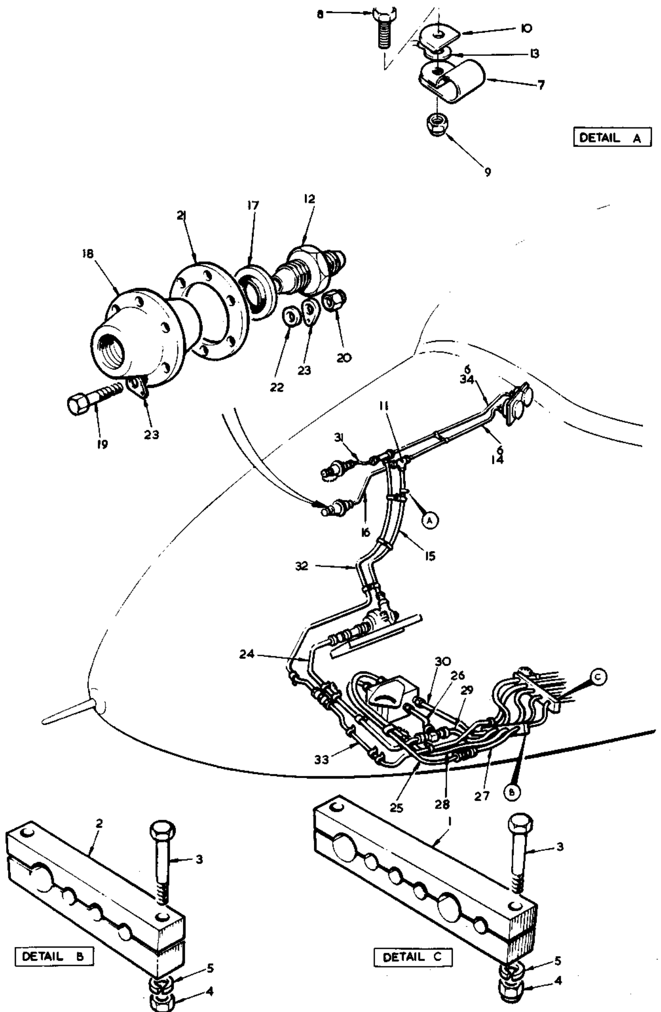
FIG.3 HYDRAULIC SYSTEM
