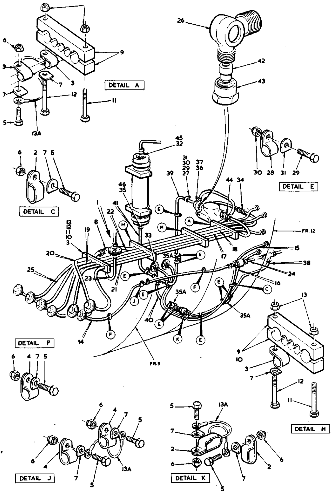
FIG. 5 HYDRAULIC SYSTEM
