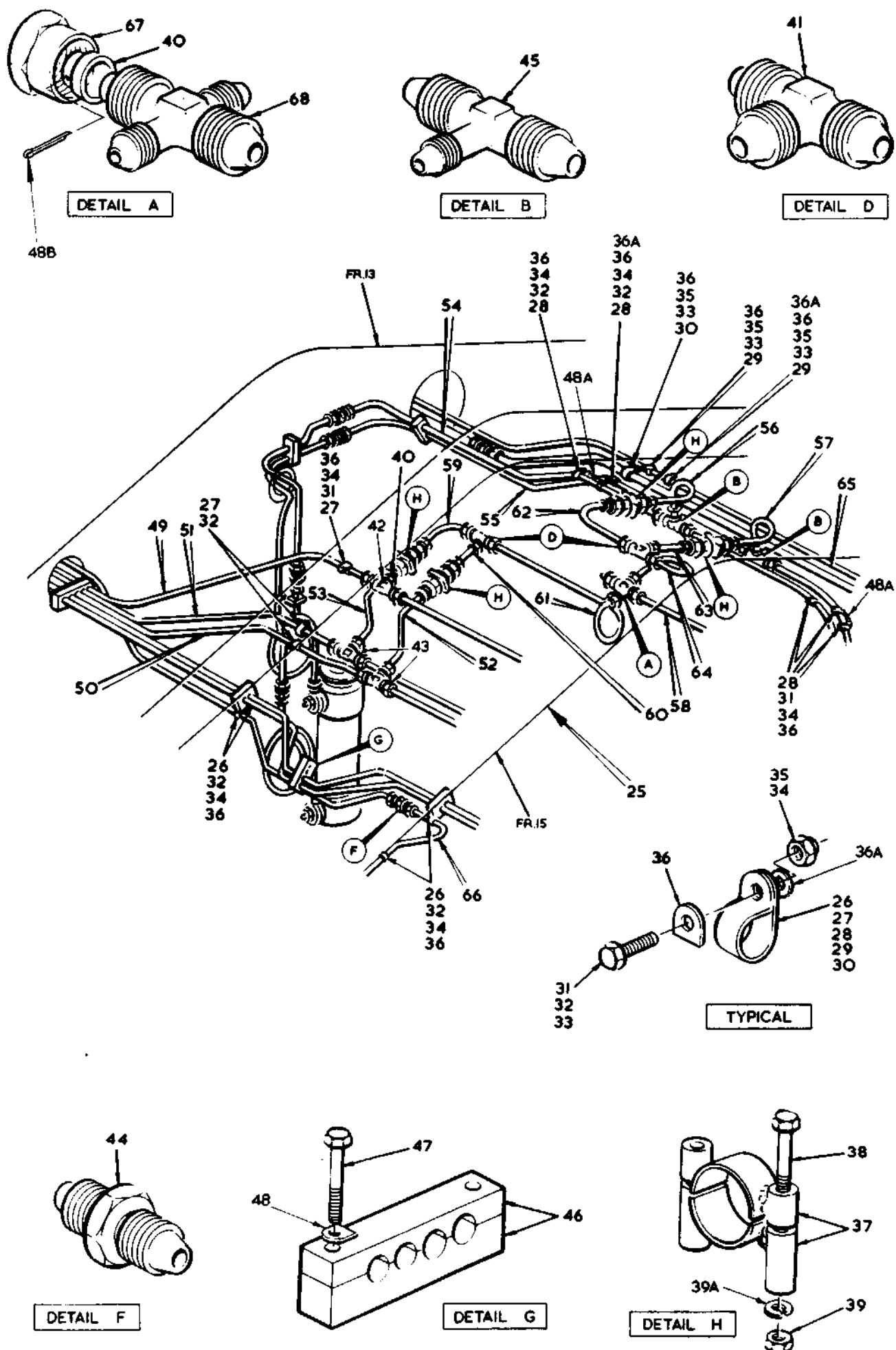
FIG. 18 HYDRAULIC SYSTEM
