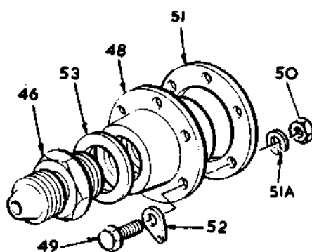
DETAIL L
