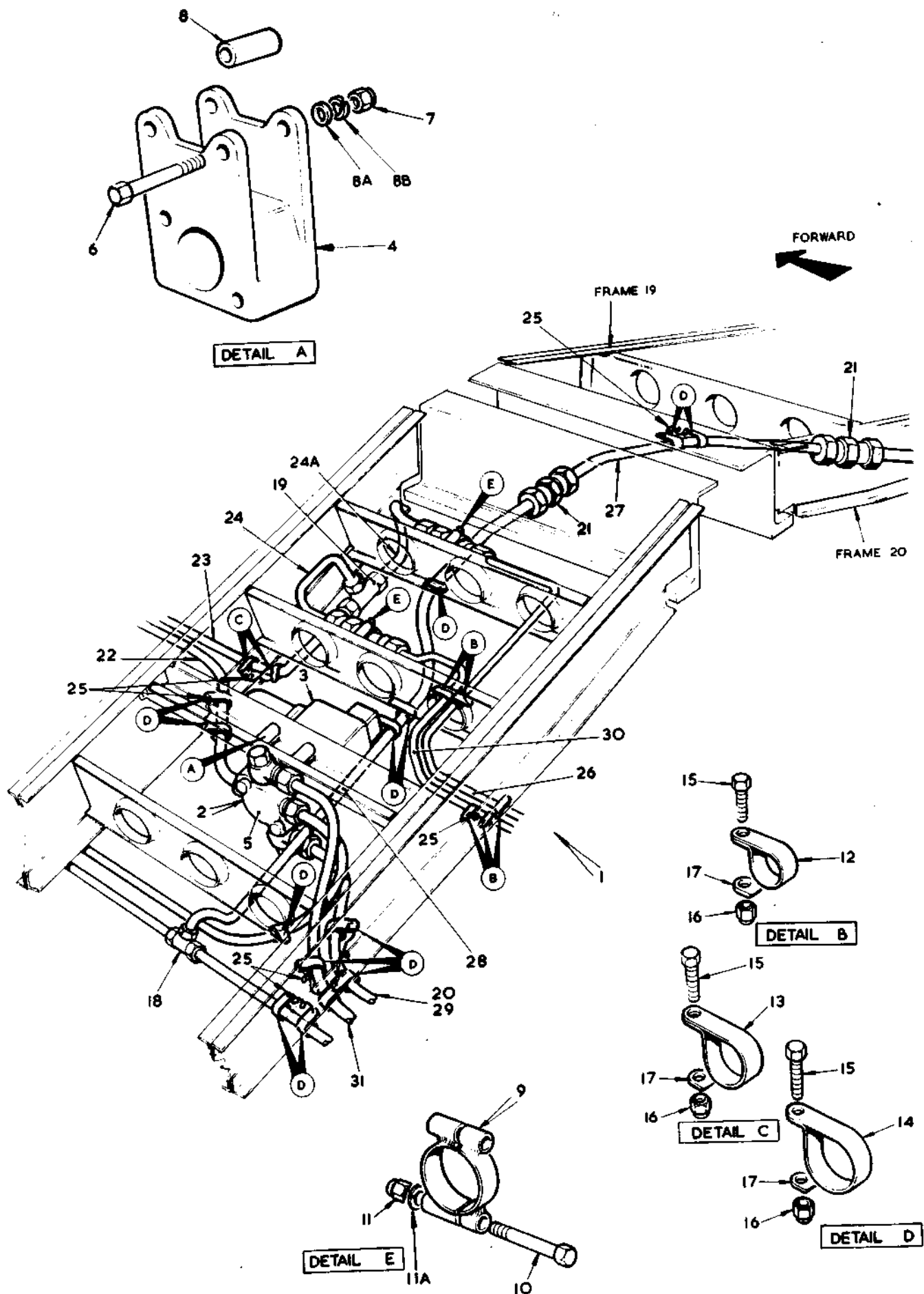
FIG 12 HYDRAULIC SYSTEM
