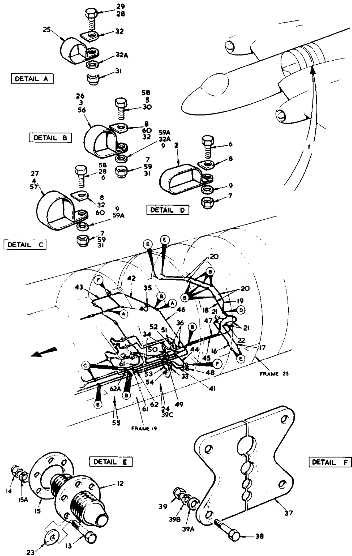
FIG.15 HYDRAULIC SYSTEM
