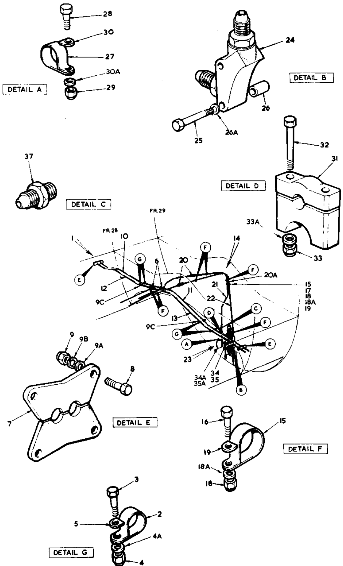
FIG. 13 HYDRAULIC SYSTEM
