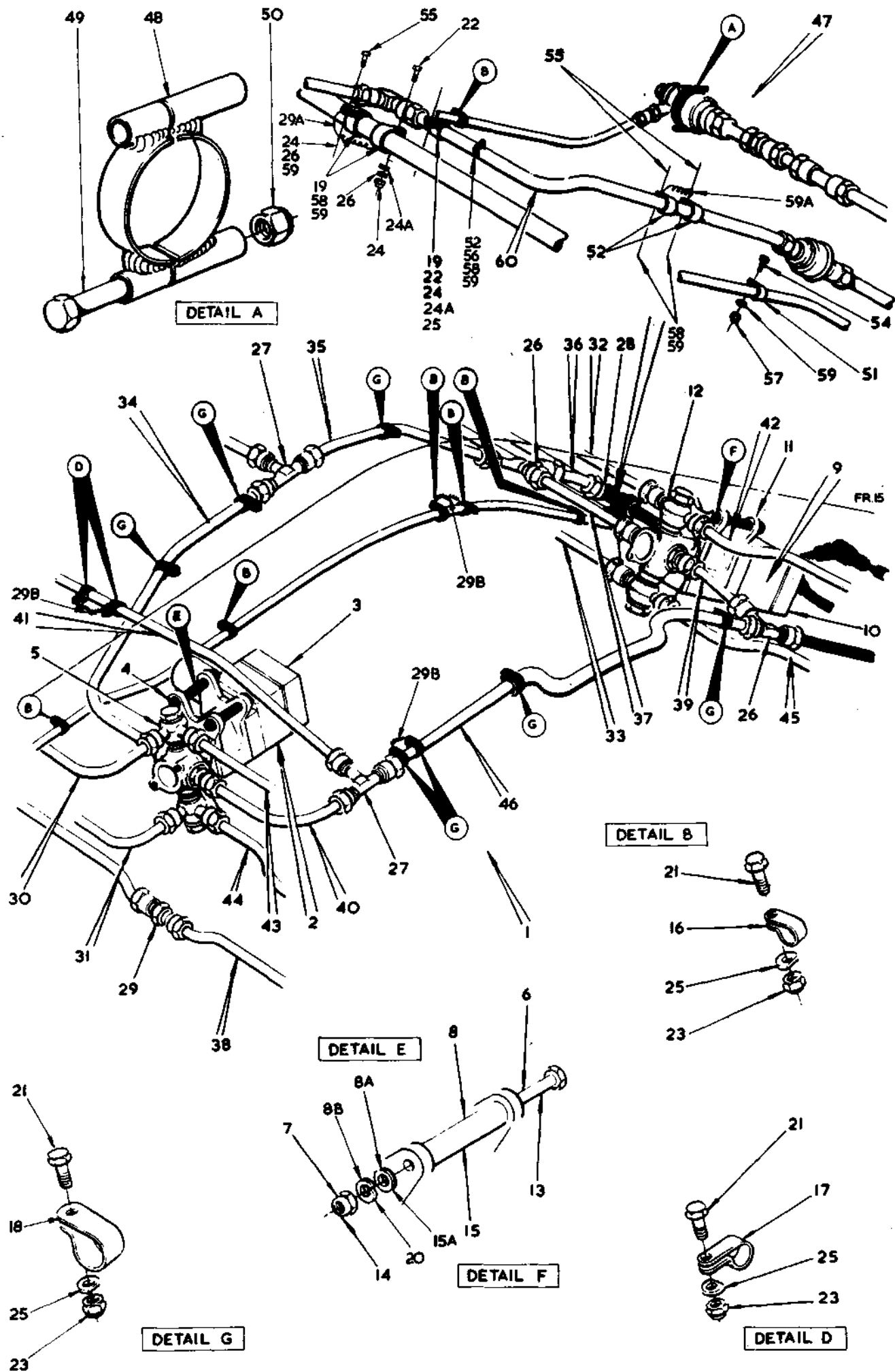
FIG 11 HYDRAULIC SYSTEM
