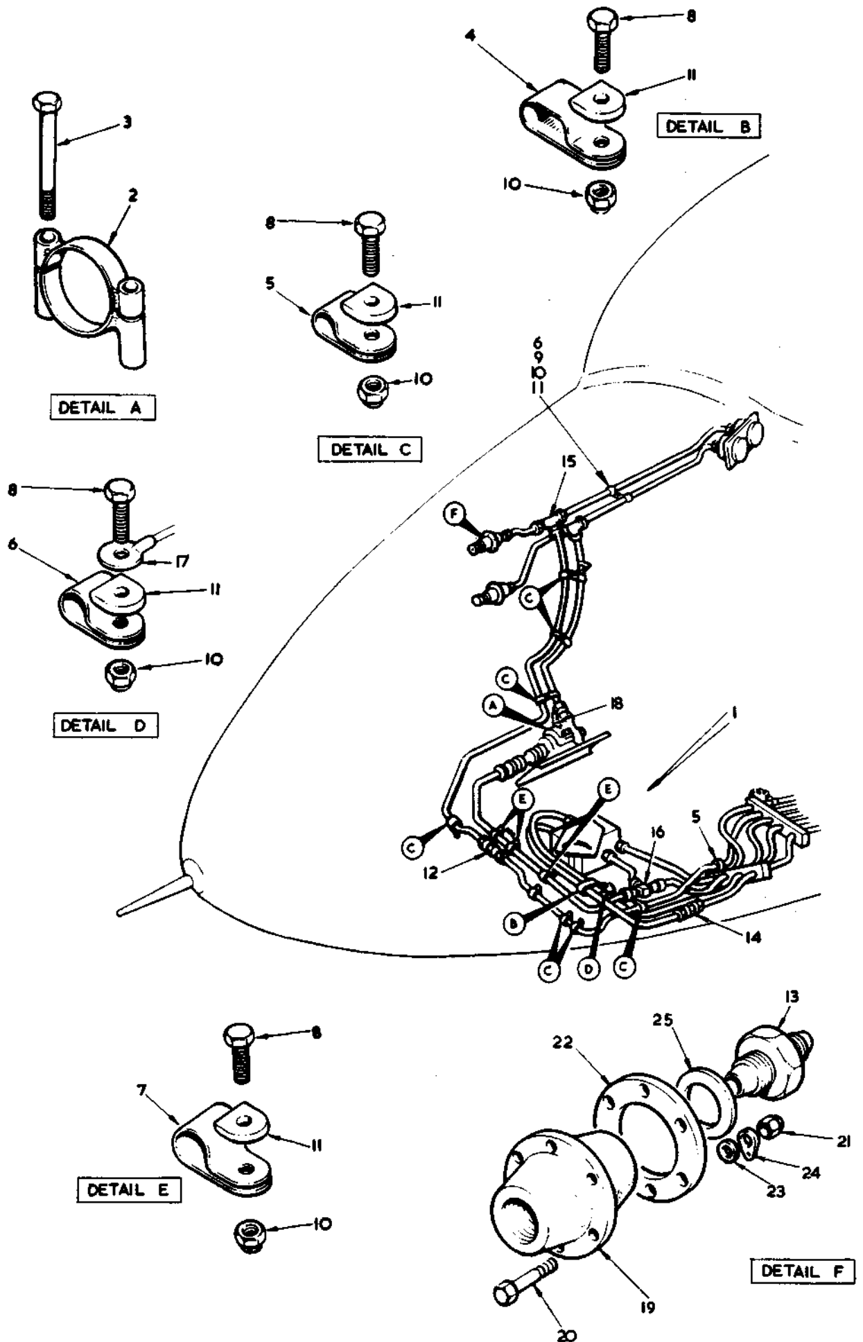
FIG. 2 HYDRAULIC SYSTEM
