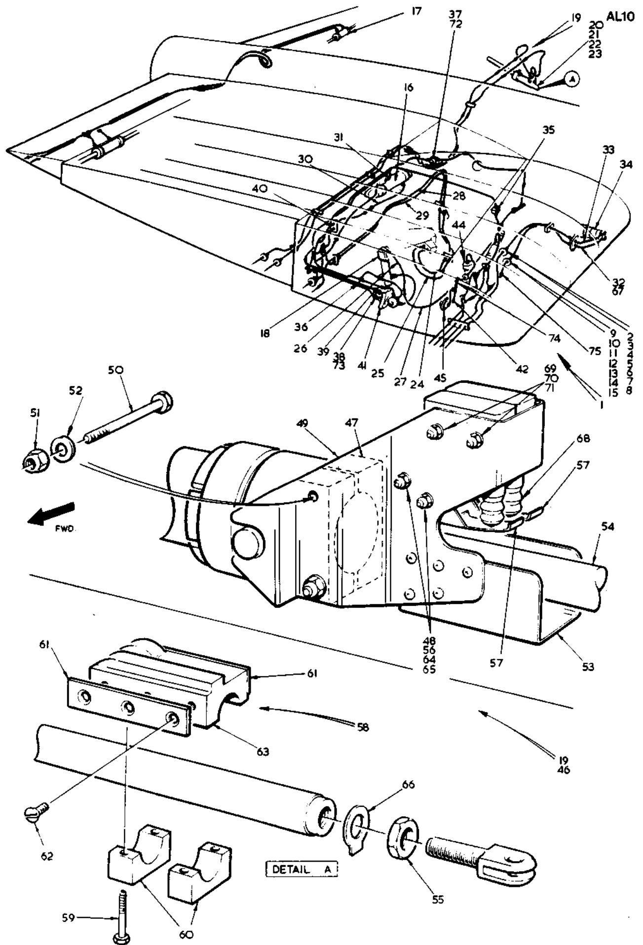
FIG. 20 HYDRAULIC SYSTEM
