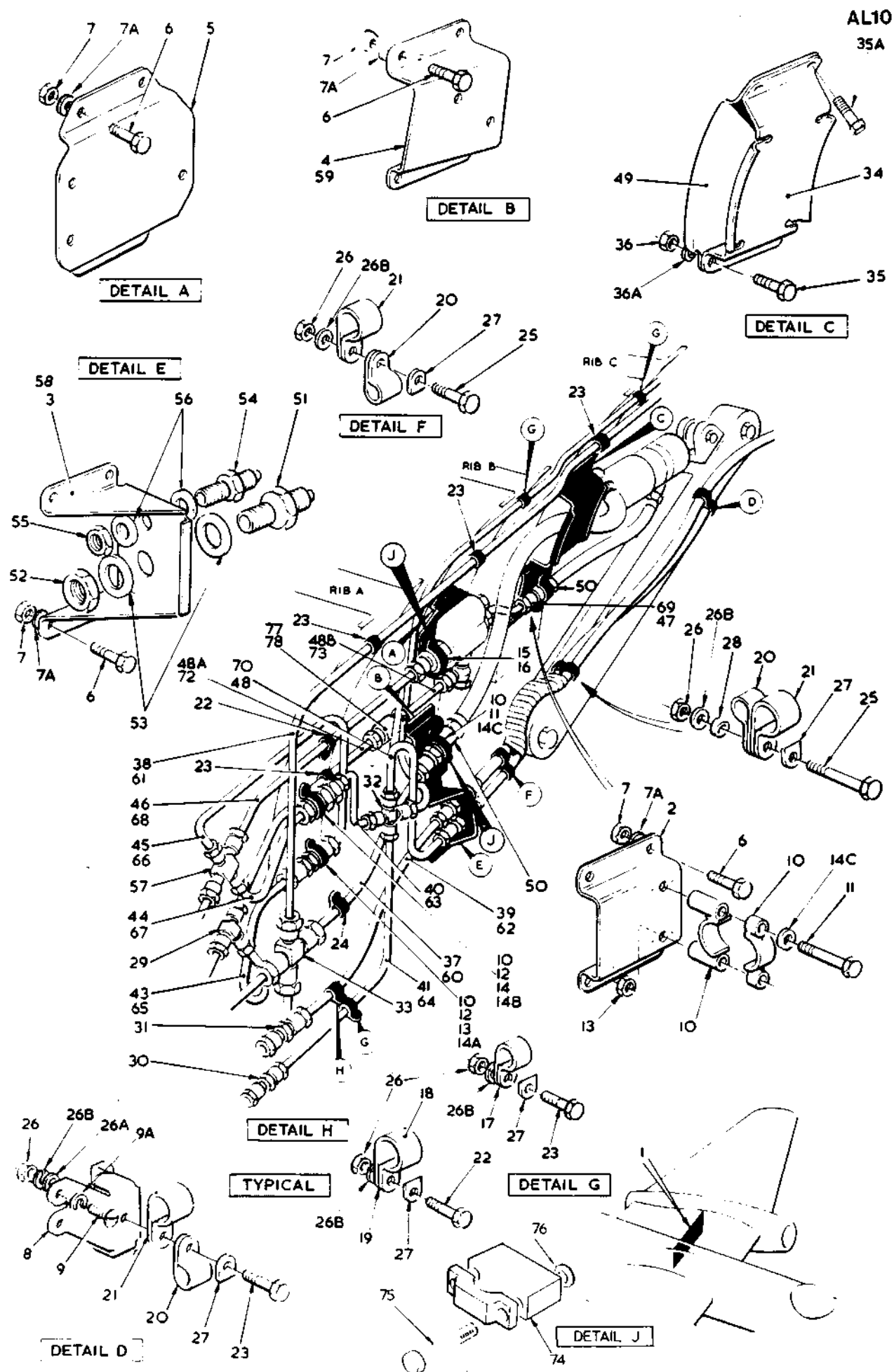
FIG 21 HYDRAULIC SYSTEM
