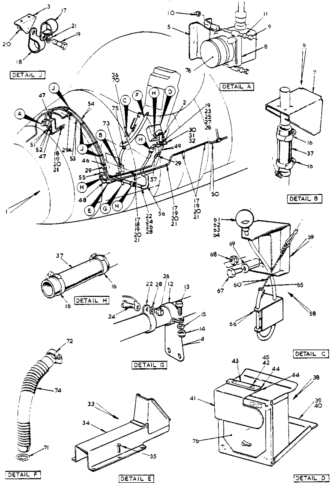
FIG. 4 OXYGEN SYSTEM
