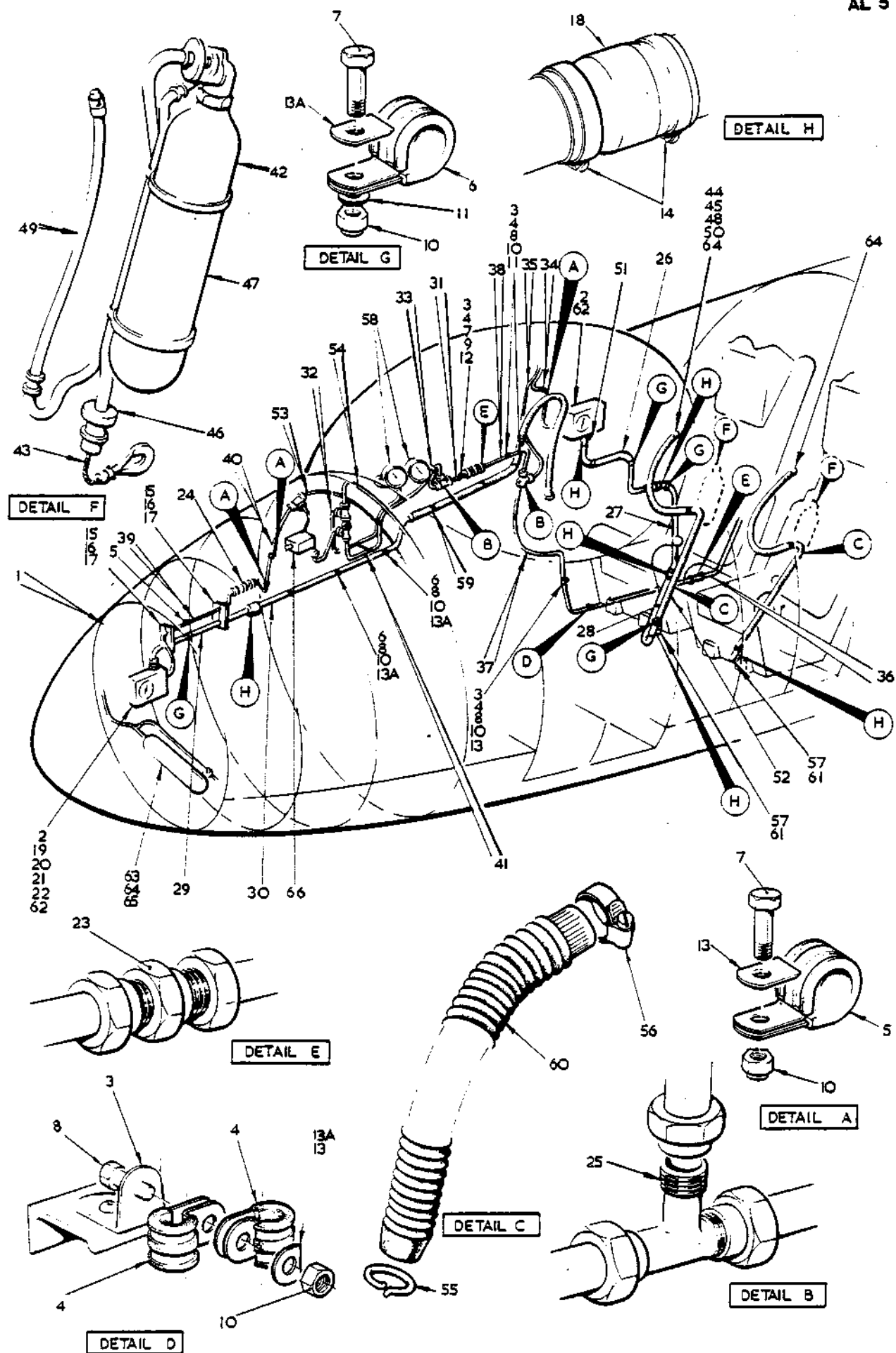
FIG.1 OXYGEN SYSTEM
