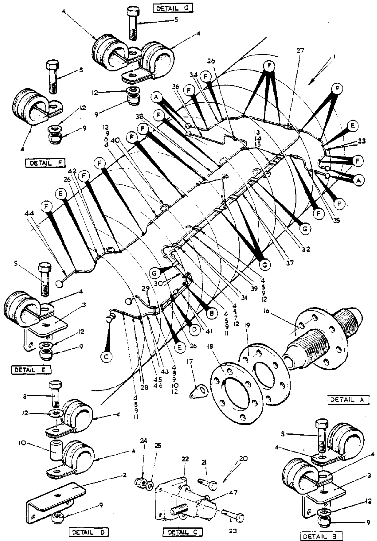
FIG. 5 OXYGEN SYSTEM
