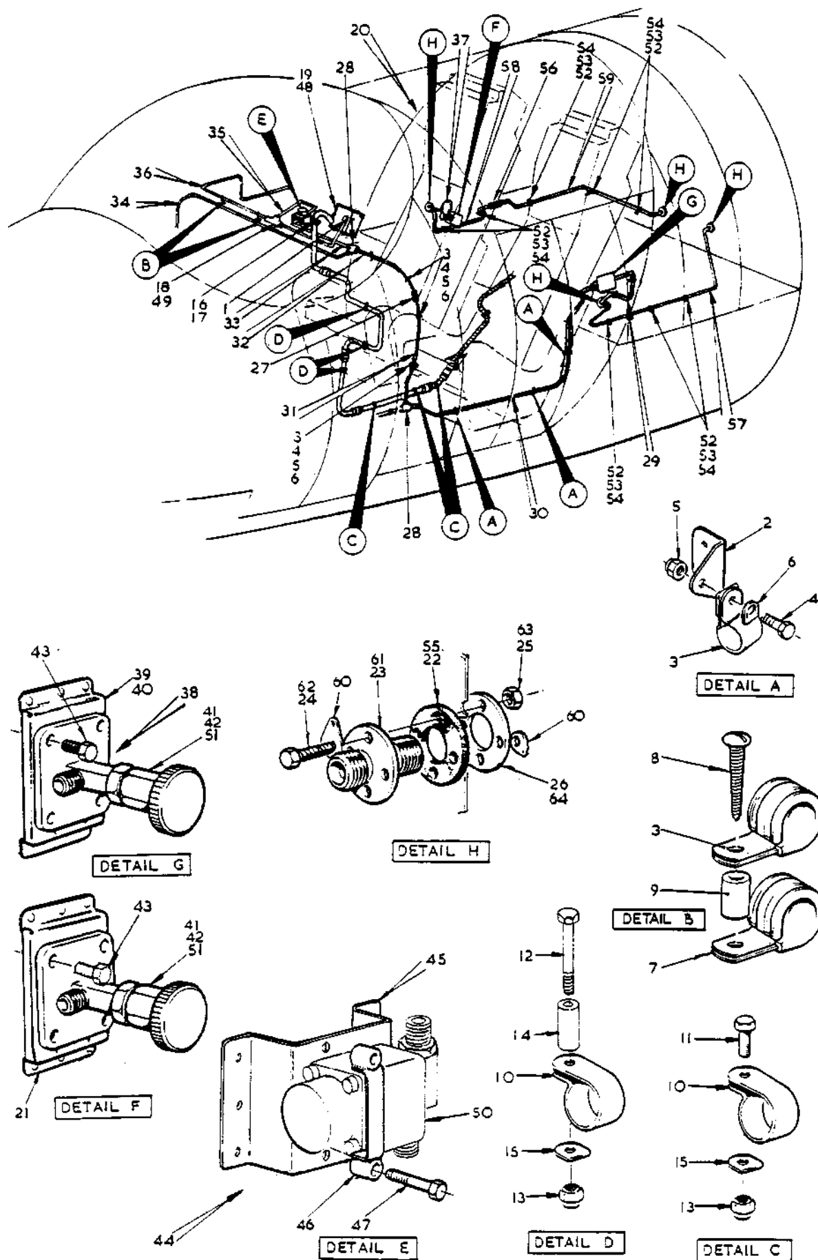
FIG. 3 OXYGEN SYSTEM
