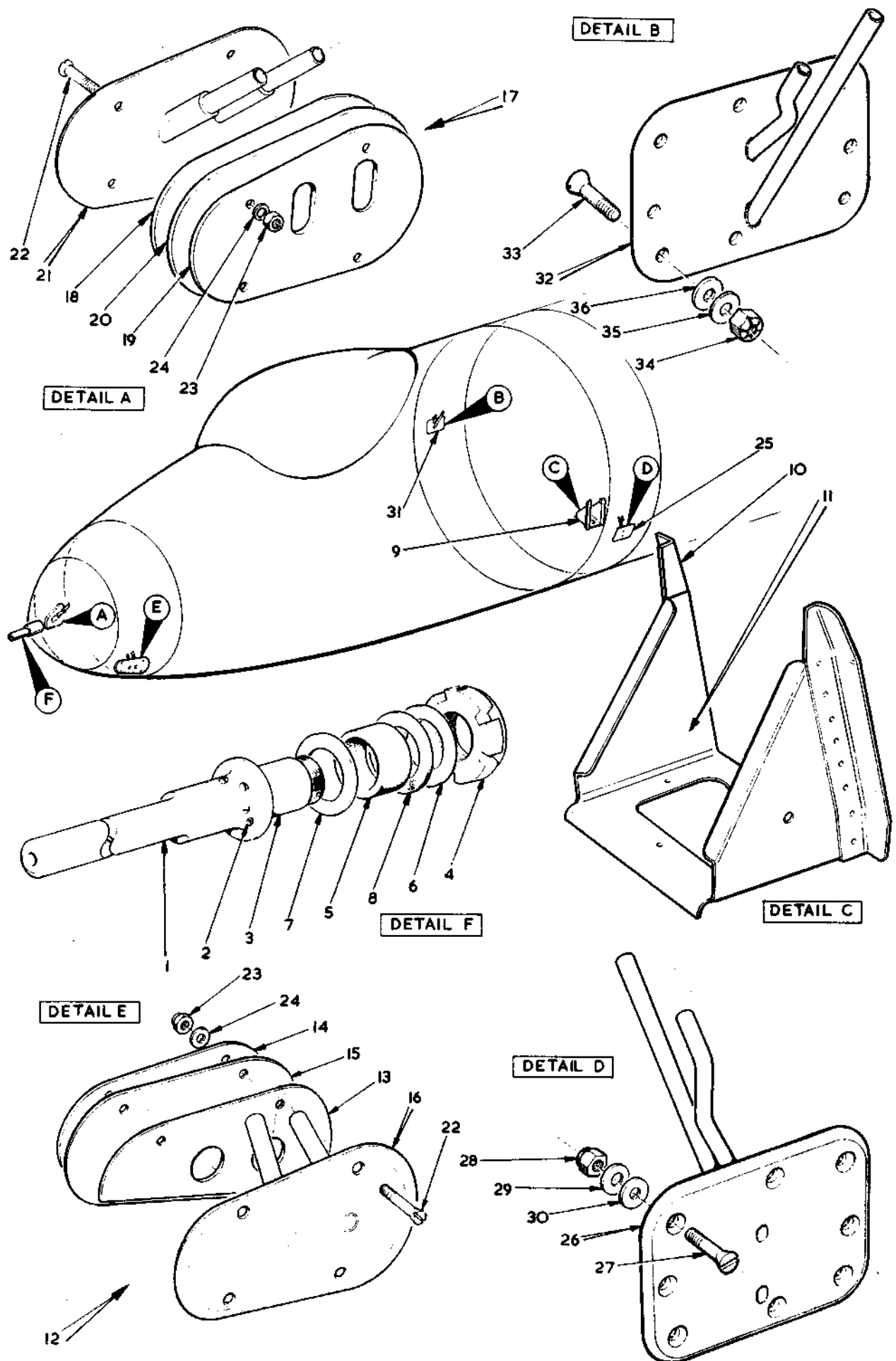
FIG. 1. PITOT AND STATIC SYSTEM
