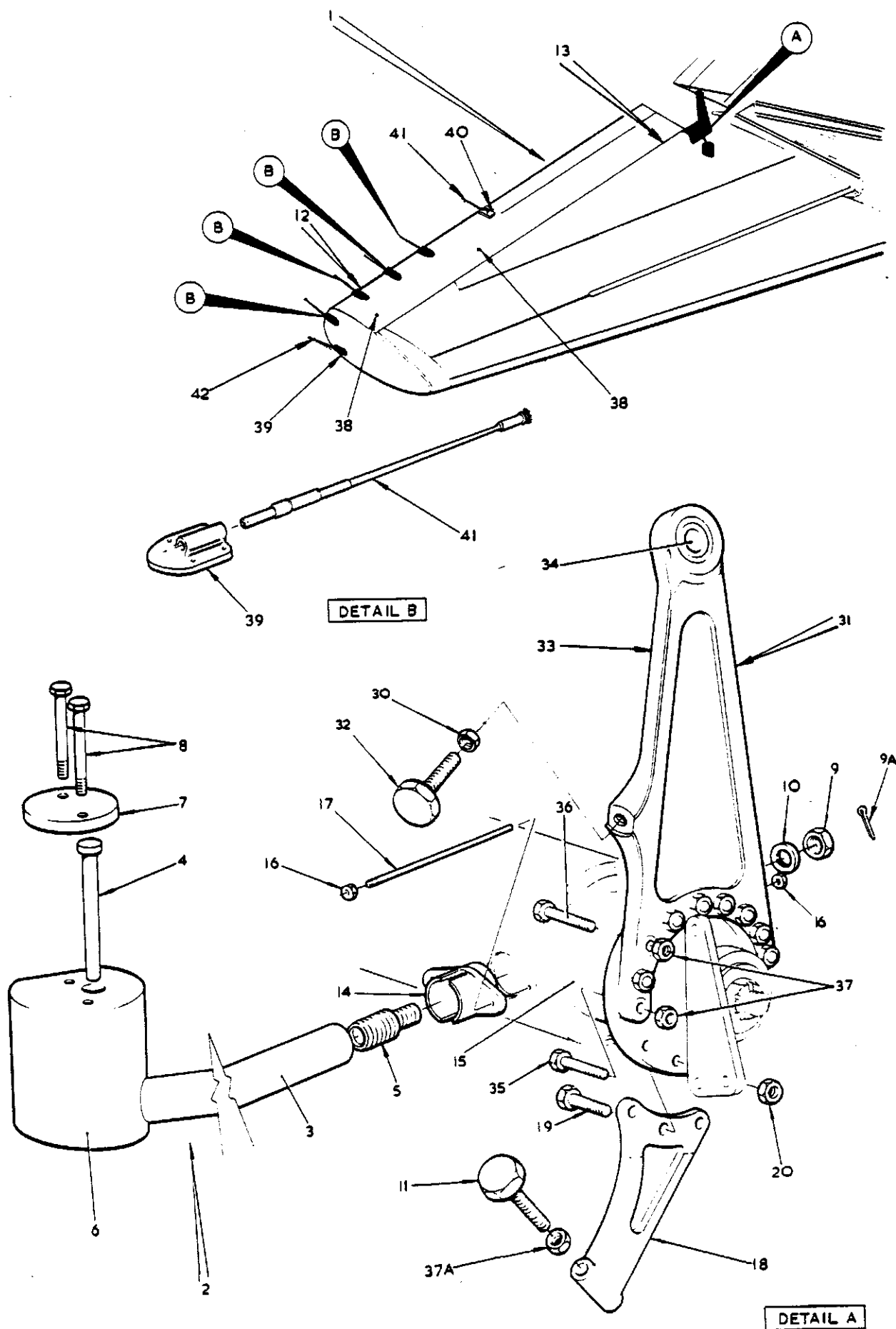
FIG. 2 TAIL UNIT
