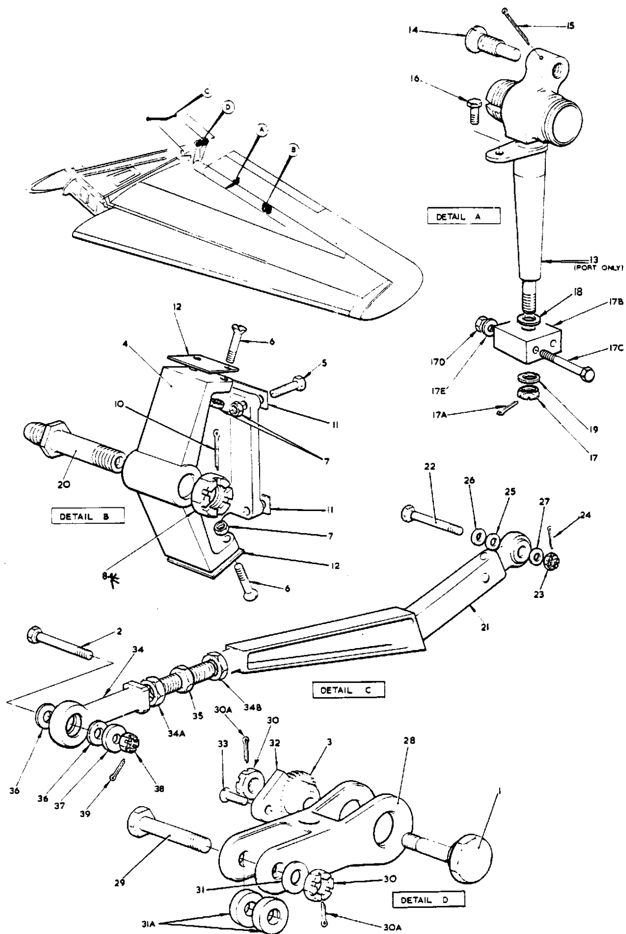
FIG 6 TAIL UNIT
