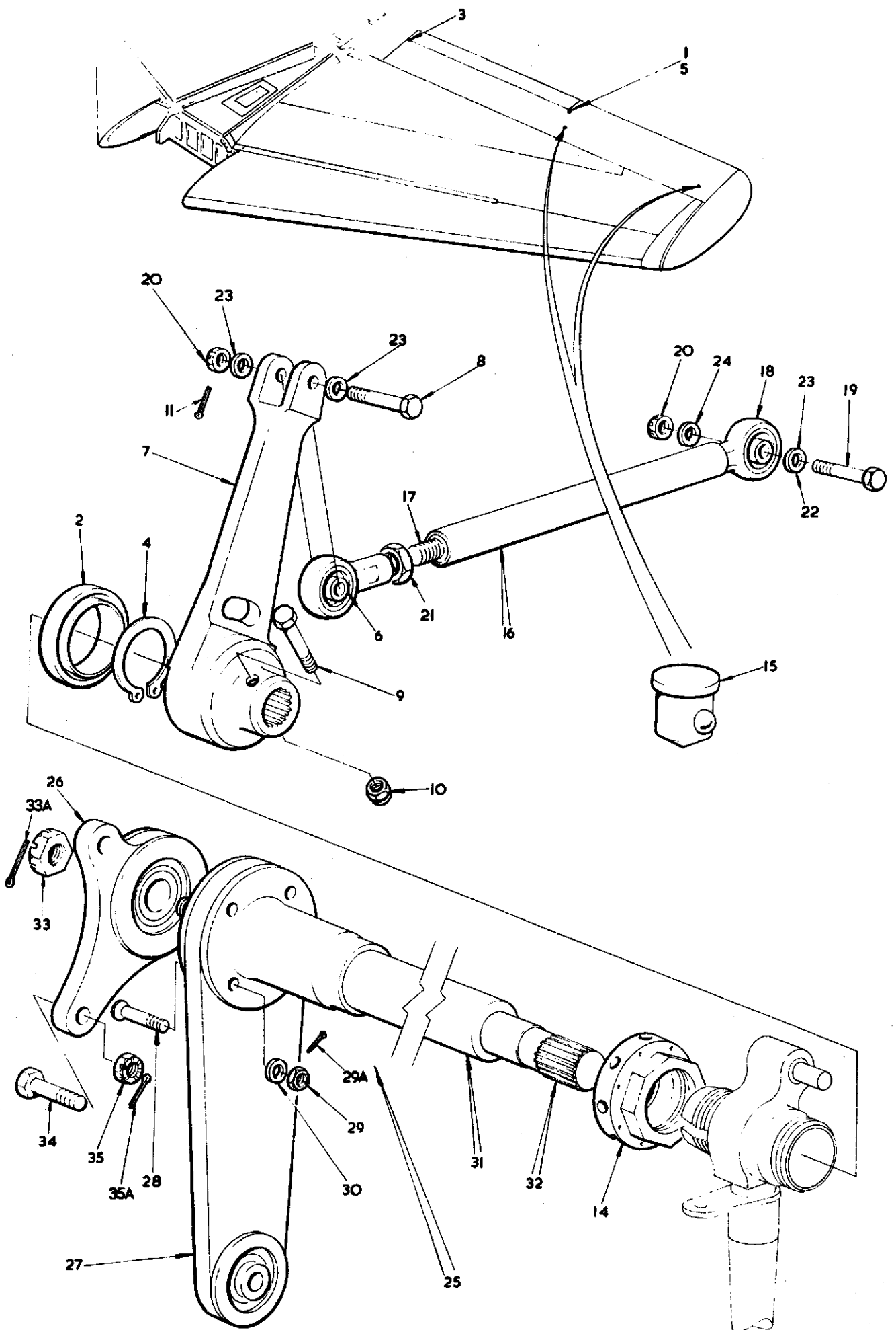
FIG.5 TAIL UNIT
