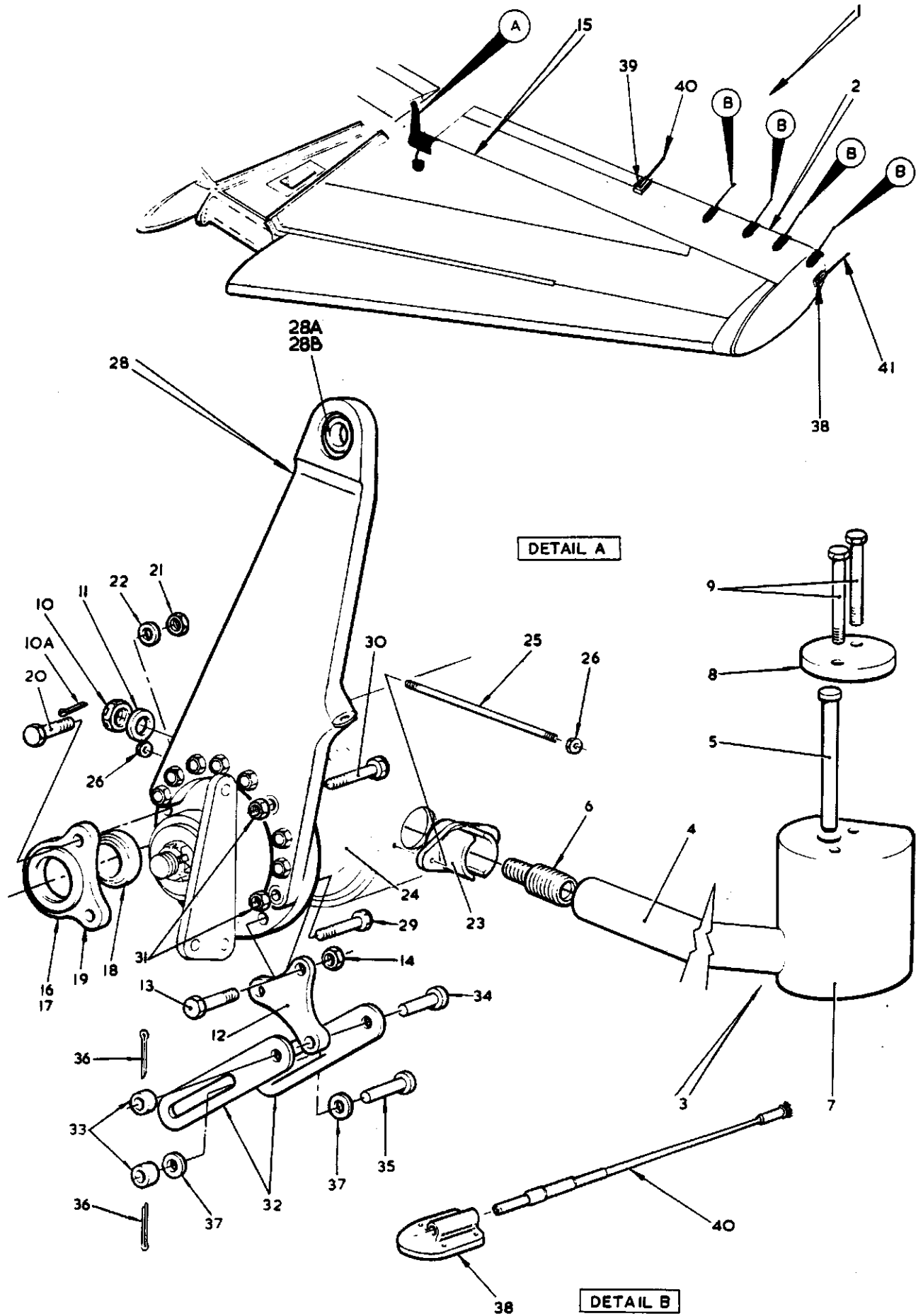
FIG.1 TAIL UNIT
