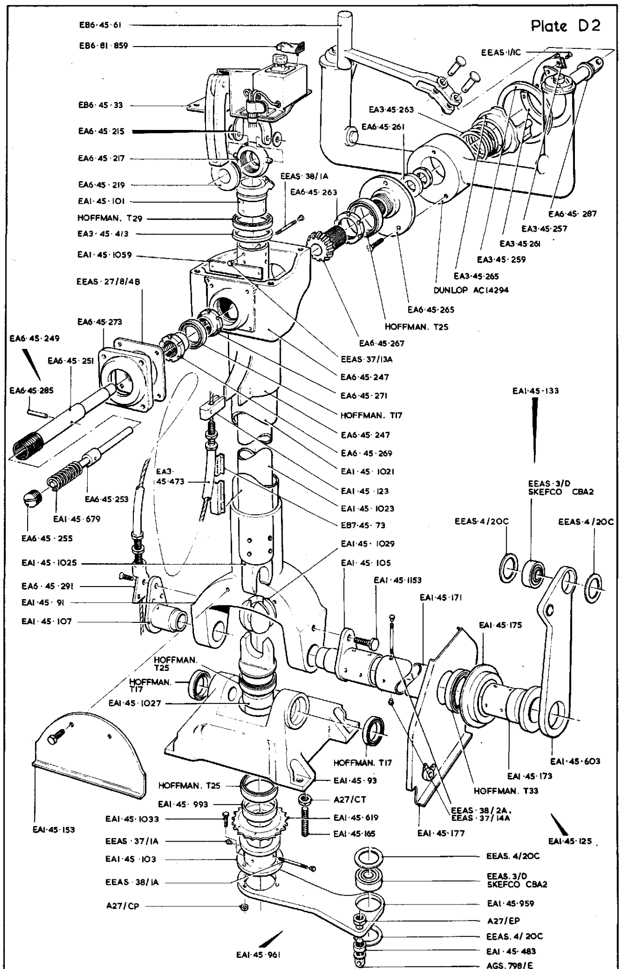
PILOTS CONTROL COLUMN
