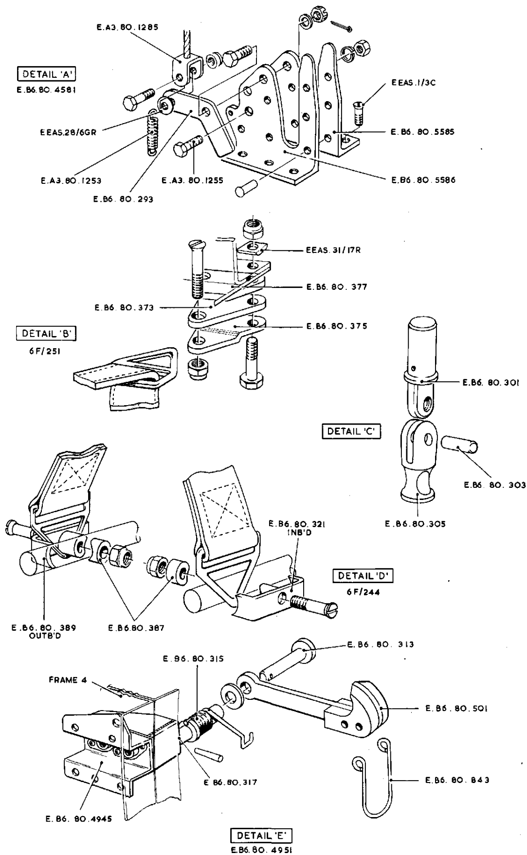
MAP READER'S SEAT - DETAIL
