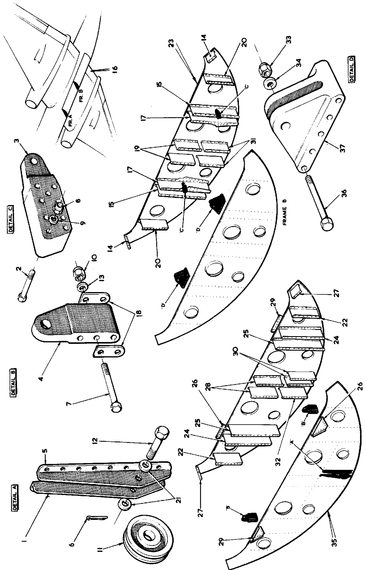
FIG.6 BOMB BAY PACK INSTALLATION Restricted
