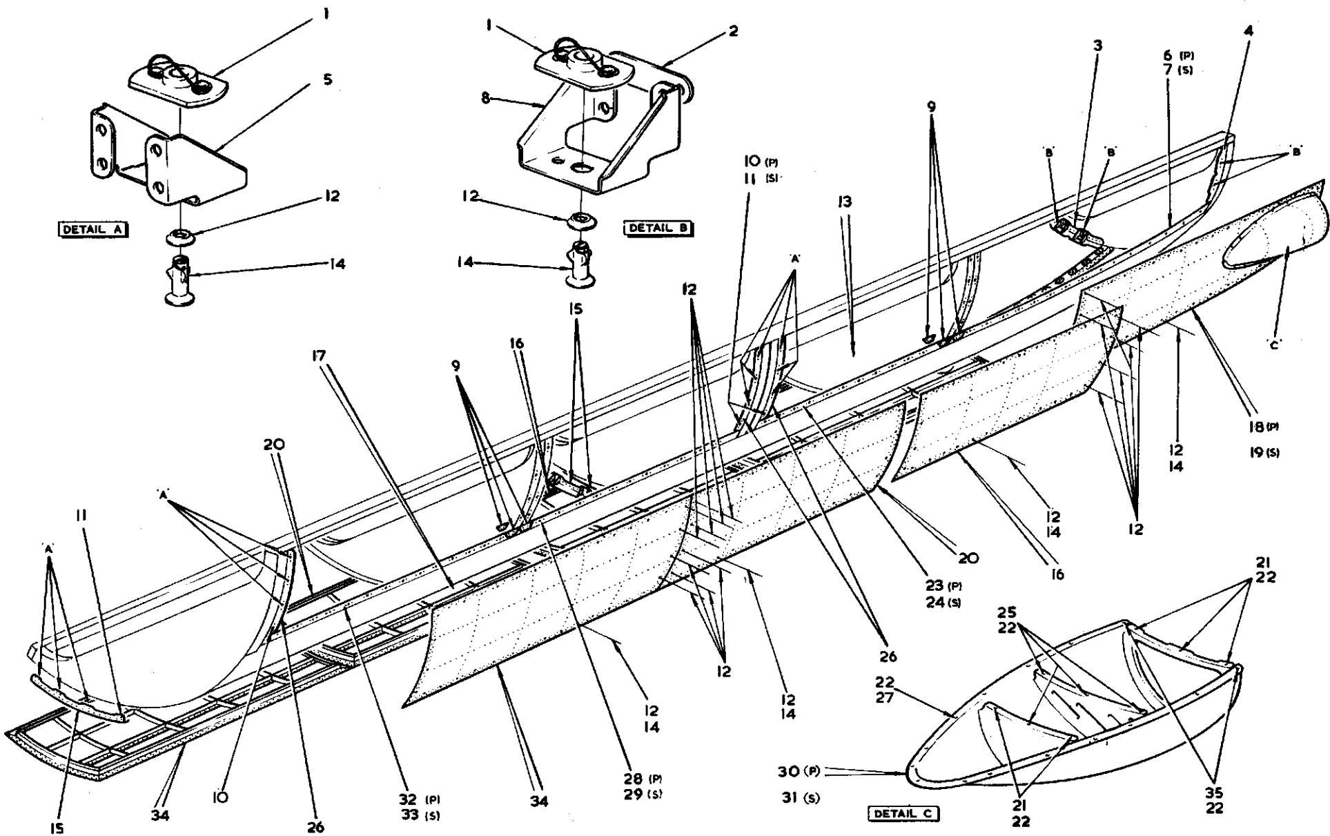
FIG. 10 BOMB BAY PACK INSTALLATION
