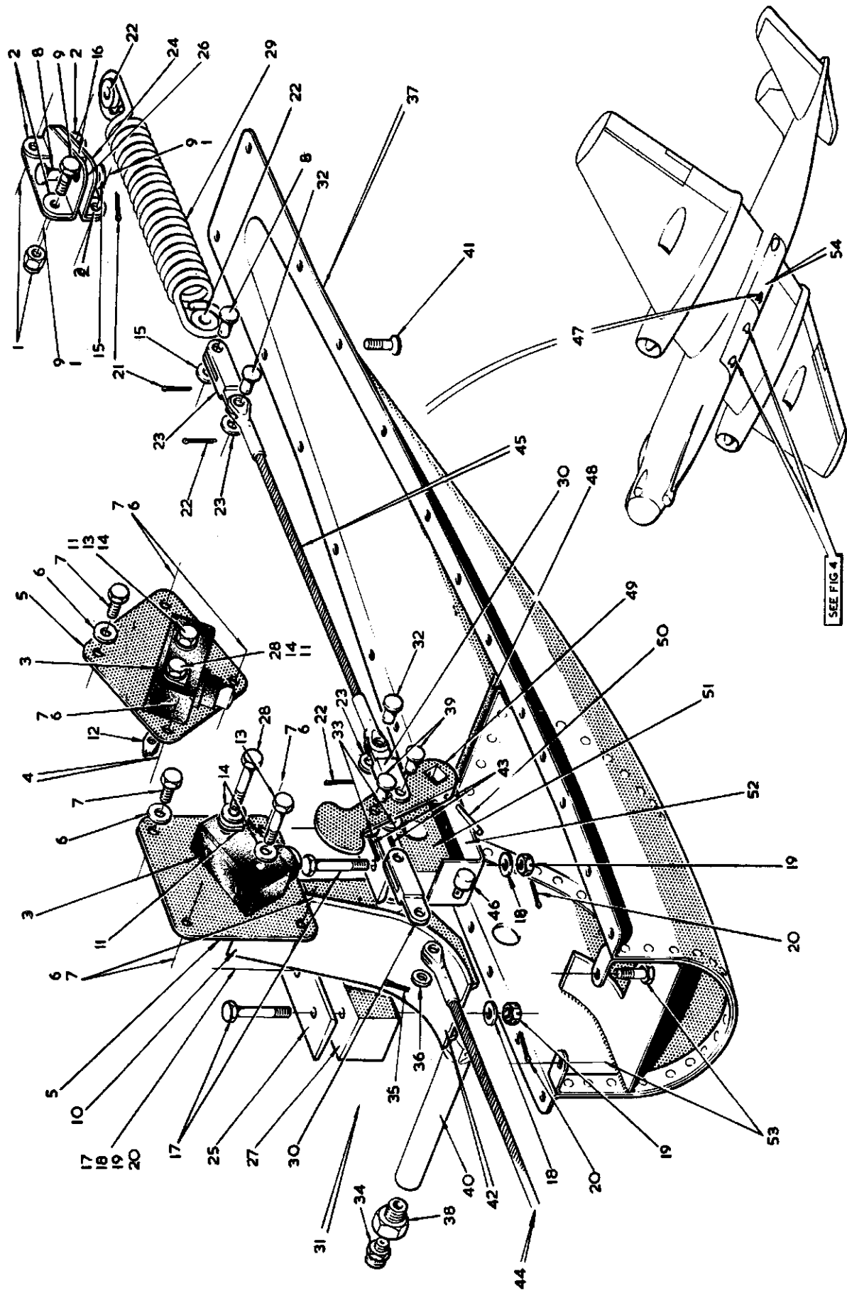
FIG.3 BOMB BAY PACK INSTALLATION Restricted
