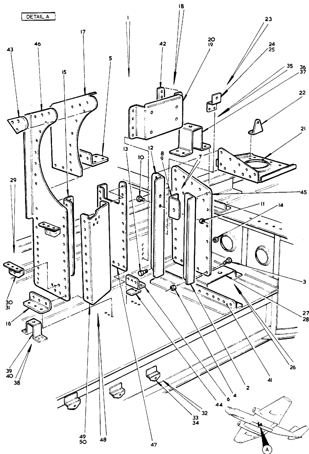
FIG.13. BOMB BAY PACK INSTALLATION
