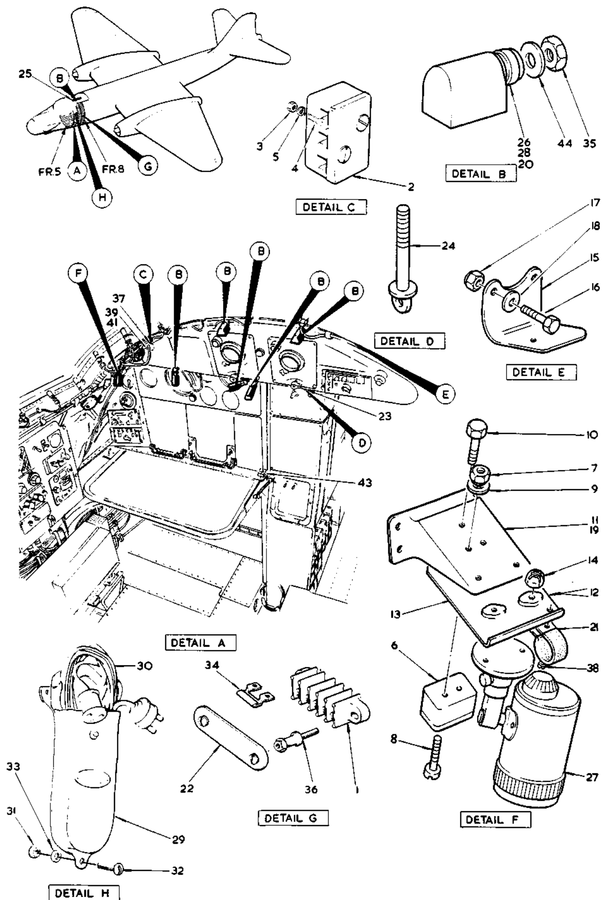
FIG. 54 ELECTRICAL EQUIPMENT IN FRONT FUSELAGE
