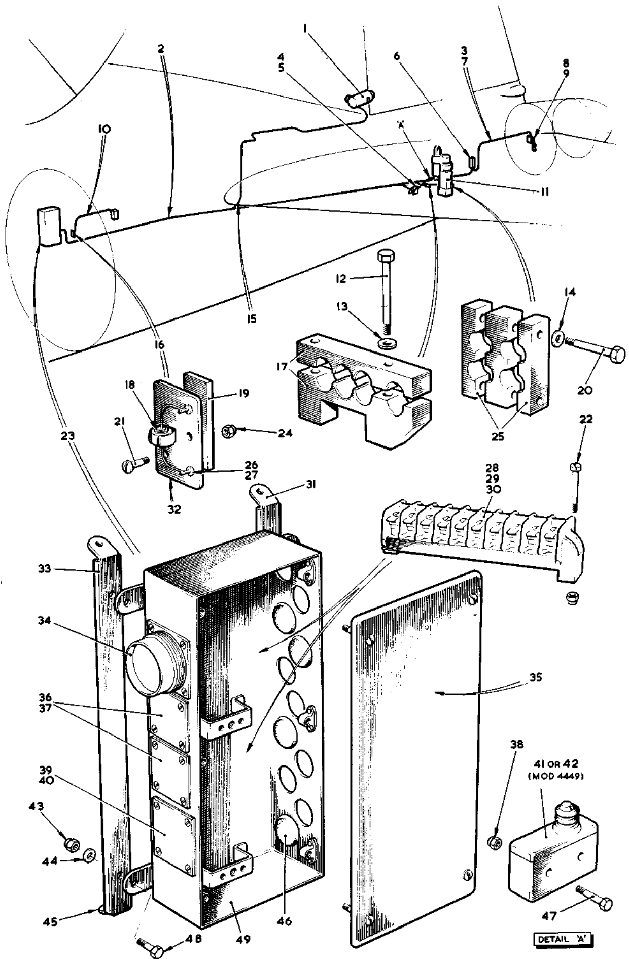
FIG. 43 ELECTRICAL EQUIPMENT IN REAR FUSELAGE Restricted
