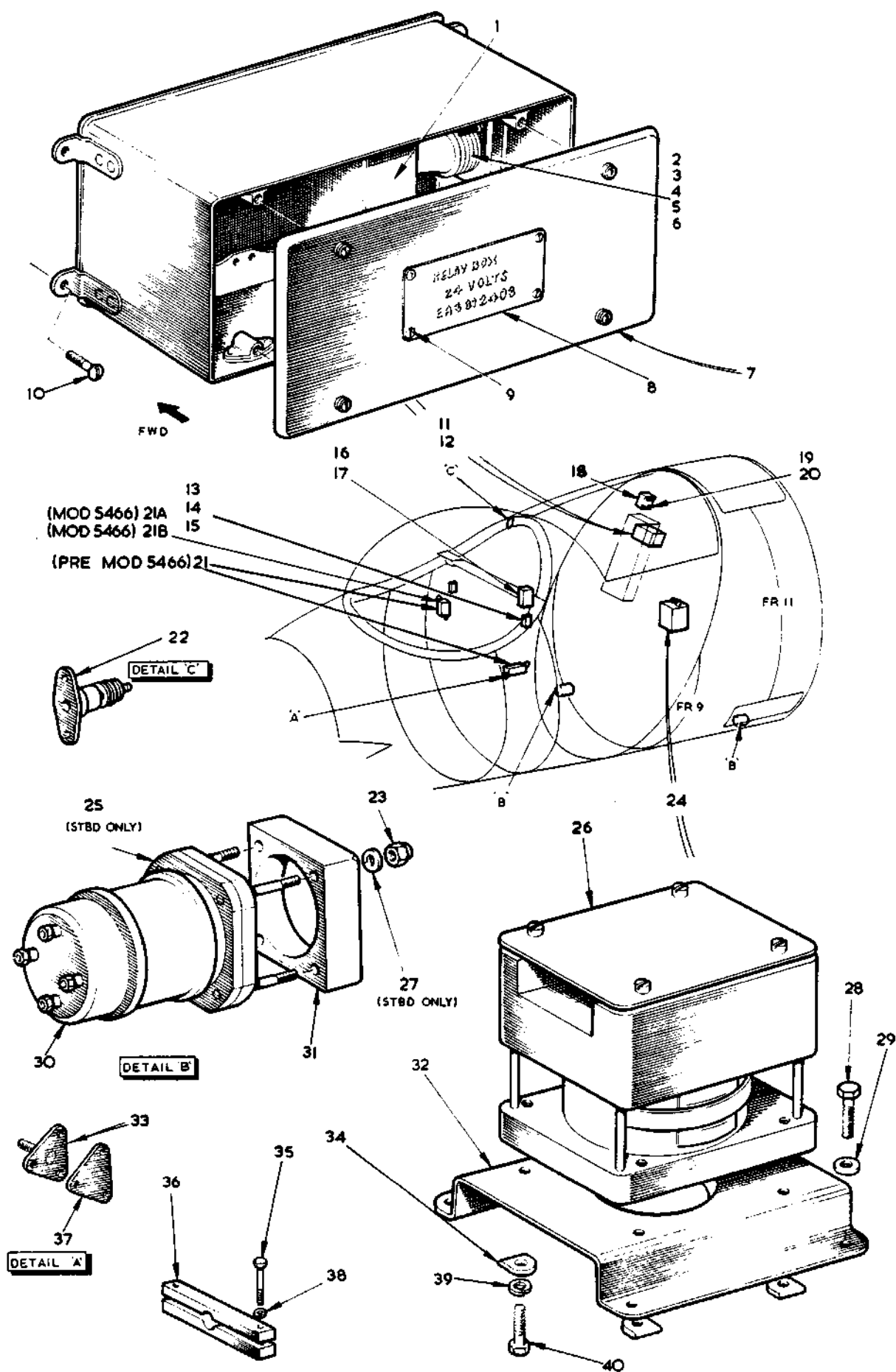
FIG.18 ELECTRICAL EQUIPMENT IN FRONT FUSELAGE
