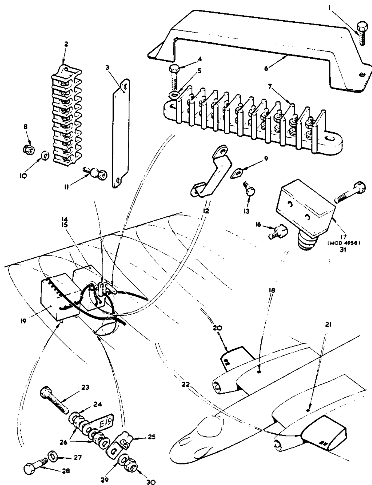
FIG.48 ELECTRICAL EQUIPMENT IN PORT & STARBOARD WINGS
