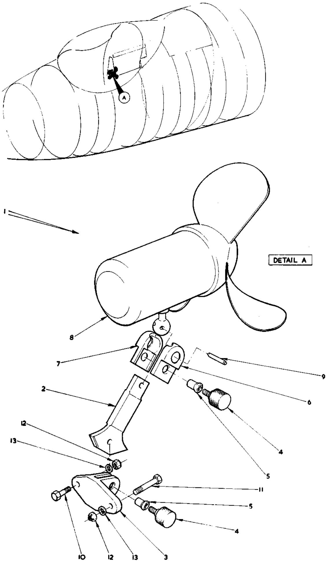
FIG. 10A PRESSURE CABIN EQUIPMENT
