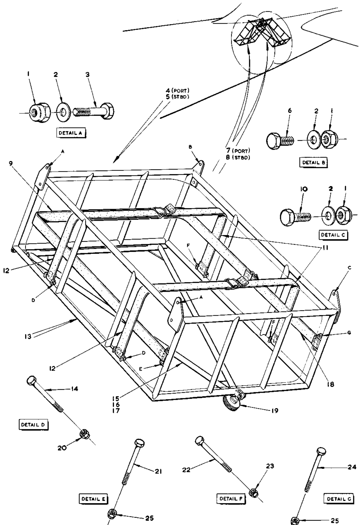
FIG.26 EQUIPMENT IN REAR FUSELAGE Restricted
