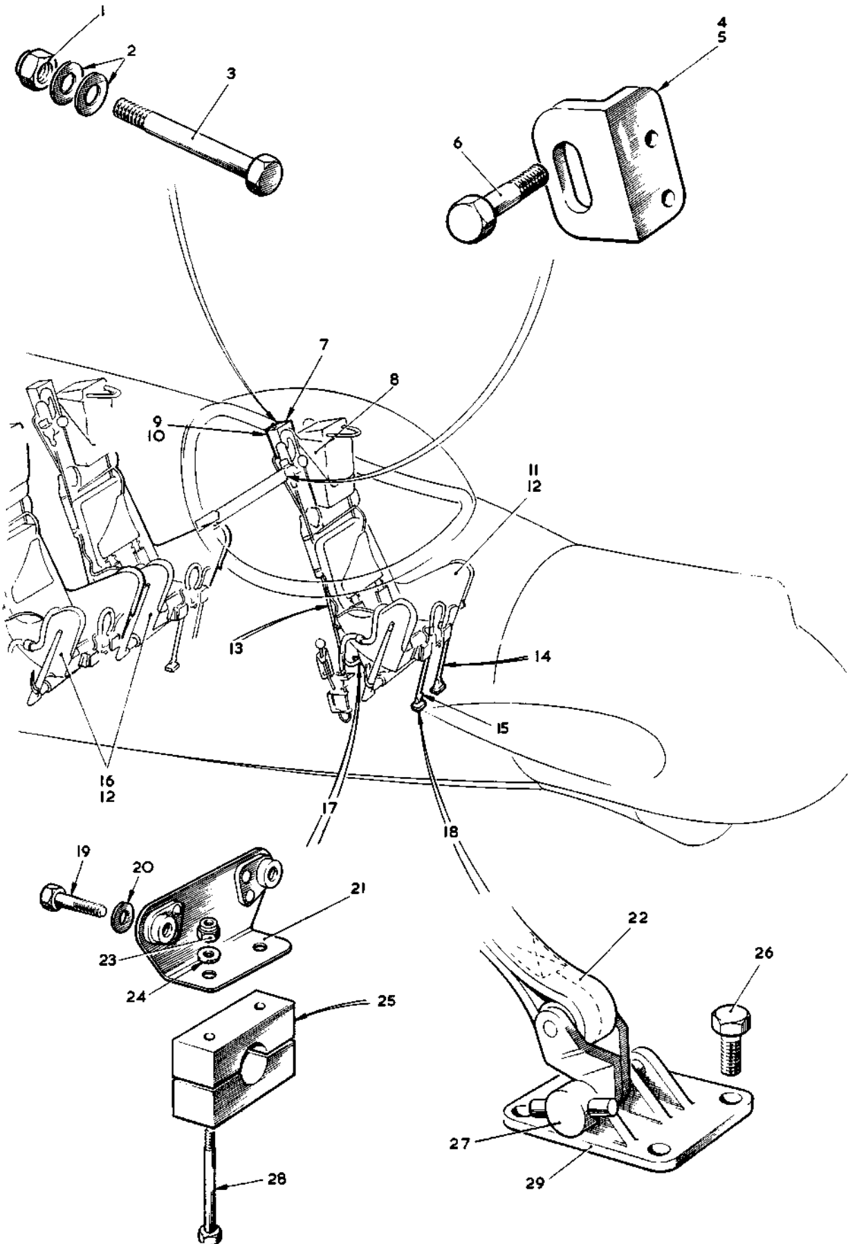
FIG.20 PRESSURE CABIN EQUIPMENT Restricted
