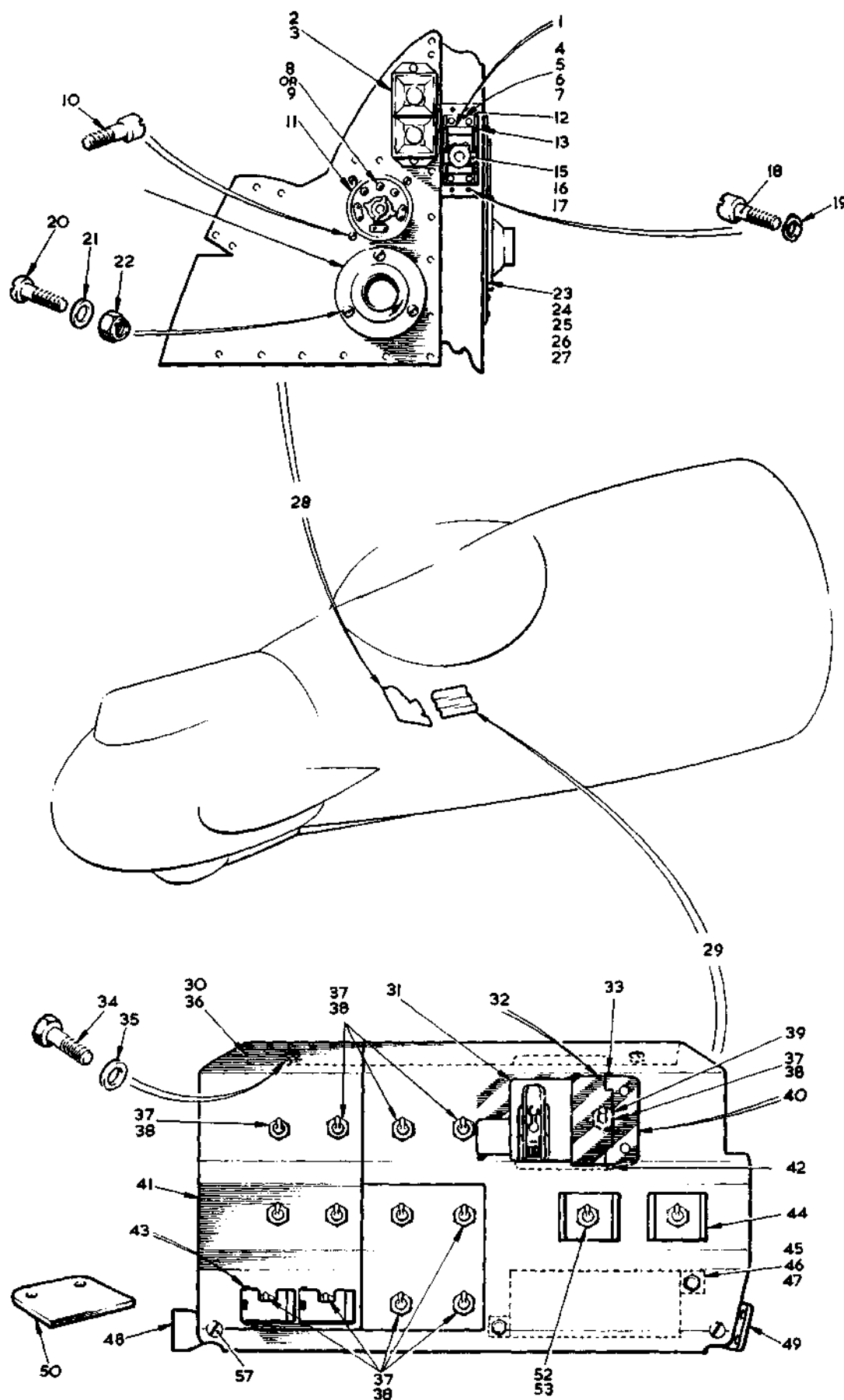
FIG.19 PRESSURE CABIN EQUIPMENT Restricted
