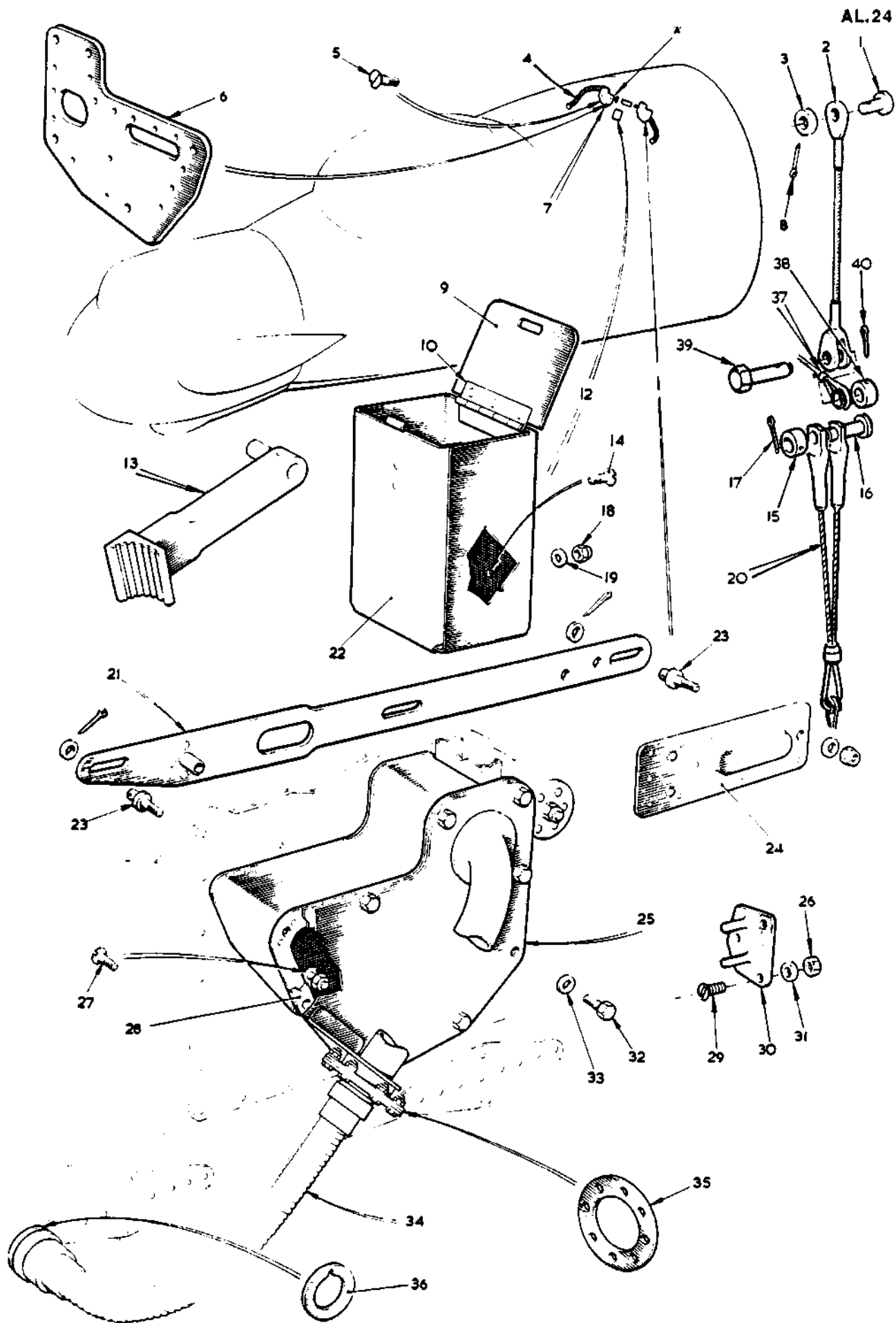
FIG.21 PRESSURE CABIN EQUIPMENT
