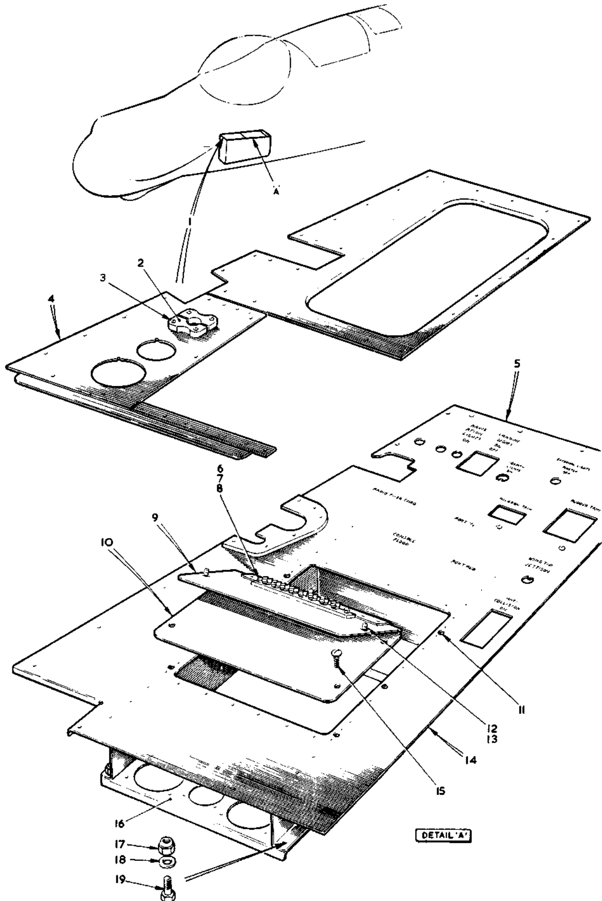
FIG 3 PRESSURE CABIN EQUIPMENT Restricted
