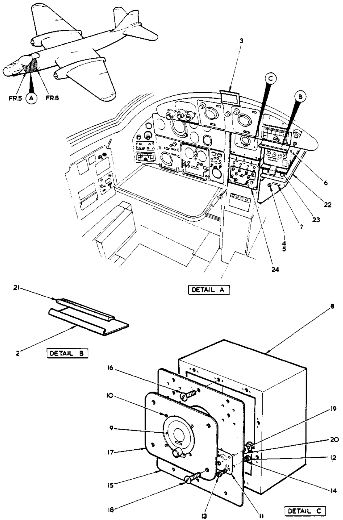
FIG 5A PRESSURE CABIN EQUIPMENT
