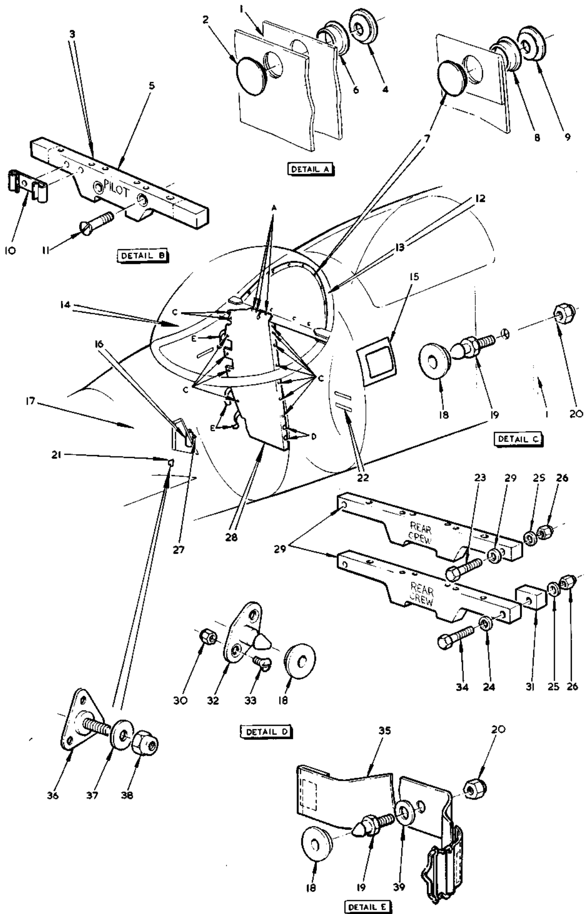
FIG. 1. PRESSURE CABIN EQUIPMENT Restricted
