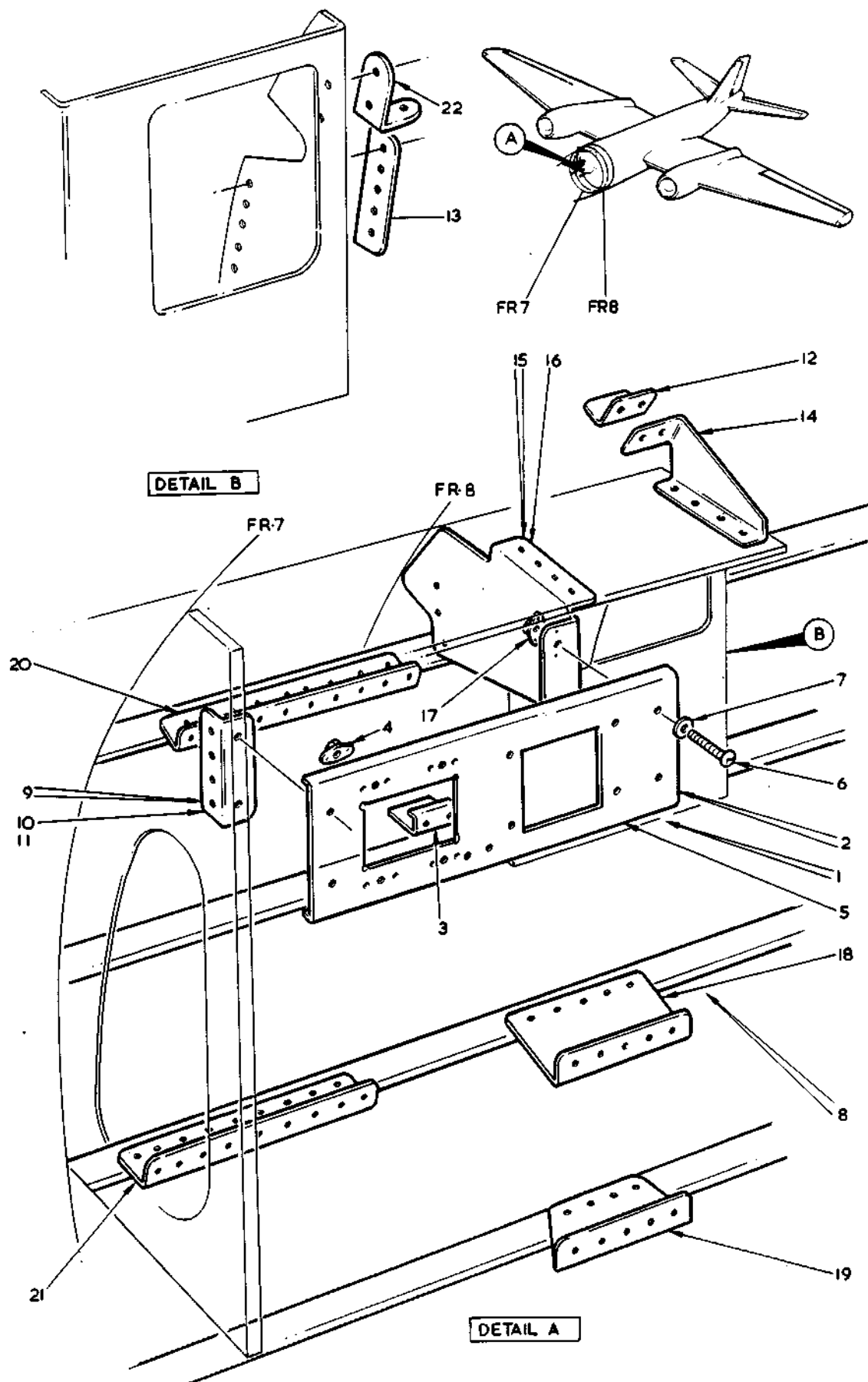
FIG 37 PRESSURE CABIN EQUIPMENT
