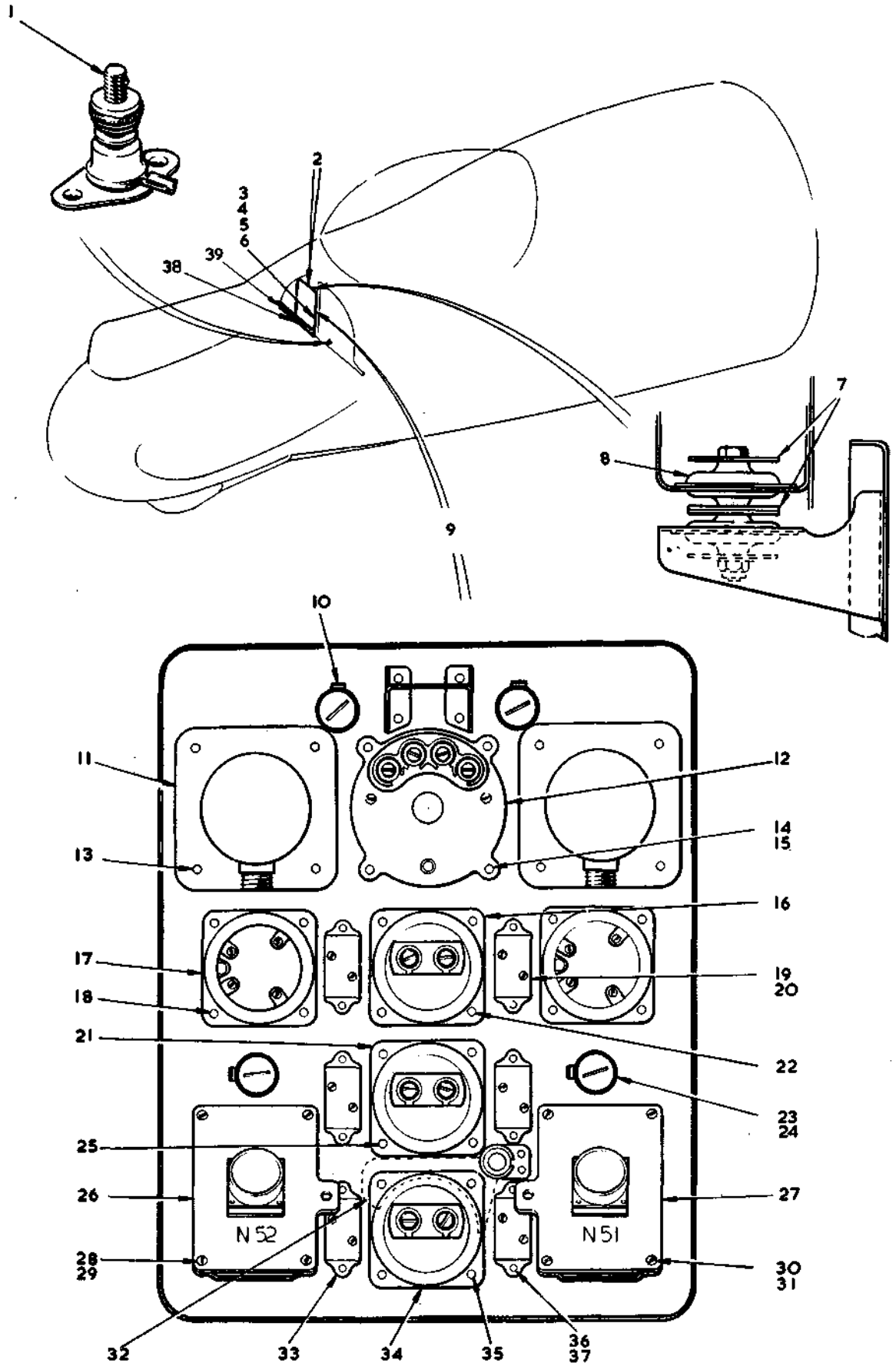
FIG. 17 PRESSURE CABIN EQUIPMENT Restricted
