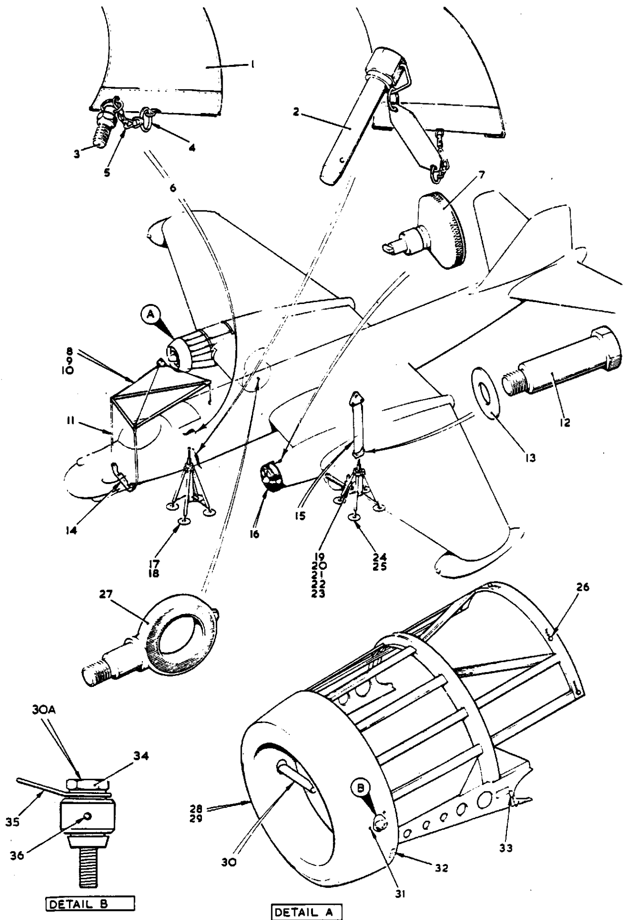
FIG.4 GROUND EQUIPMENT
