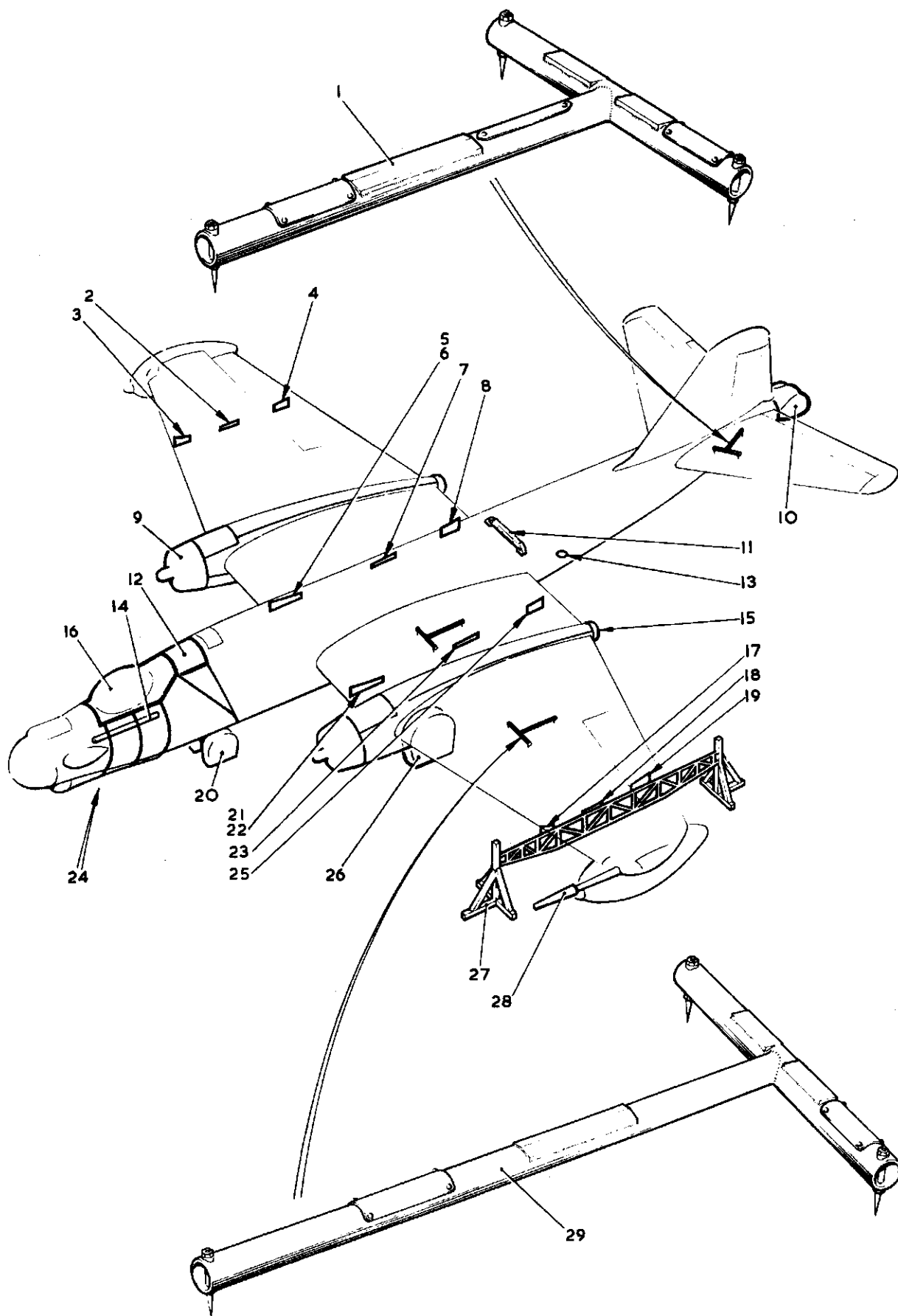
FIG3. GROUND EQUIPMENT Restricted
