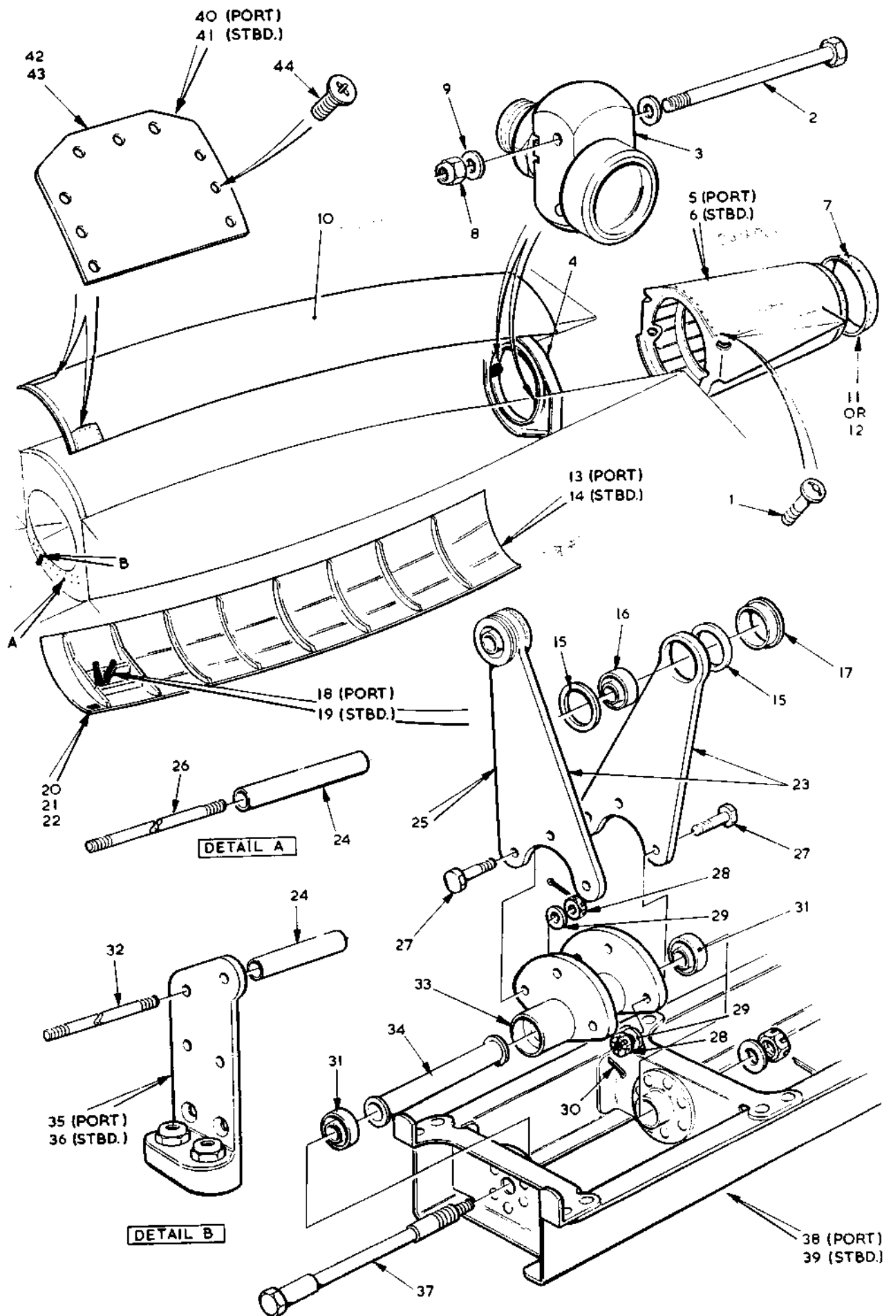
FIG. 12 WING STRUCTURE PORT AND STARBOARD Restricted
