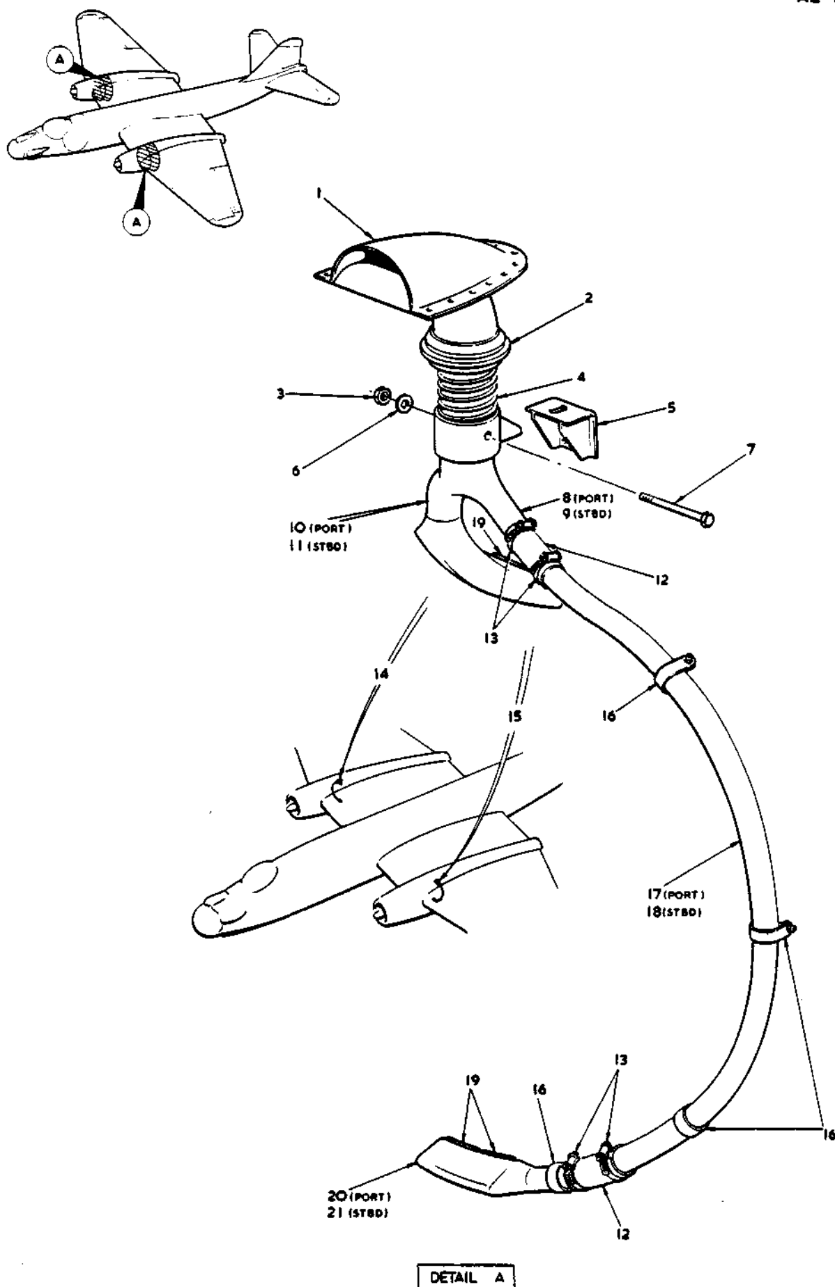
FIG 27 MAIN SPAR COOLING PORT &amp; STARBOARD
