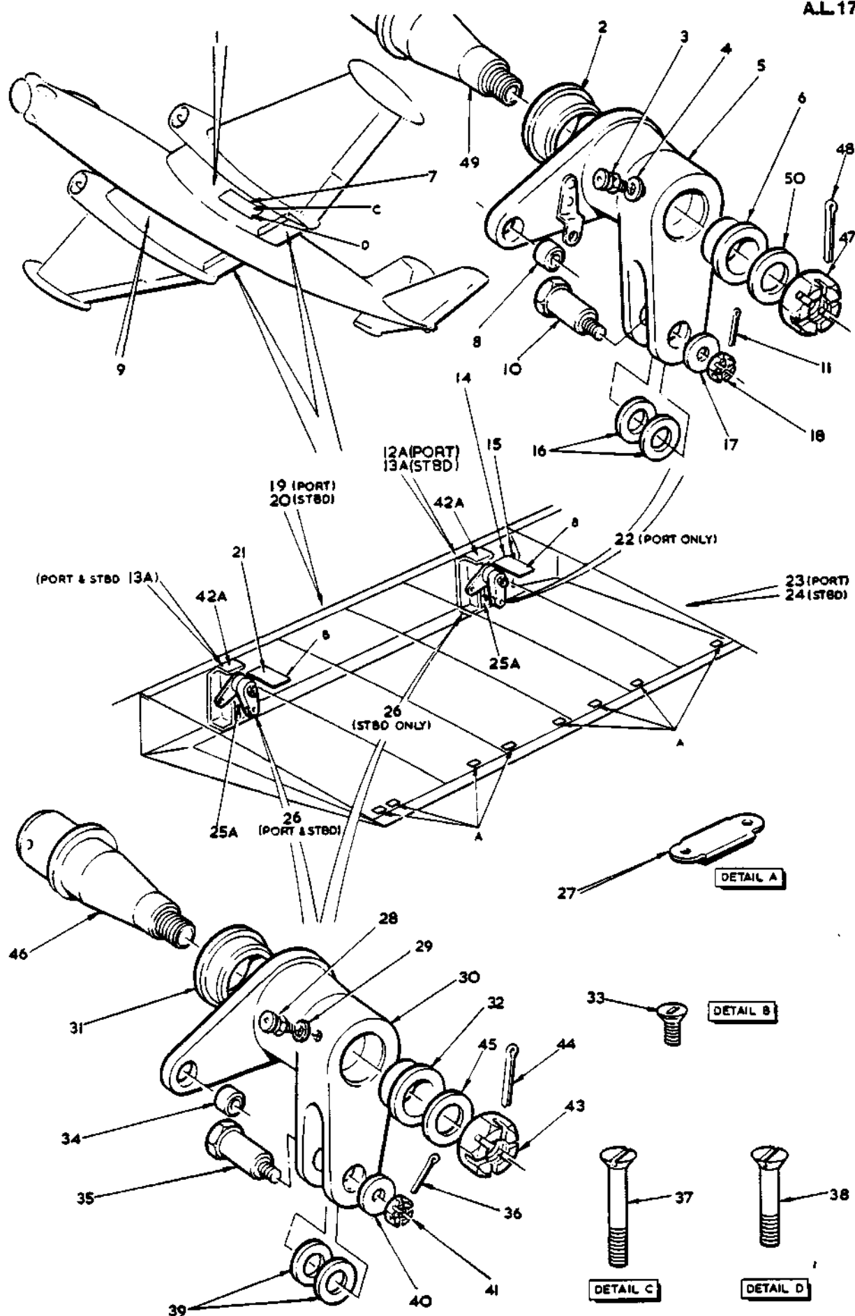
FIG 15 WING STRUCTURE PORT &amp; STBD
