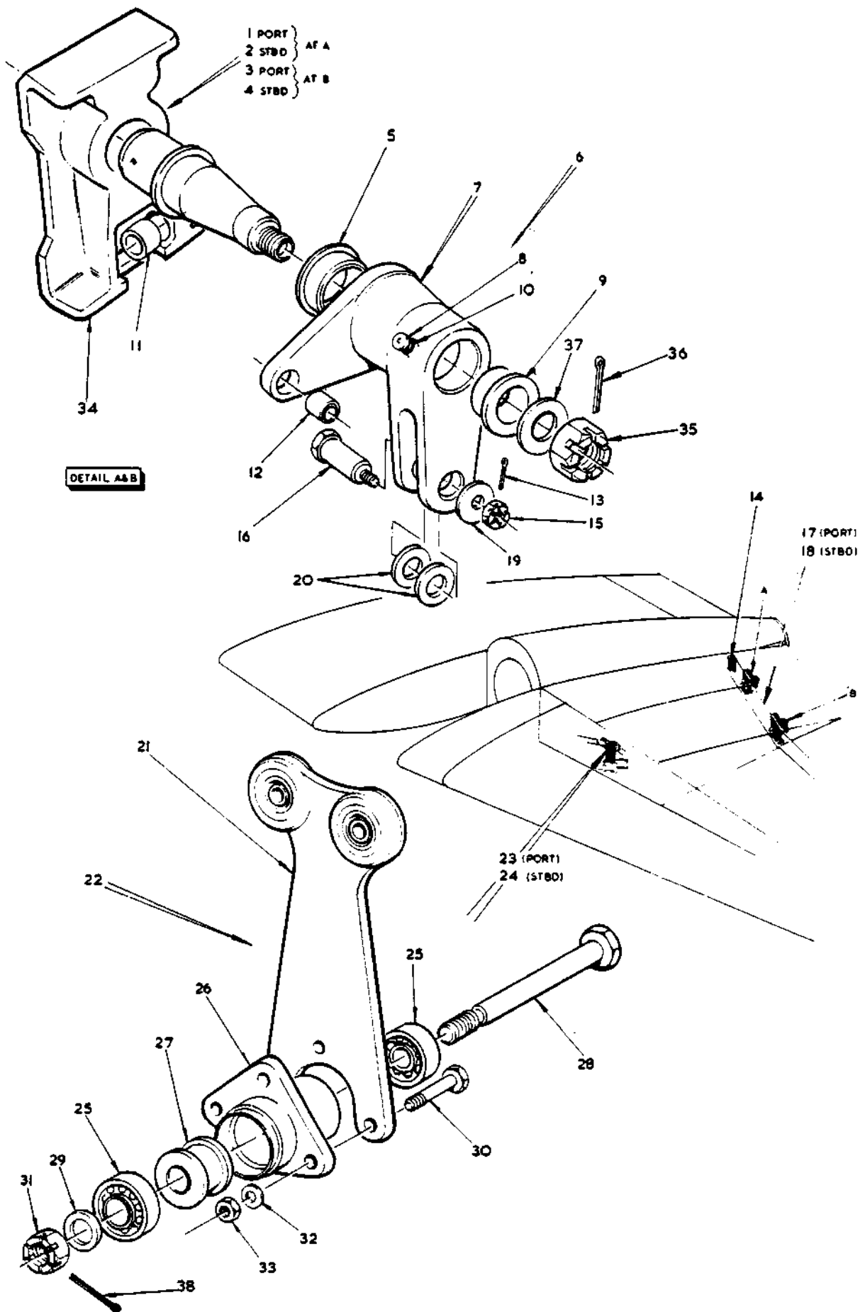
FIG.22 WING STRUCTURE PORT &amp; STBD
