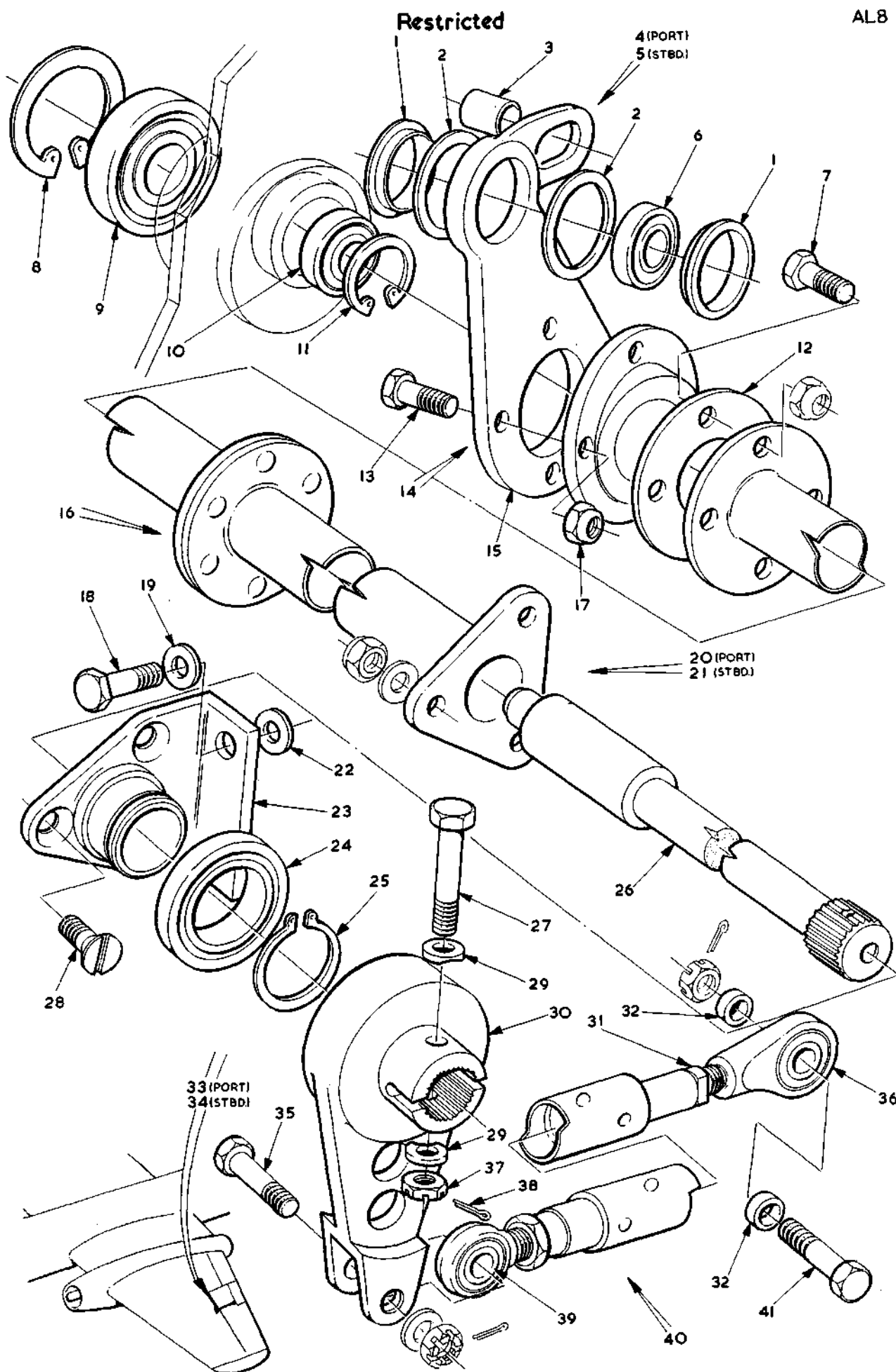
FIG 9. AILERON PORT AND STBD Restricted
