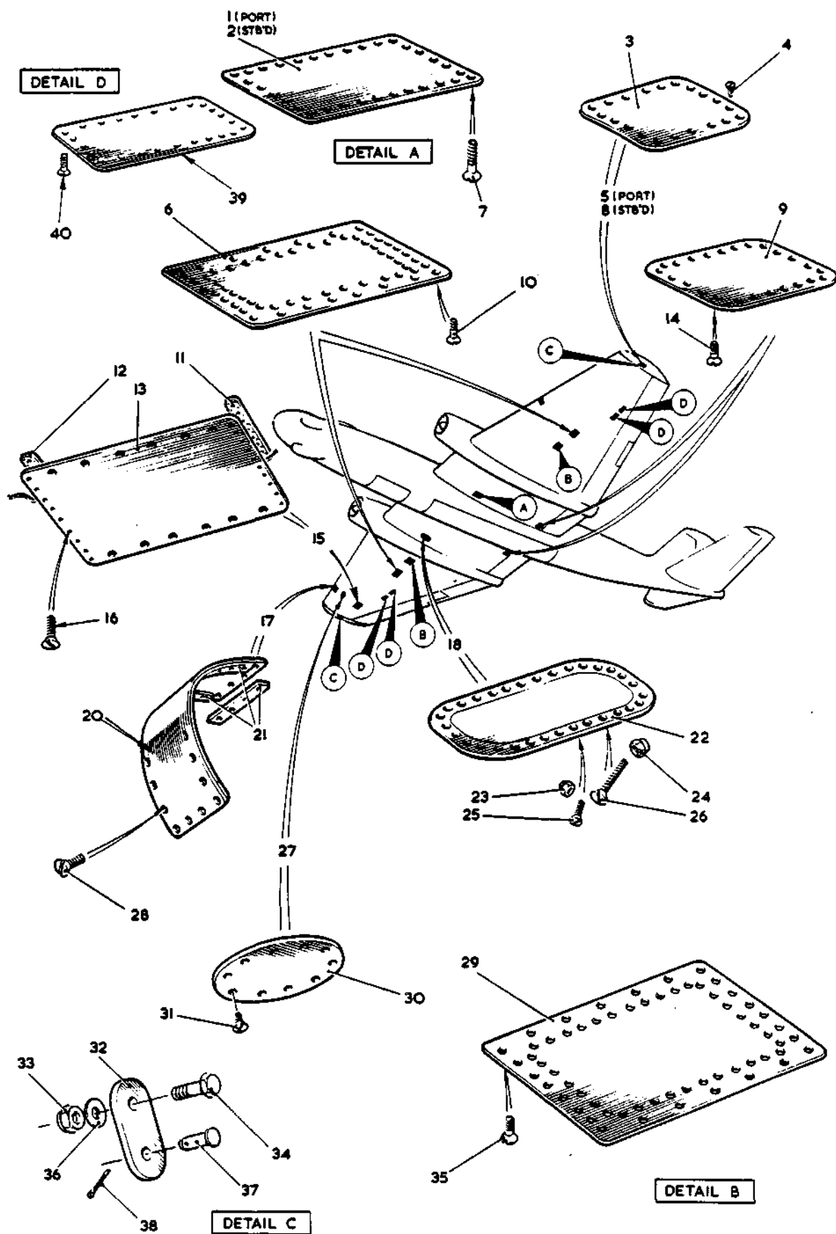
FIG.3 MAIN PLANE PORT &amp; STB'D.
