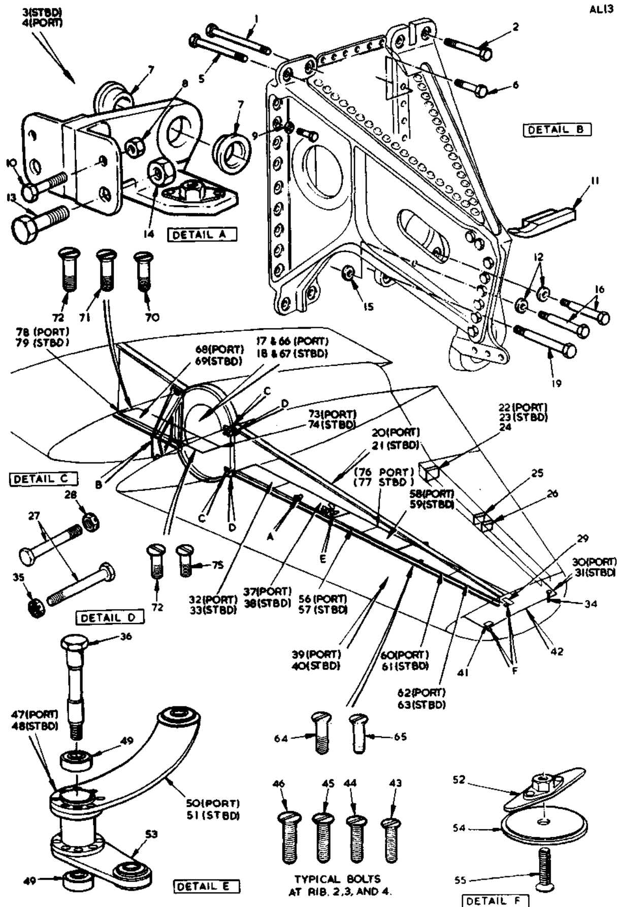
FIG. 14 WING STRUCTURE PORT AND STARBOARD
