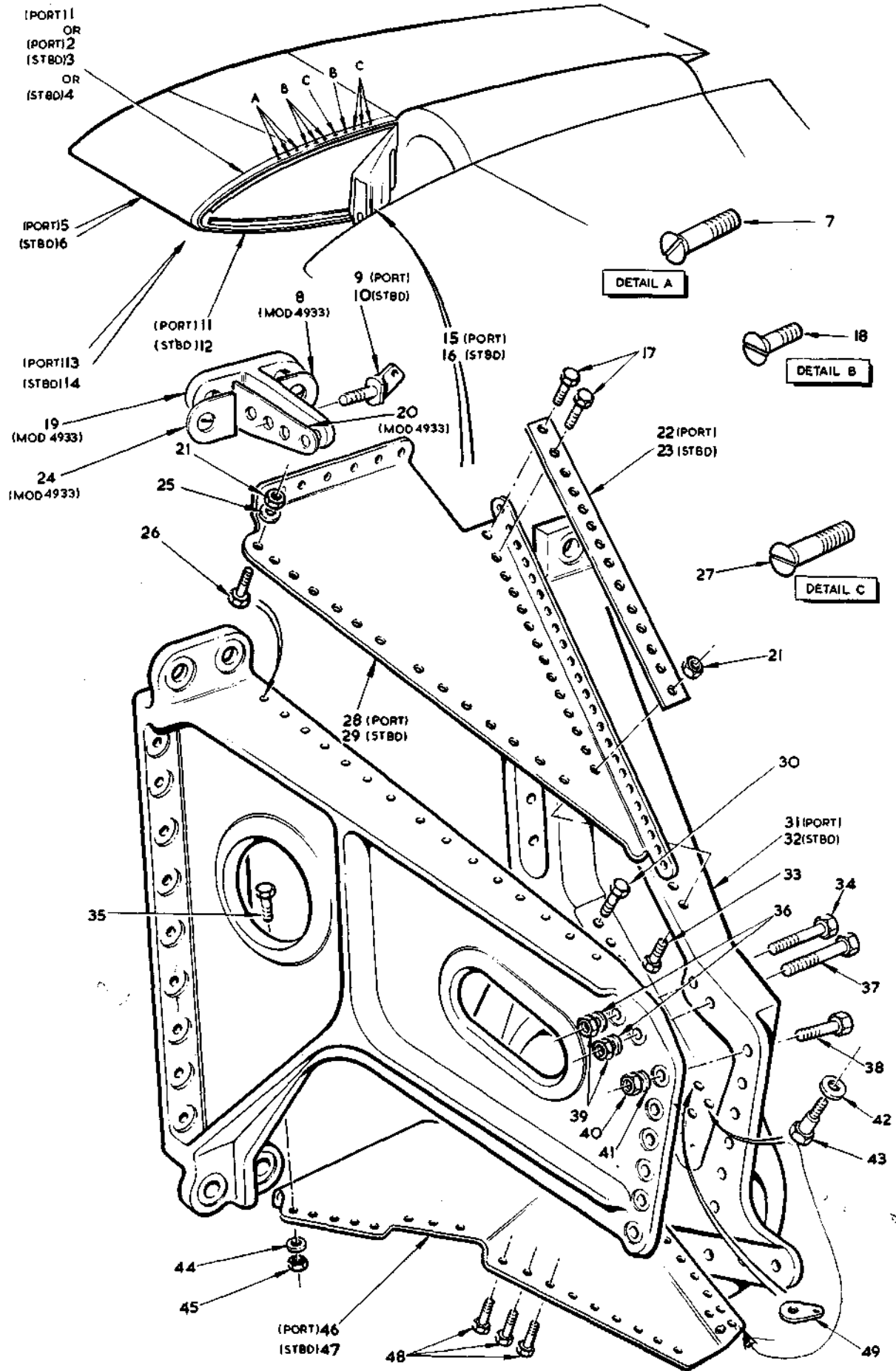
FIG 18 WING STRUCTURE PORT & STBD Restricted
