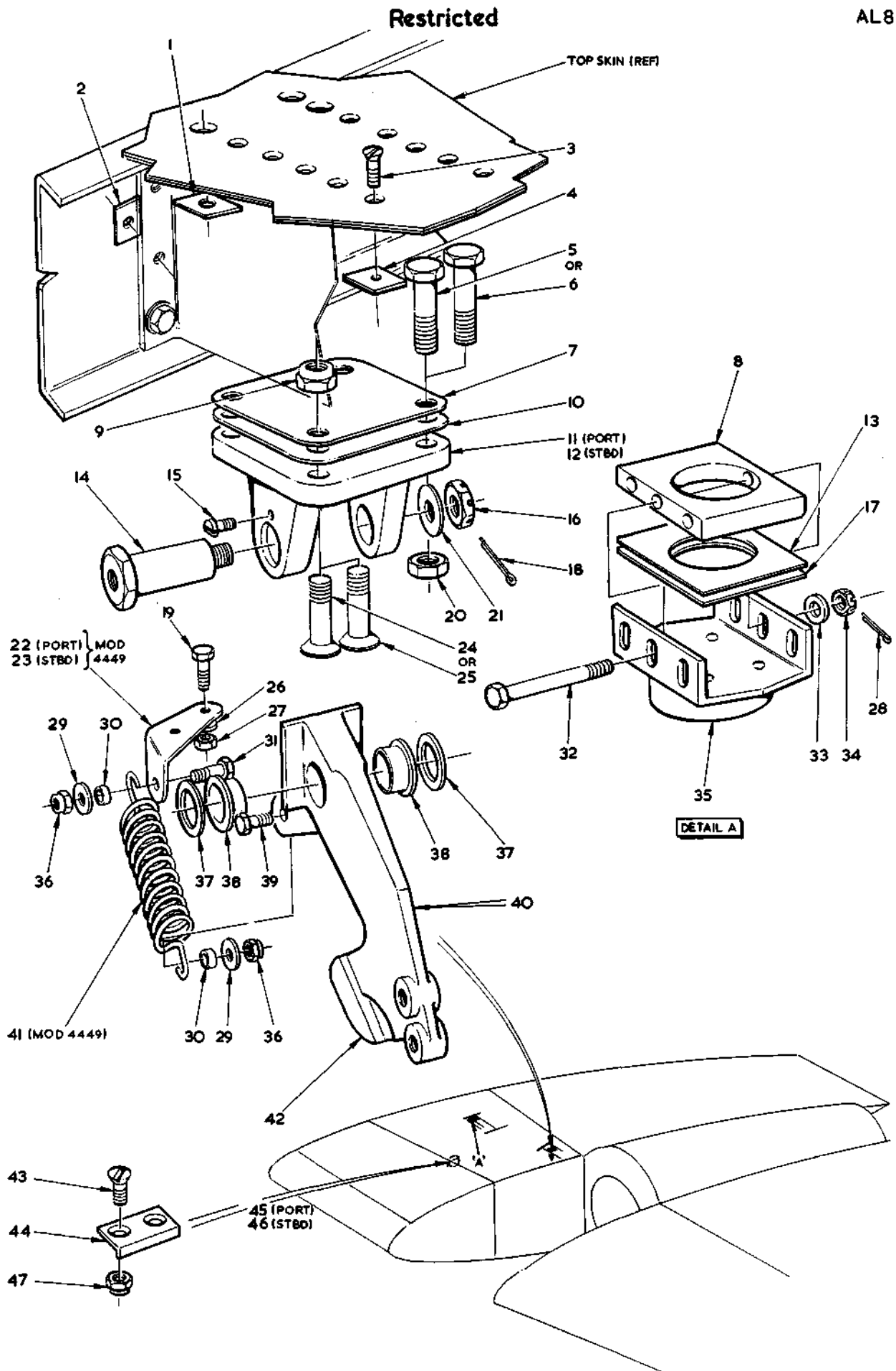
FIG. 17 WING STRUCTURE PORT & STBD. Restricted
