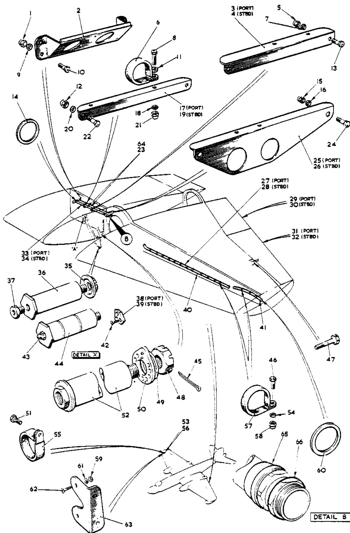
FIG.1 MAIN PLANE PORT &amp; STARBOARD
