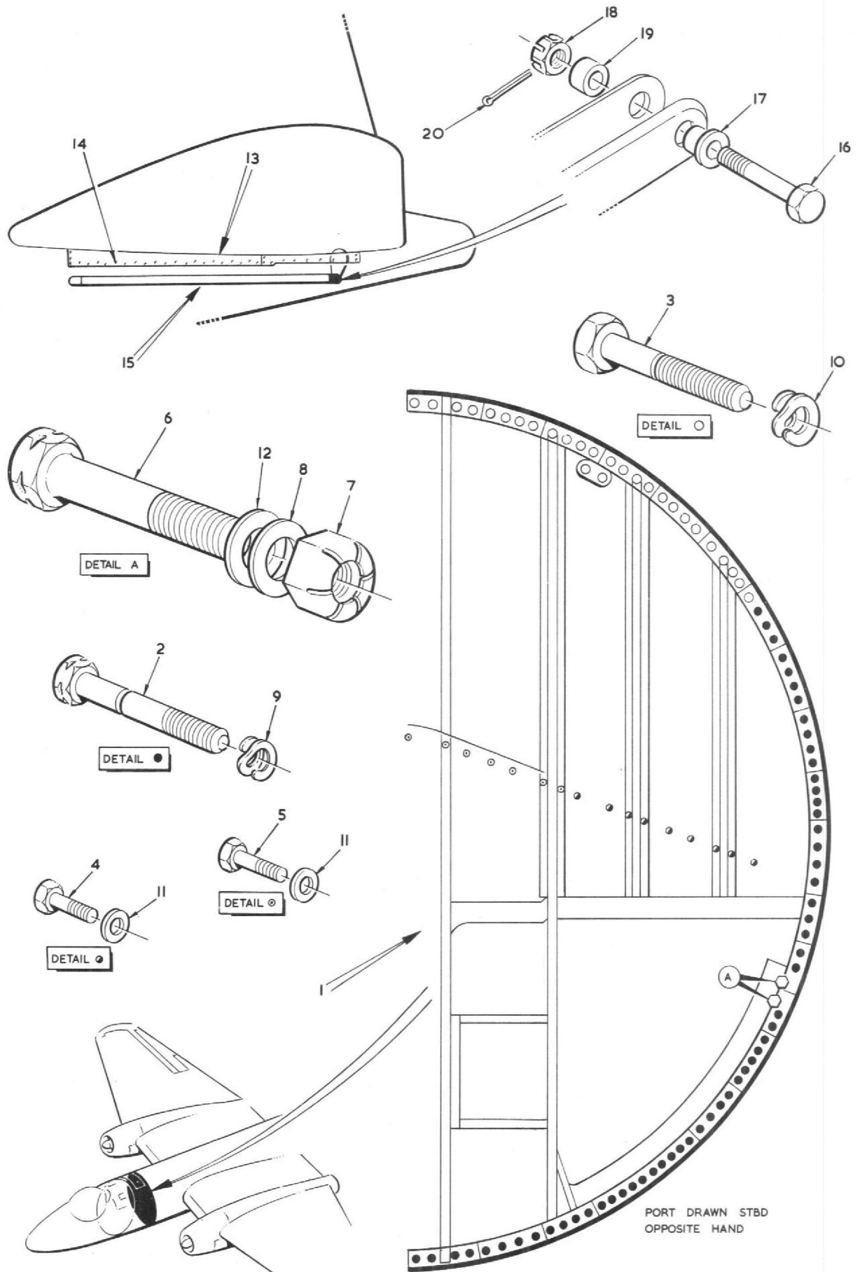
FIG 2 MISCELLANEOUS ATTACHMENT DETAILS Restricted
