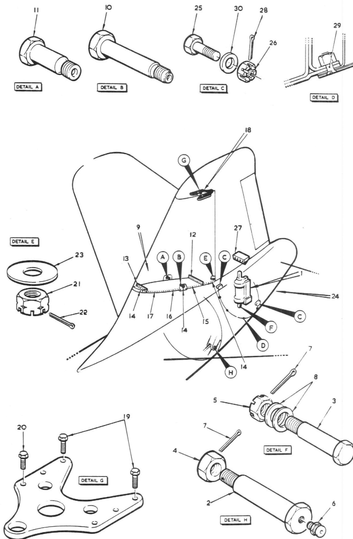
FIG.4 MISCELLANEOUS ATTACHMENT DETAILS
