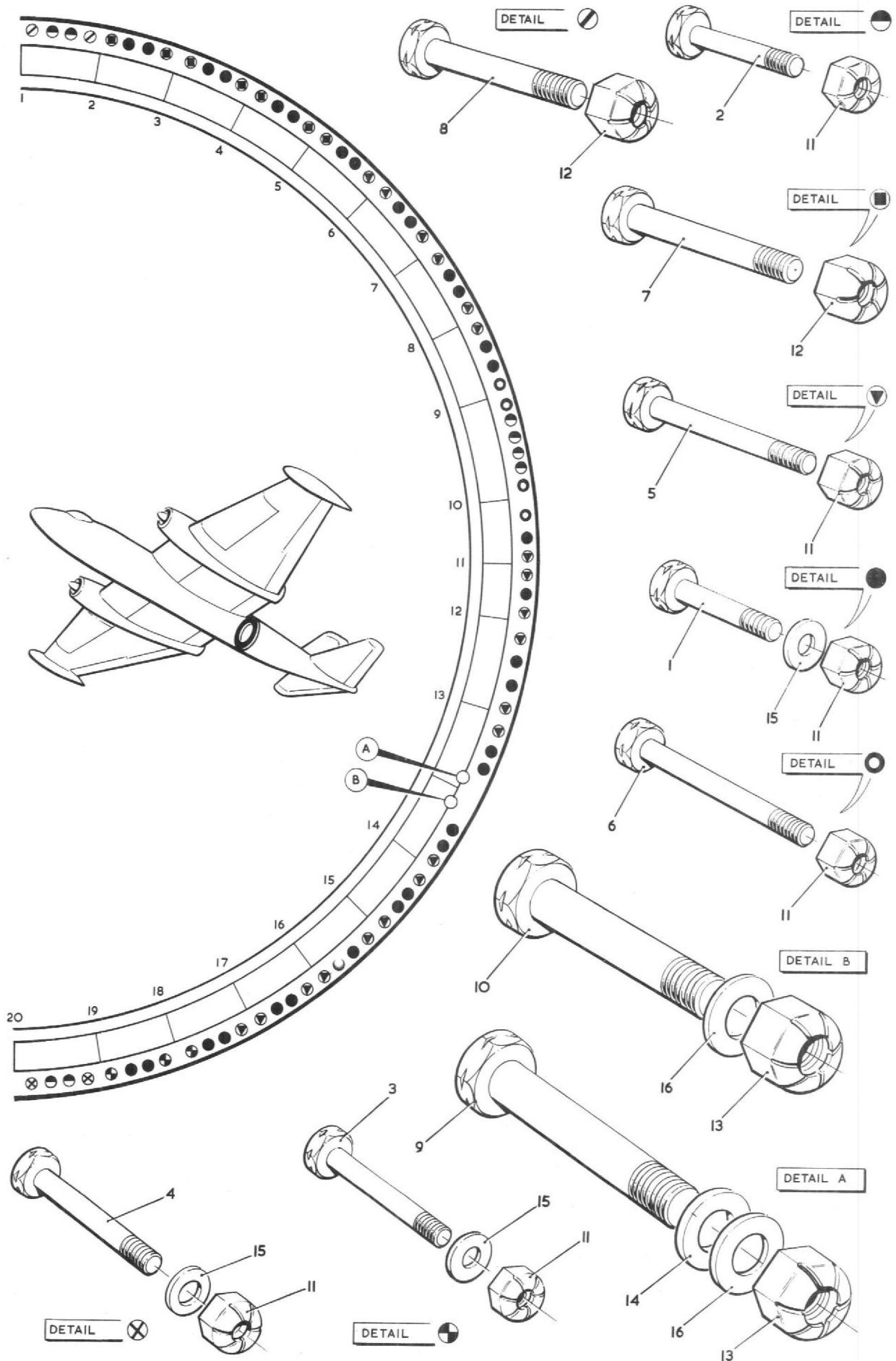
FIG.3 MISCELLANEOUS ATTACHMENT DETAILS Restricted
