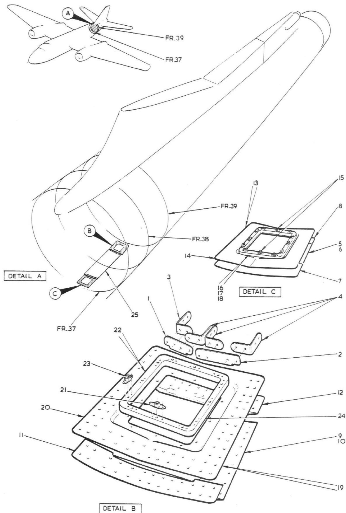
FIG. 5 MISCELLANEOUS ATTACHMENT DETAILS
