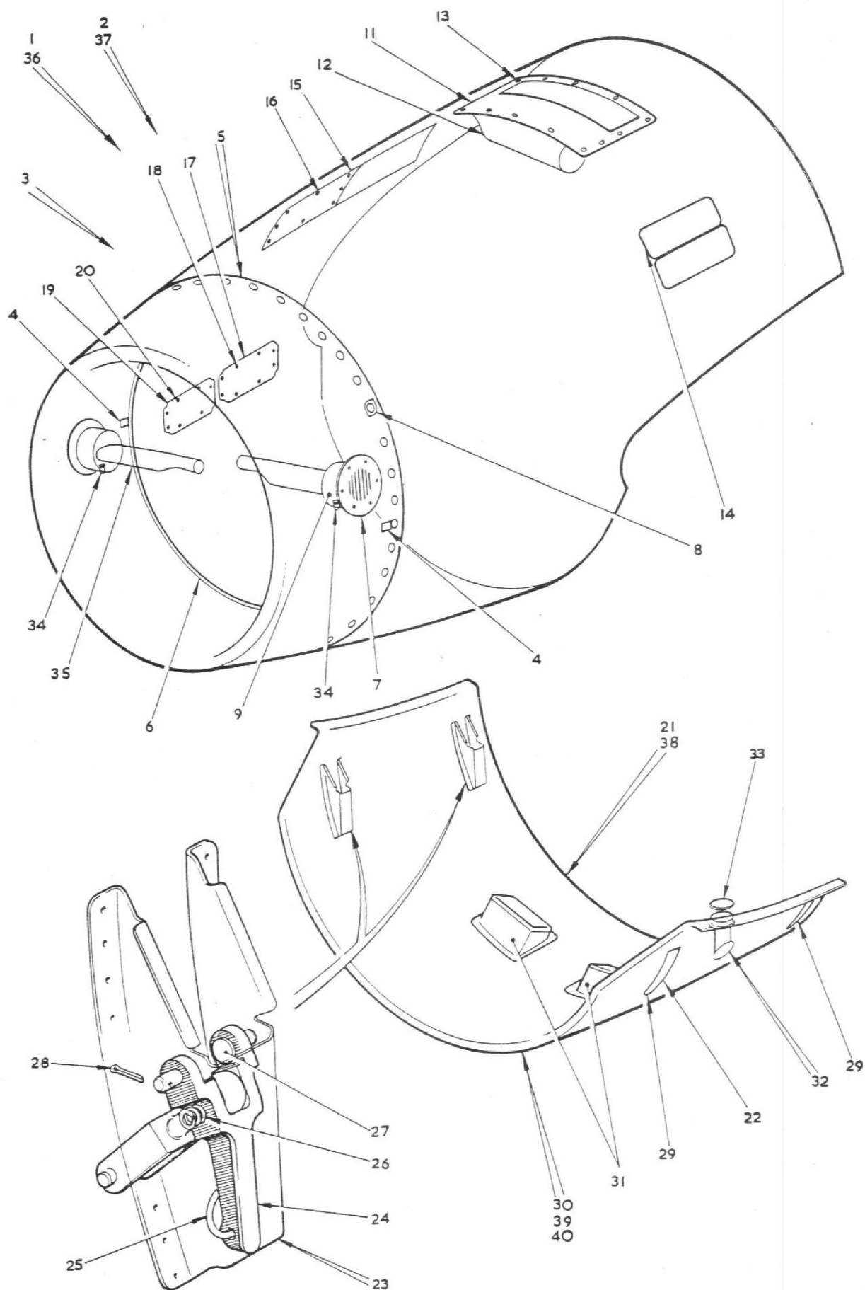
FIG.4 COWLING ENGINE, PORT &amp; STARBOARD
