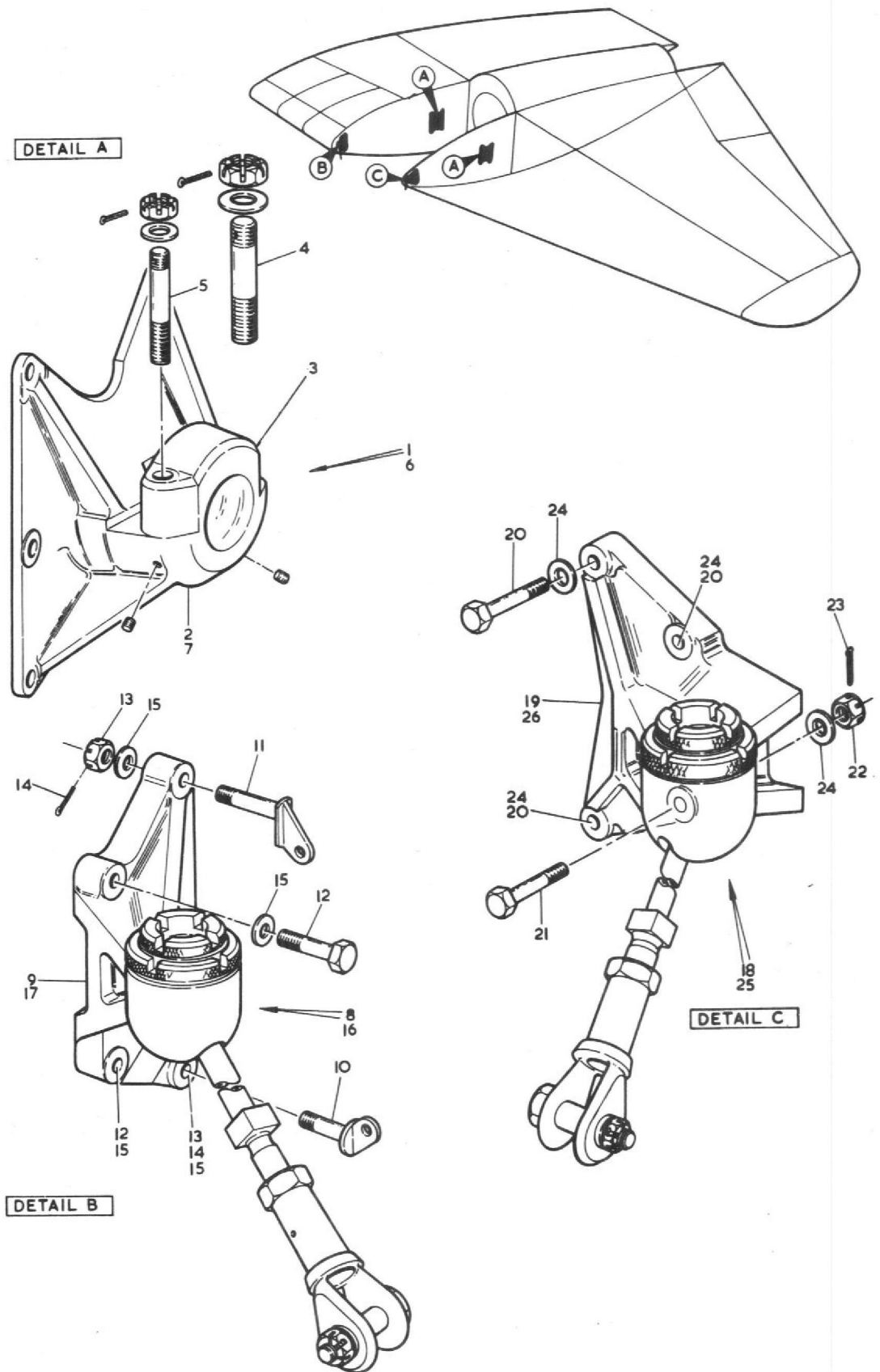
FIG.6A. ENGINE MOUNTINGS AND ATTACHMENTS PORT &amp; STBD.
