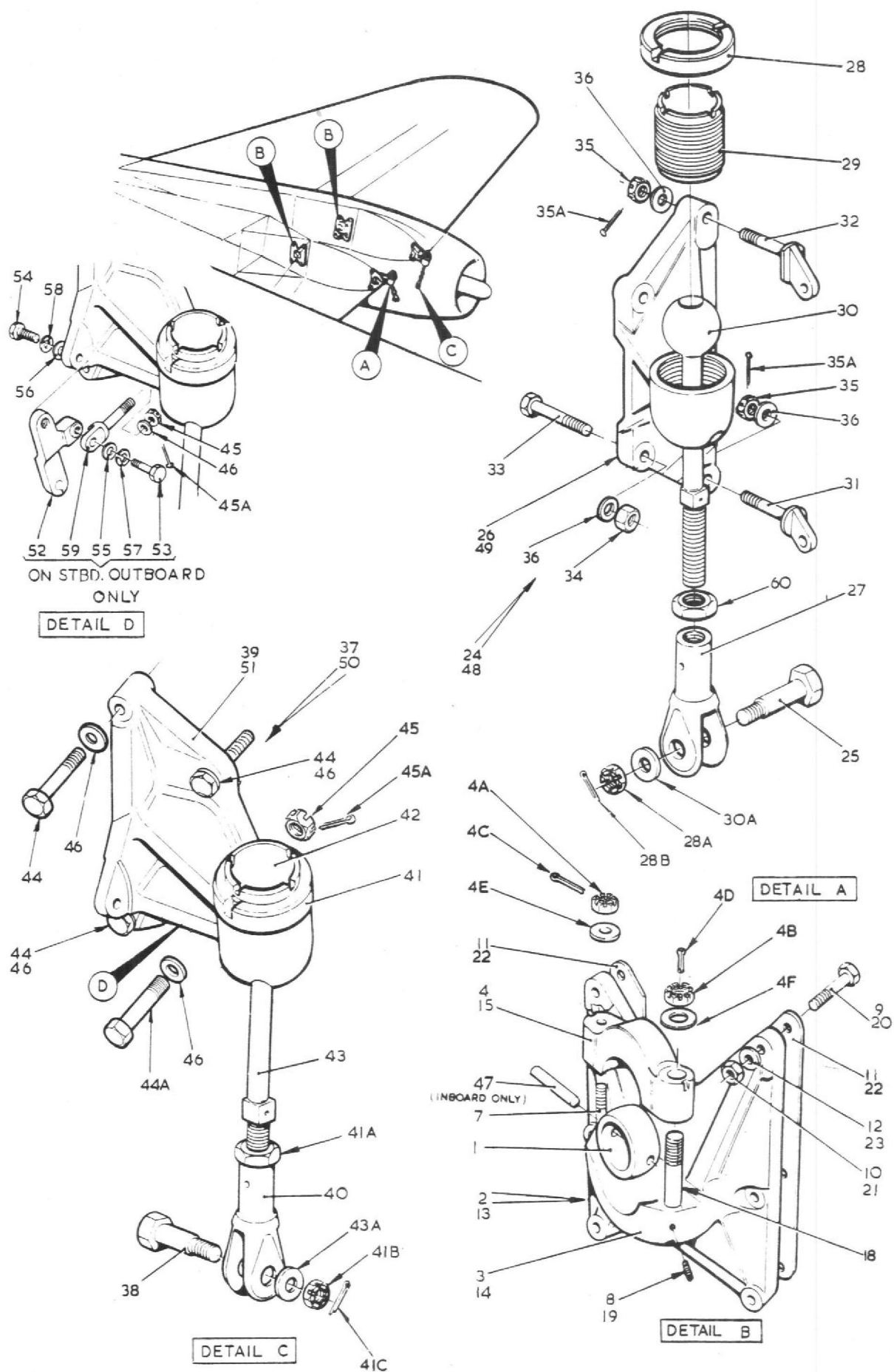
FIG.6 ENGINE MOUNTINGS &amp; ATTACHMENTS, PORT &amp; STBD.
