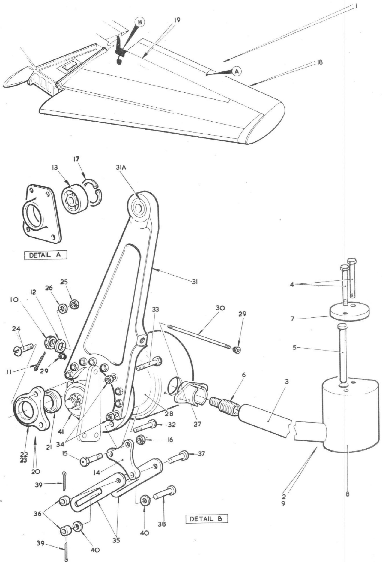
FIG. 4 TAIL UNIT AND ELEVATORS Restricted
