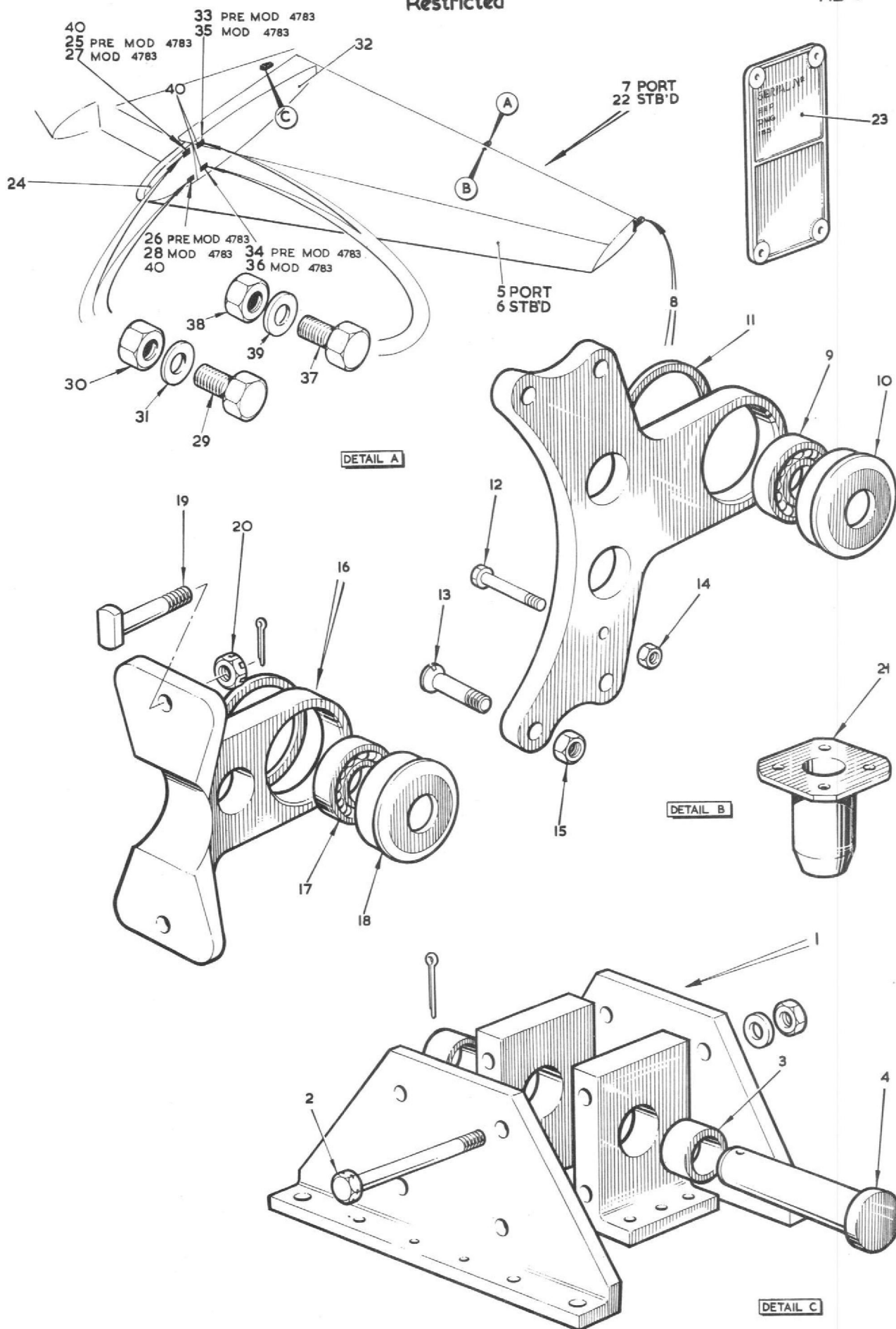
FIG. II TAIL UNIT AND ELEVATORS
