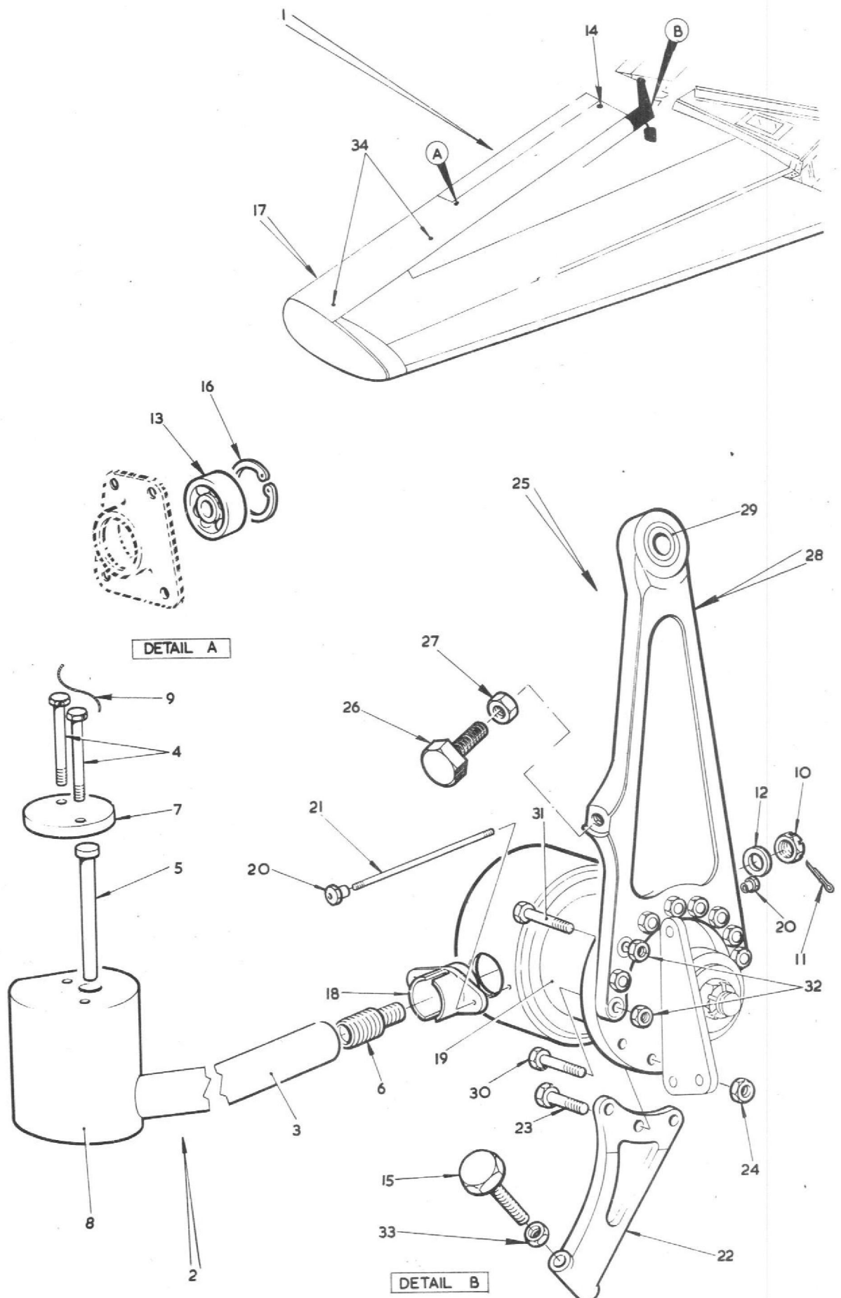
FIG. 5 TAIL UNIT AND ELEVATORS Restricted
