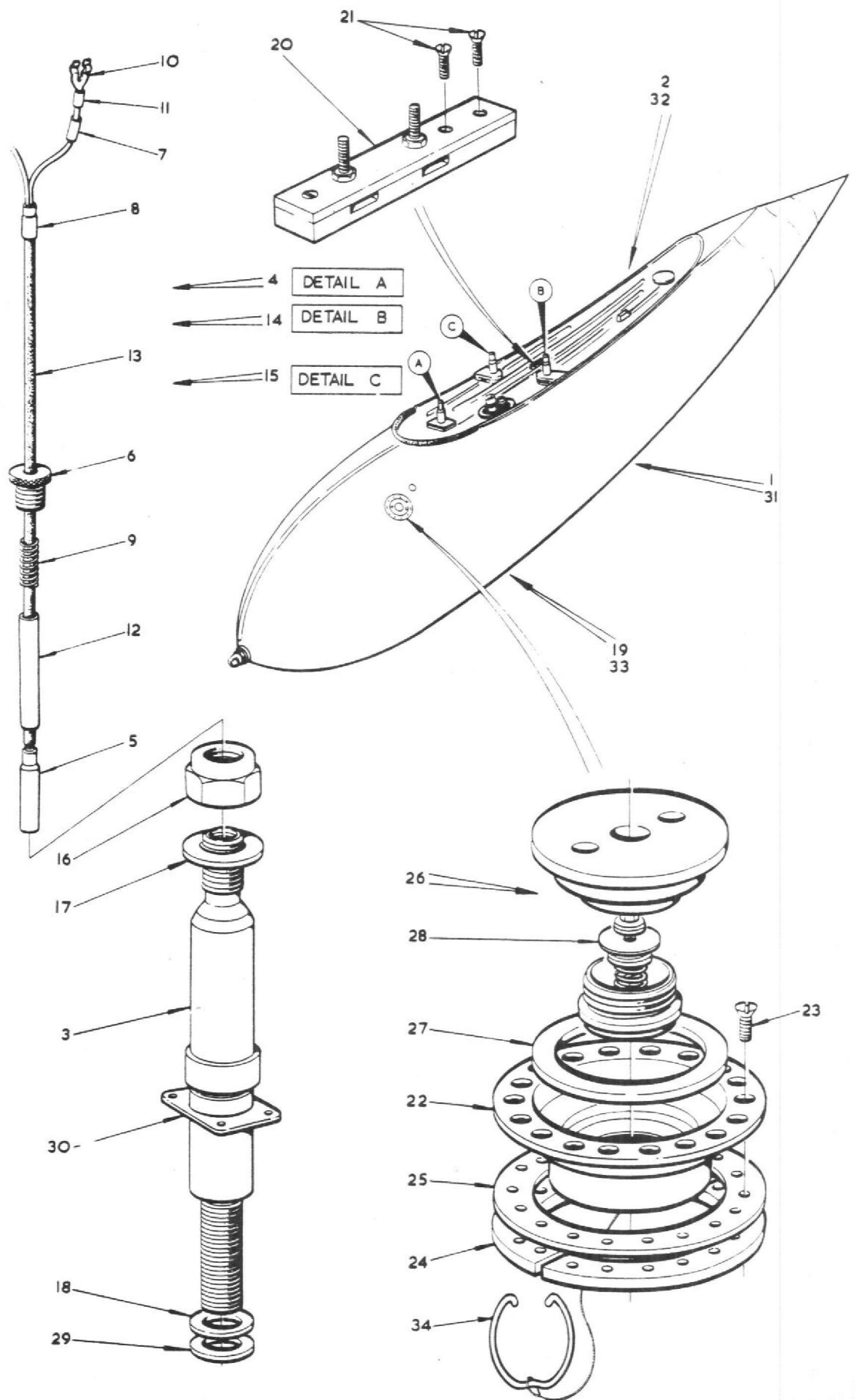
FIG 1 JETTISON WING FUEL TANK PORT &amp; STBD
