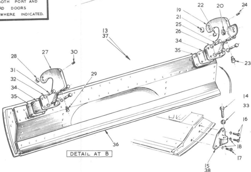
FIG. 4 UNDERCARRIAGE, NOSE UNDERCARRIAGE DOORS Restricted
