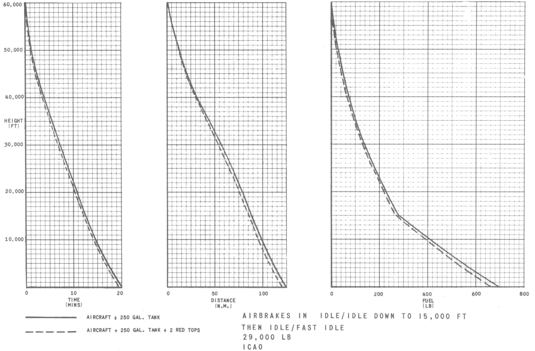
FIG. 6-2. RANGE DESCENT AT 0.9M/250KT.
