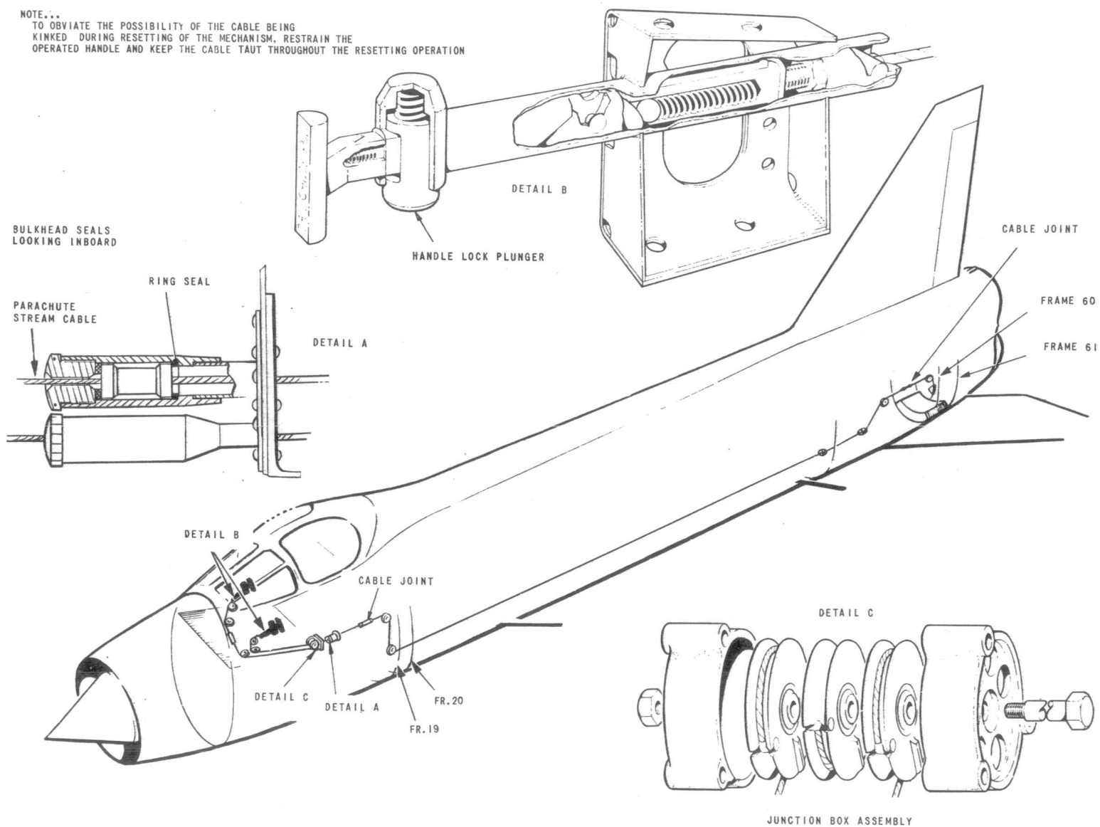
FIG.4. CONTROLS INSTALLATION
