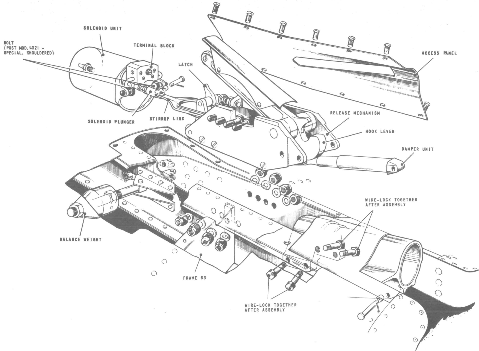
FIG. 7. JETTISONING UNIT—REMOVAL AND INSTALLATION
