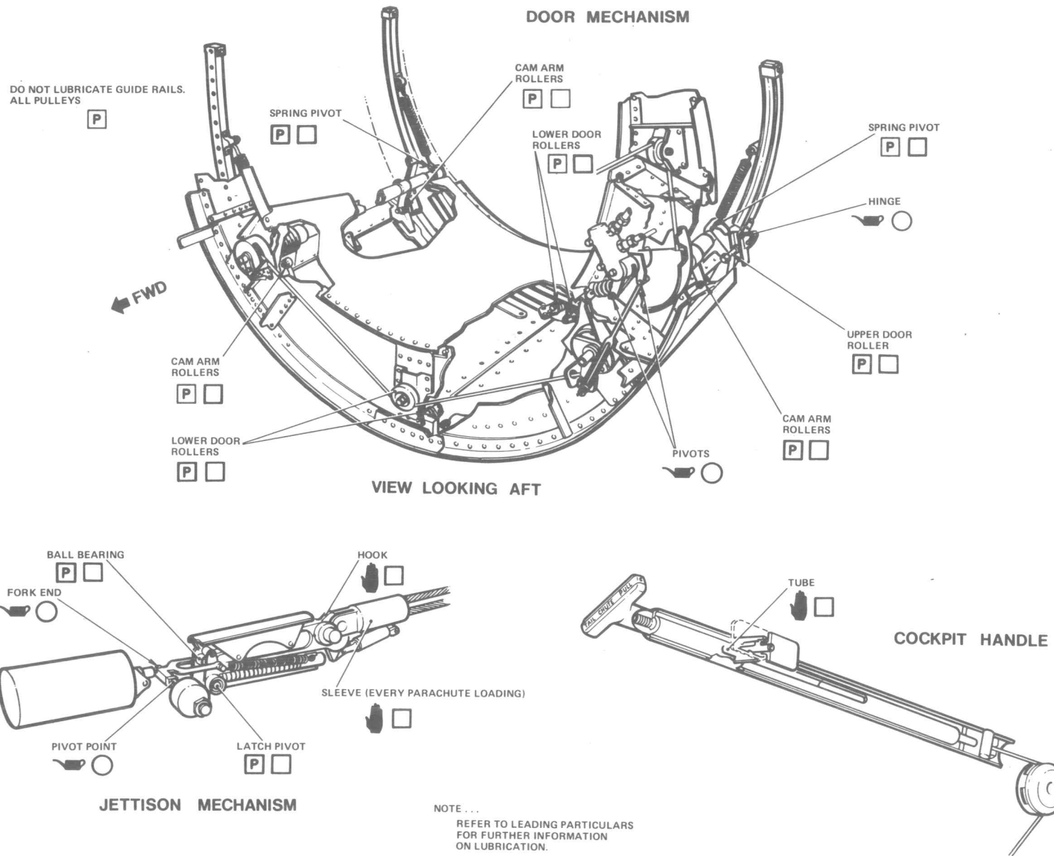
FIG.9. LUBRICATION
