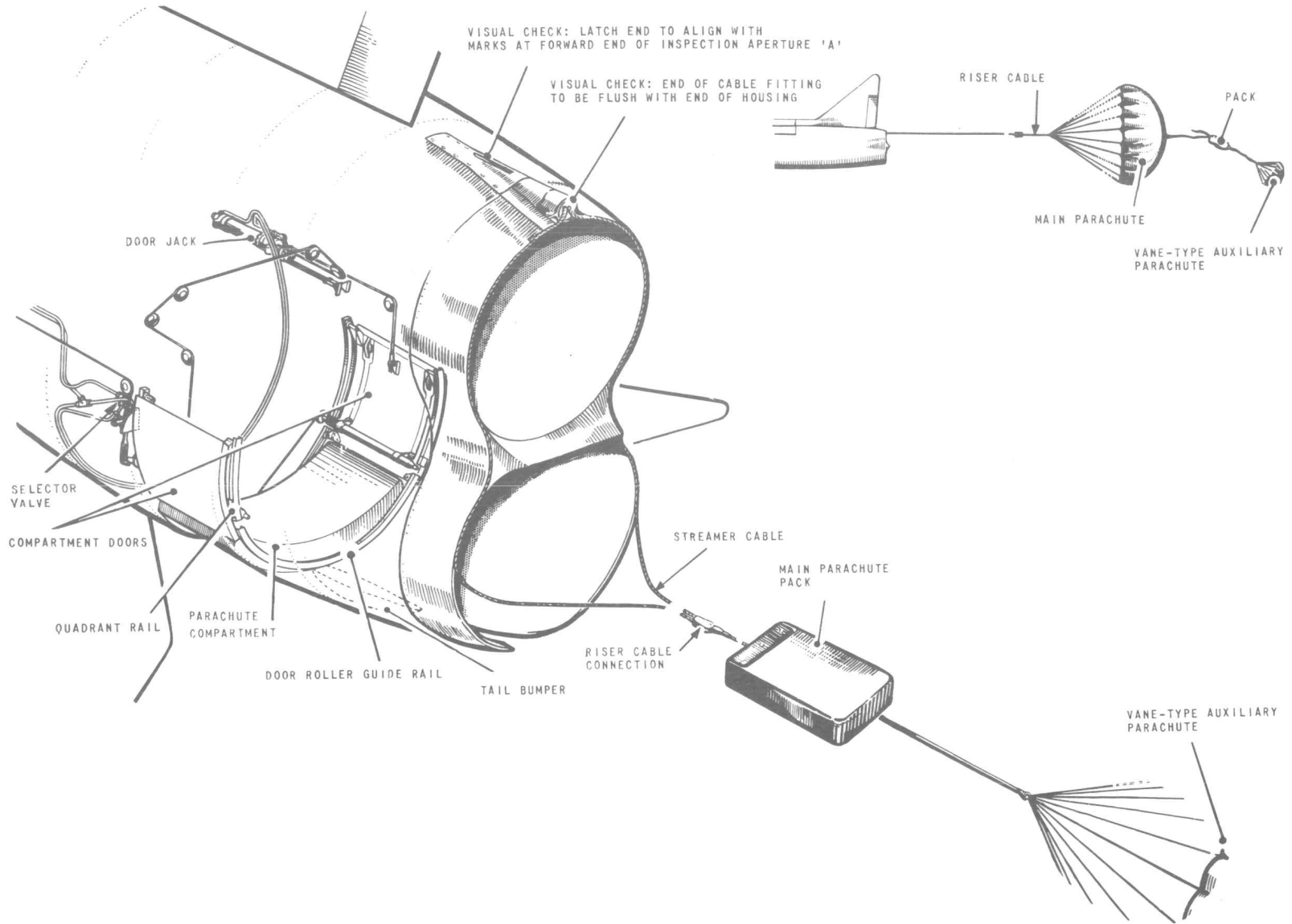
FIG.1. BRAKING PARACHUTE
