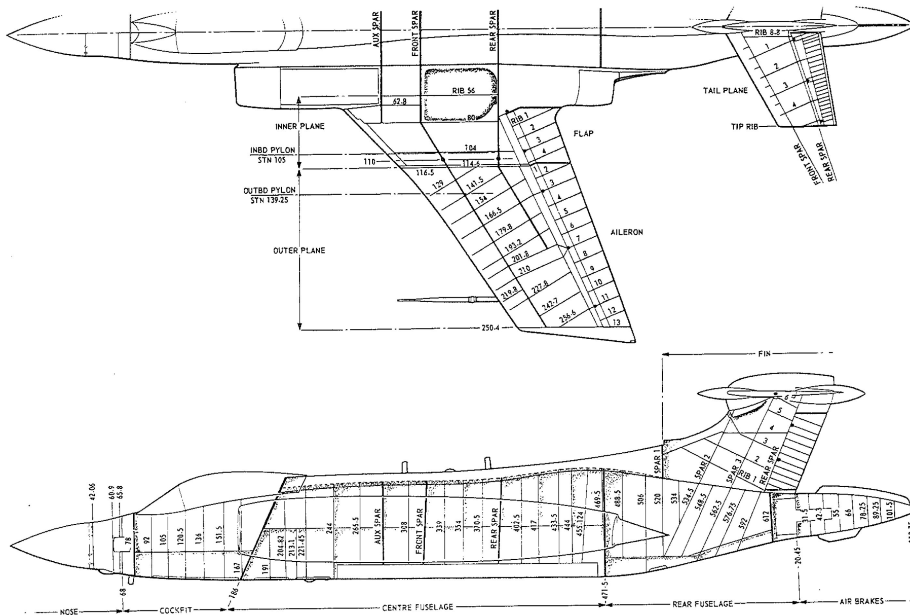
Structural station diagram
