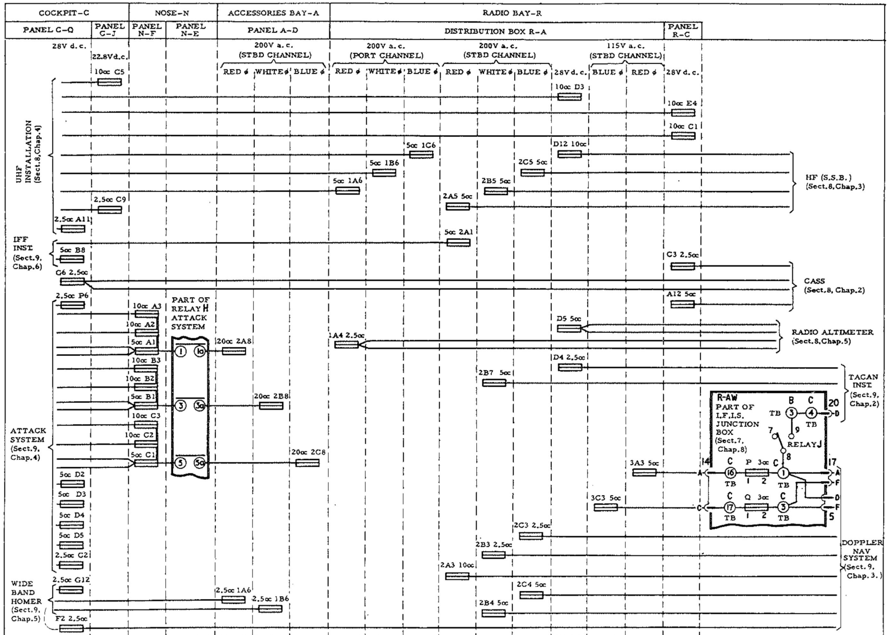
Fig.2. Radio power supplies (pre-Mod 1548)
