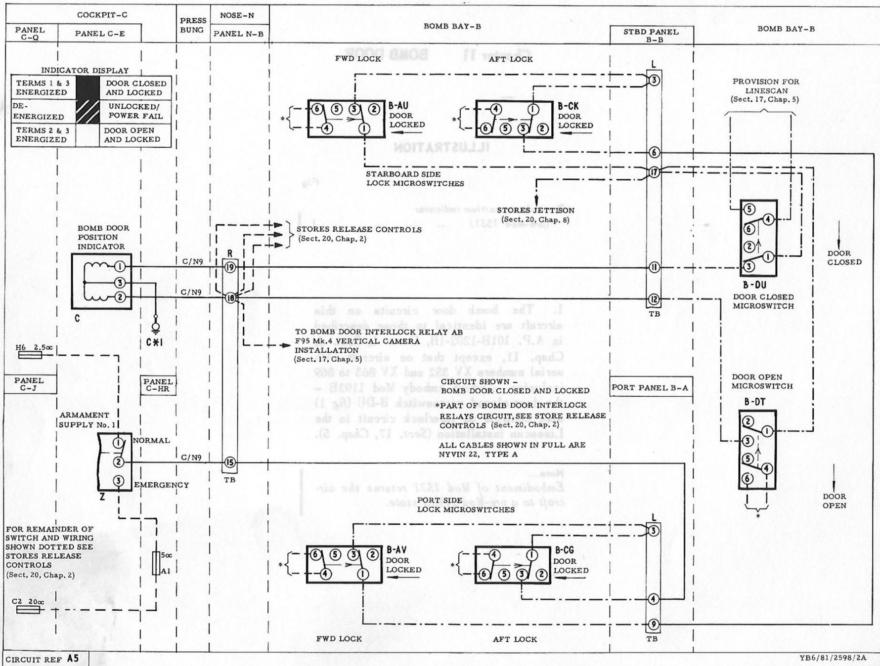
Fig.1. Bomb door position indicator (pre-Mod 1531)
